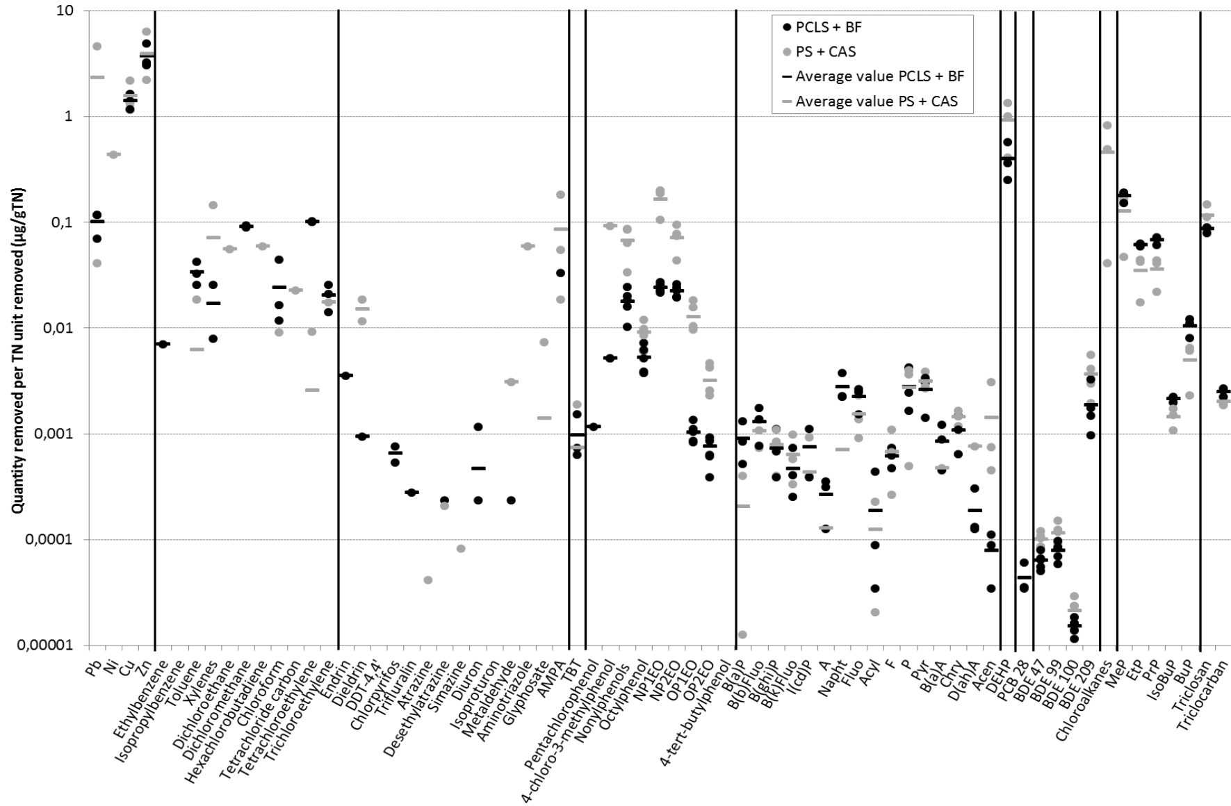
Figure I-17 : Micropolluant removal normalized to nitrogen removal in both WWTPs
