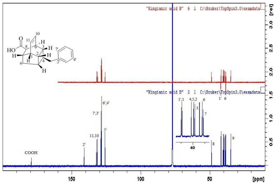
Figure 3.11: ^{13}\text{C} NMR and DEPT-135 spectrum for compound 121
