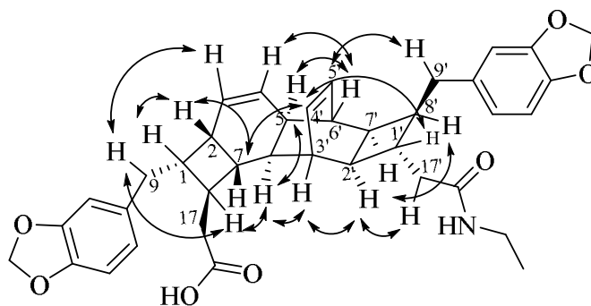
Figure 3.52: Key NOESY ( ^1\text{H} \leftrightarrow ^1\text{H} ) correlations of compound 129
