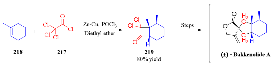
Scheme 5.22: Synthesis of (±) – bakkenolide A
