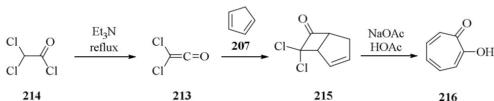
Scheme 5.21: Preparation of tropolone ( 216 )
