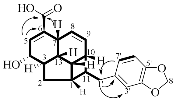
Figure 3.37: Key ^1\text{H} - ^1\text{H} COSY (bold) and HMBC ( ^1\text{H} \rightarrow ^{13}\text{C} ) correlations of 126
