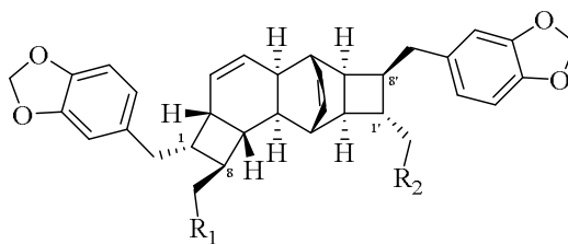
55 : R_1 = \text{CONH}^t , R_2 = \text{CH}_2\text{CH}_2\text{COOH} 56 : R_1 = \text{CH}_2\text{CH}_2\text{COOH} , R_2 = \text{CONH}^t
