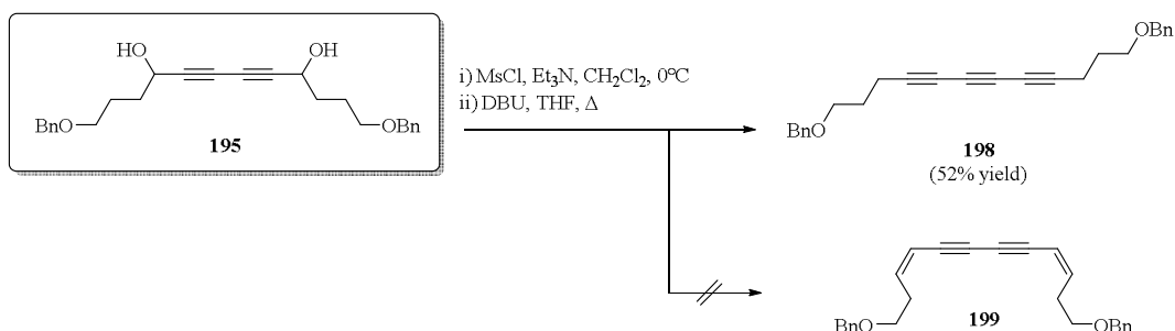
Scheme 5.14: Double dehydration of enyne 195 using mesylate
