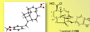
Figure 3. ORTEP plot of tsangibeilin B (10) with the displacement ellipsoids drawn at the 50% probability level
