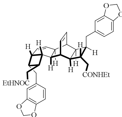
Figure 5.1: Kingianin A ( 45 )
