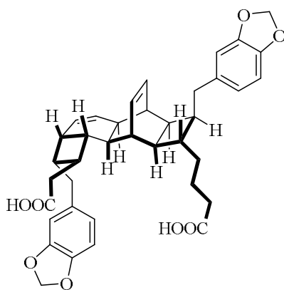
Figure 5.2: Kingianin G ( 51 )
