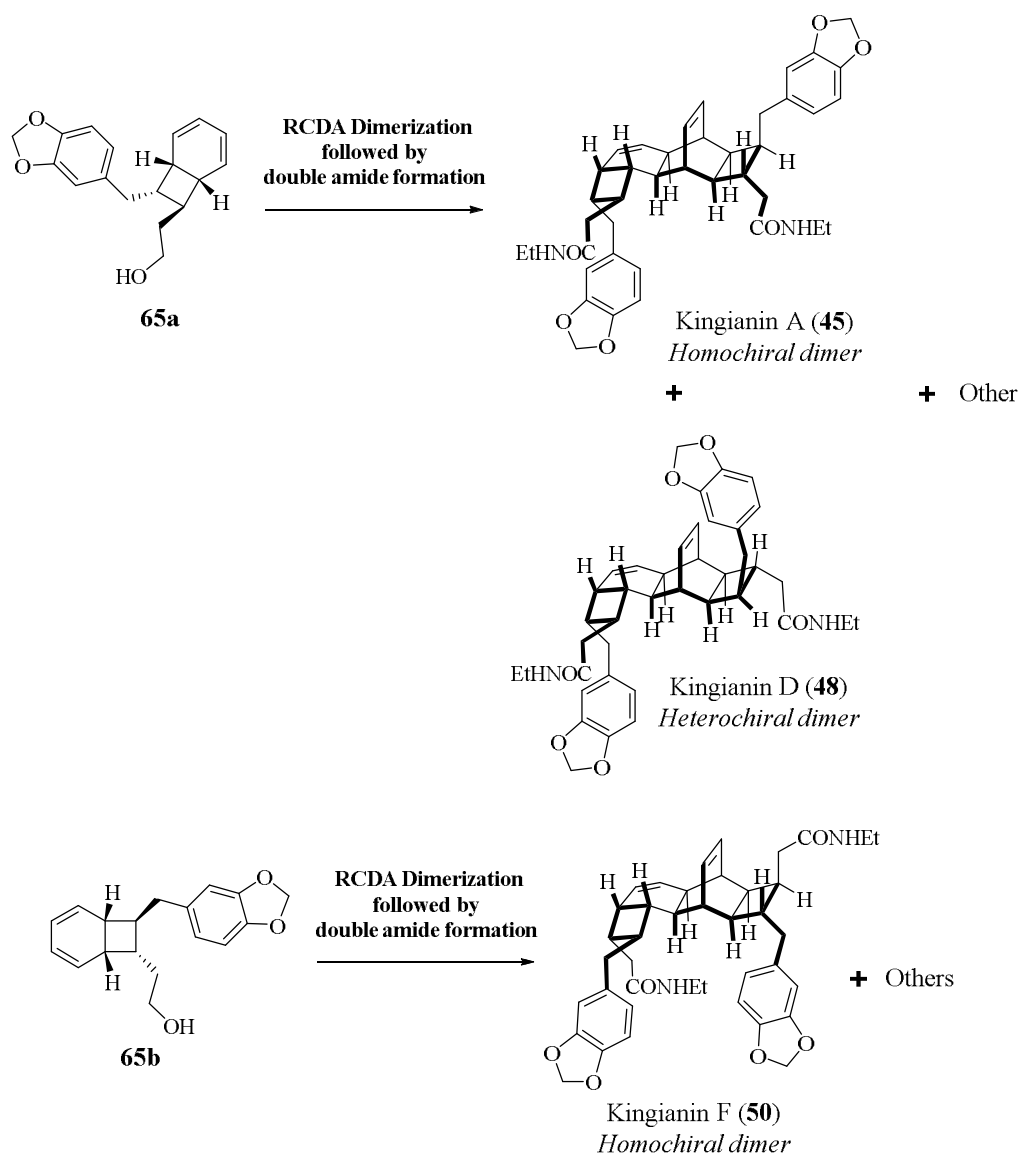
Scheme 2.8: Total synthesis of kingianin A ( 45 ) by Drew et al. (2013)
