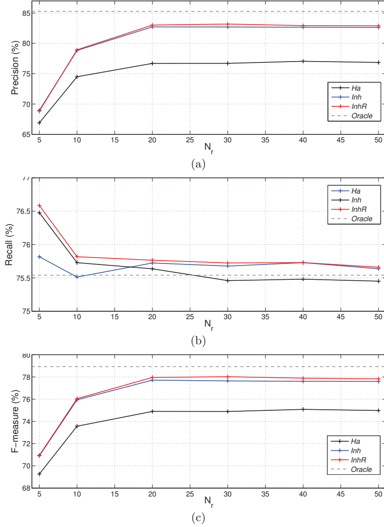
Figure 5.6: (a) Precision, (b) Recall and (c) F-measure (in %) obtained for all methods as a function of the number of partials N_r for T_{on} = -22 dB.
