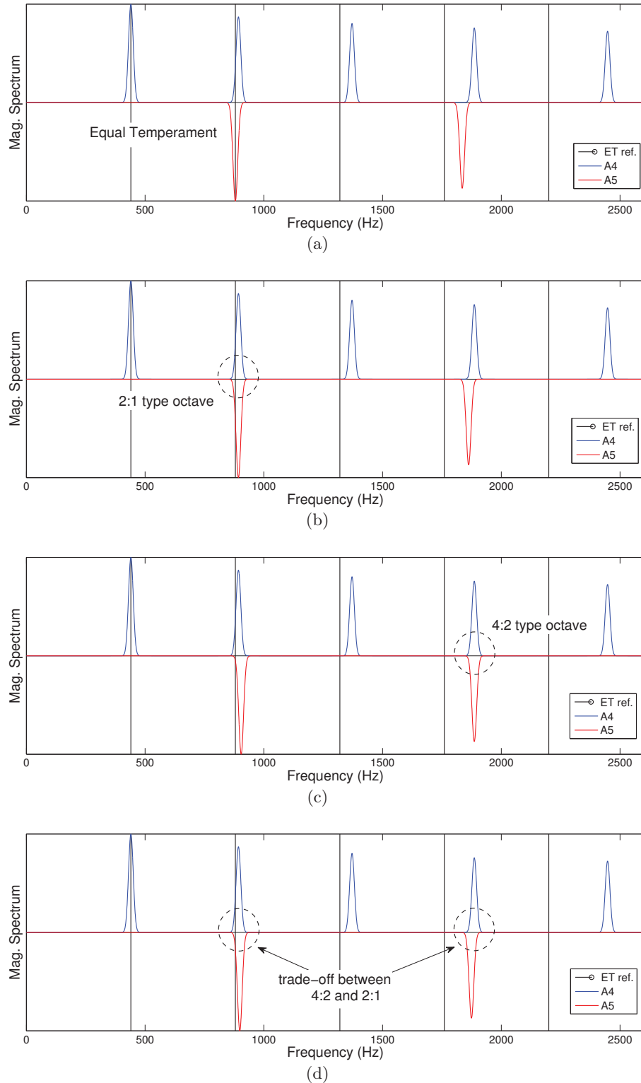
Figure 4.1: Influence of the inharmonicity and the octave type choice on the tuning of the octave A4-A5. Note: the inharmonicity coefficients have been significantly increased from typical values in order to highlight the deviations of the first partial frequencies from the harmonic reference.
