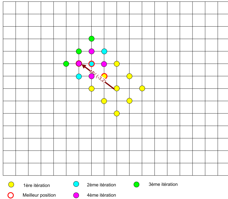
FIGURE 6.9 – Etapes de l'algorithme Diamond Search
