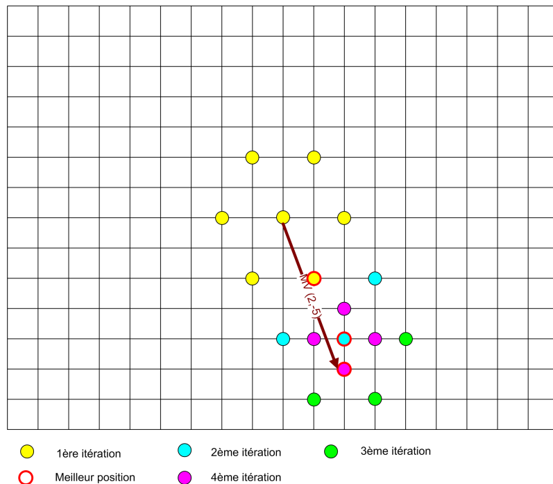
FIGURE 6.10 – Etapes de l'algorithme Hexagone-Based Search
