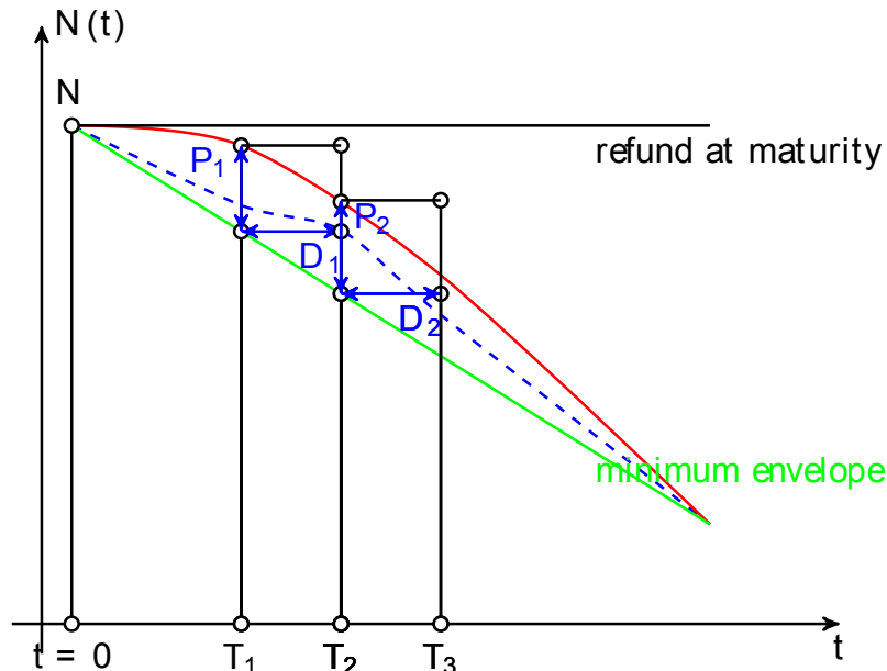
Figure 6.1: Example of schedule for a pool of mortgages. The constant black line is the schedule assuming constant interest, without prepayment and refunding of the full notional at maturity. The concave red curve is the schedule assuming constant annuities and without prepayment. The green straight line represents the minimum of the envelope, i.e. the estimated minimum notional that will remain in the mortgage pool. The envelope is the region between the red and the green curves and it can be approximated by a series of swaptions or caplets. In the figure we have represented two consecutive swaptions/caplets of expiry T_1 and T_2 , maturity D_1 and D_2 , and of notional N_1 and N_2 . The dashed line represents the realized schedule.
