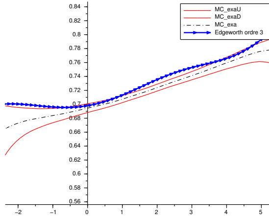
Figure 4.3: Normal implied volatility smile of a 3M \times 5Y caplet using Edgeworth series expansion of the cumulative distribution function of the ZCB P_{T,T+\delta} with T = 5Y and \delta = 3M . We have used the 3 th order expansion. The origin represent the ATM forward libor rate L_t(T, \delta) . The Monte Carlo price is obtained with 10^5 simulation paths and a N = 30 discretization steps. The figures represent different values of the correlation parameter \rho , starting from the left \rho = -0.21_2 , \rho = 0 and \rho = 0.21_2 . The higher order moments of the ZCB are computed using the numerical resolution of the MRDE described in 3.1.4, with a time discretization step of 0.01.
