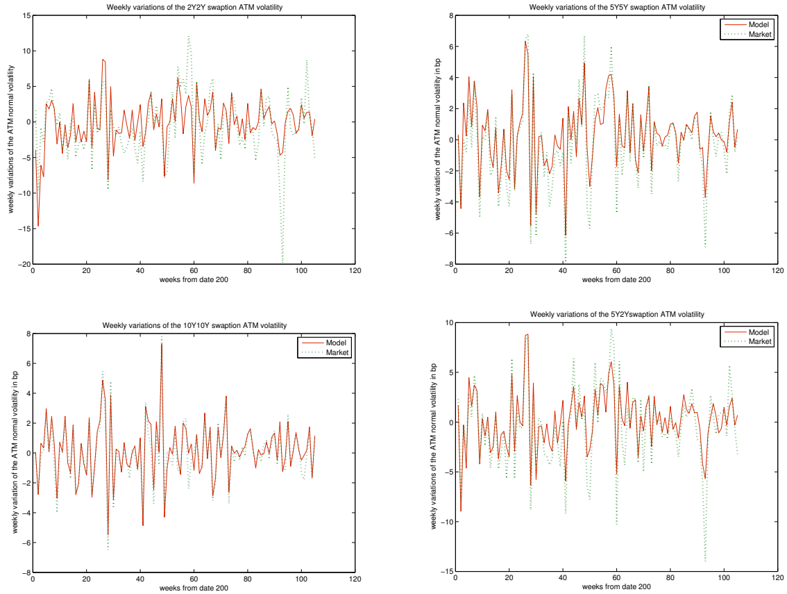
Figure 5.9: Plot of the historic variation of the swaption ATM normal volatility fitted model vs market. We have calibrated x and \Omega at date 200 and calibrated the weekly variations of the volatility surface on successive weeks. We have used a model with 2 curve factors Y and a 4 \times 4 volatility matrix X , with k_1 = 0.01, k_2 = 1, b = \text{diag}(-0.41, -0.01, -0.41, -0.01) and the parameter c is given by (5.4).
