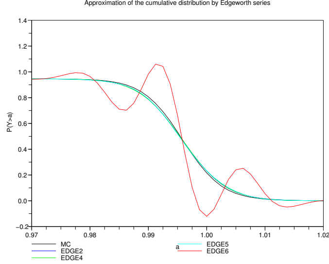
Figure 4.2: Quality of the approximation of Q^T(P_{T,T+\delta} > a) by the Edgeworth series at different orders, with T = 4 and \delta = 3m . The model parameters are x = 10^{-4}I_d , y = (-0.02, 0.01) , \alpha = 2.5 , b = \text{diag}(-0.11, -1.1) , K = \text{diag}(1, 0.1) , c = I_d . The higher order moments of the ZCB are computed using the numerical resolution of the MRDE described in 3.1.4, with a time discretization step of 0.01.
