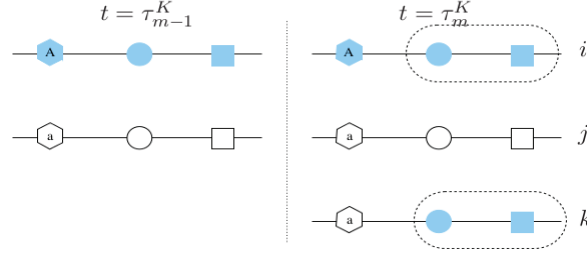
Figure 4.3: Illustration of Definition 5 : the newborn (individual k ) has inherited the selected allele from its "white" parent and the two neutral alleles from its "blue" parent ; hence the encircled neutral loci (of individuals i and k ) coalesce at time \tau_m^K . In terms of recombinations, the two neutral loci of the newborn individual recombine at time \tau_m^K from the a - to the A -population
