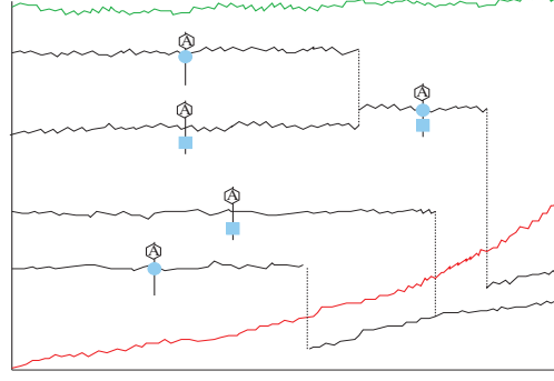
Figure 4.4: Illustration of events [2, 1]_{A,i}^{rec} (individual 1) and [12, 2]_{A,i}^{rec} (individual 2)
