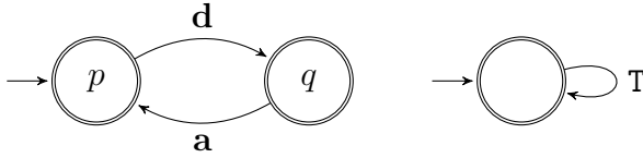
Figure 8.2: An automaton for (\mathbf{da})^*(\varepsilon + \mathbf{d}) and its S-T encoding of type \mathbf{d}
