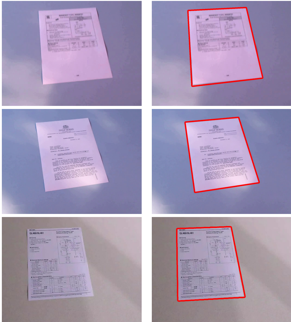
Figure 62: ICDAR competition on document detection. These images show the robustness of our method to blur and light specularity that move object boundaries. Note that some videos are available as supplementary materials [24].
