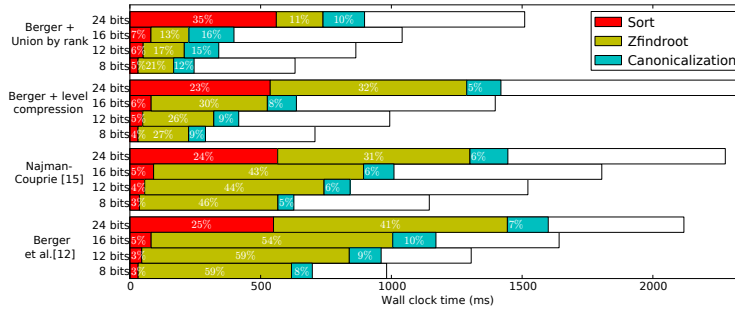
Figure 71: Time distribution of the sequential union-find-based algorithms.
