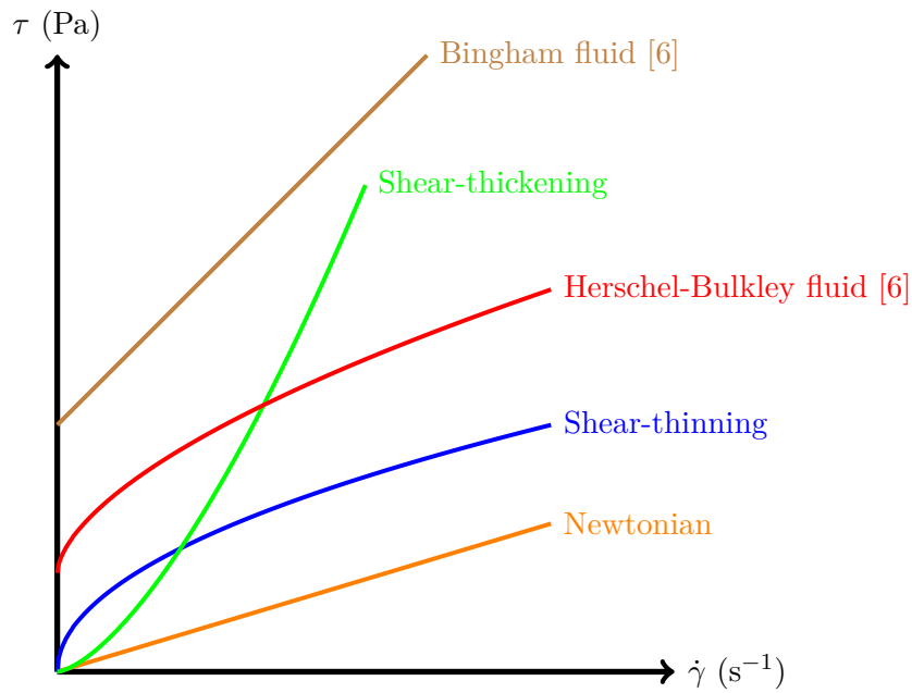
Figure 1.6 – \tau = f(\dot{\gamma}) for the most common behavior of materials
