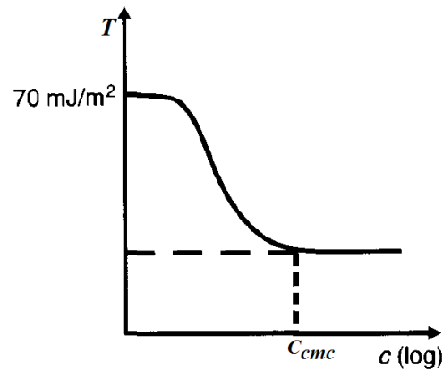
Figure 1.5 – Typical variation of surface tension T as function of the surfactant concentration, adapted from [56].
