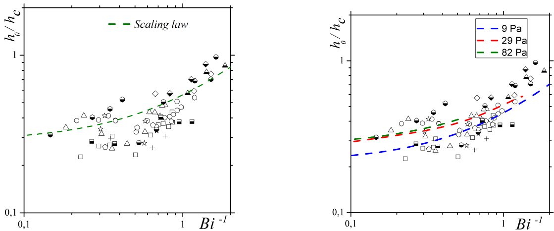
(a) Scaling for the gravitational regime ( \beta = 0 , \alpha = 0.28 ). (b) Scaling for the cross-over of the capillary and gravitational regime ( \beta = 0.1 , \alpha = 0.28 ).
