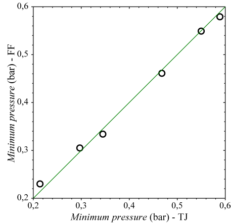
Figure 5.3 – Comparison of minimum bubbling pressure for T-junction (TJ) and flow focusing (FF) device with R=1 mm, L=10 cm, for carbopol ( \tau_y = 75 Pa). The plain line indicates y = x . The flow rate values are: 0.01, 0.05, 0.1, 0.5, 1, 1.5 ml/min.
