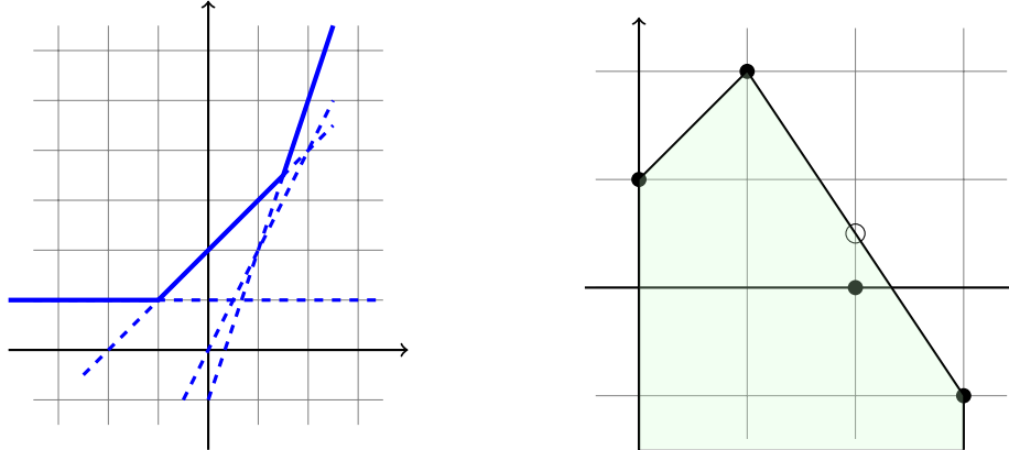
Graph of p = -1X^3 \oplus X^2 \oplus 2X \oplus 1 . Note that the line with slope 2 does not appear in the convex hull.
