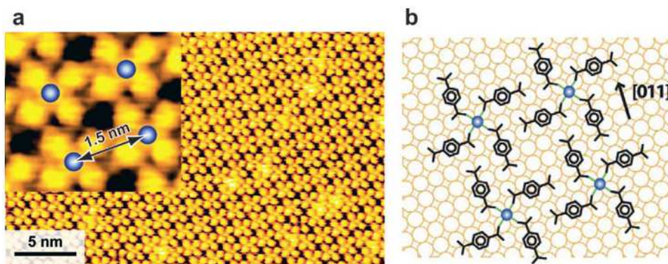
Figure 1.4: (a) High-resolution STM image of the "Clover-leaf" phase, with Fe atoms marked. (b) Geometrical model: each Fe atom (blue spheres) coordinates four 1,4-benzenedicarboxylic acid ligands (TPA molecules), in a square-planar configuration [19].
