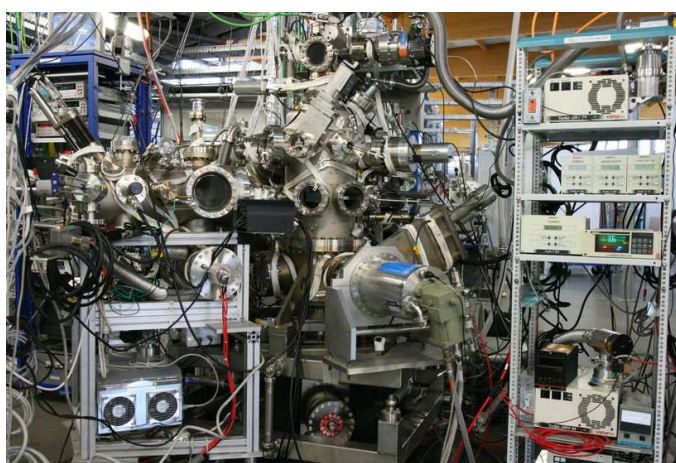
Figure 2.22: The UHV chambers of the TEMPO beamline.
