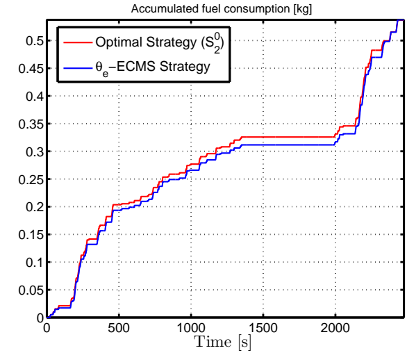
Figure B.15: Accumulated fuel consumption [kg]
