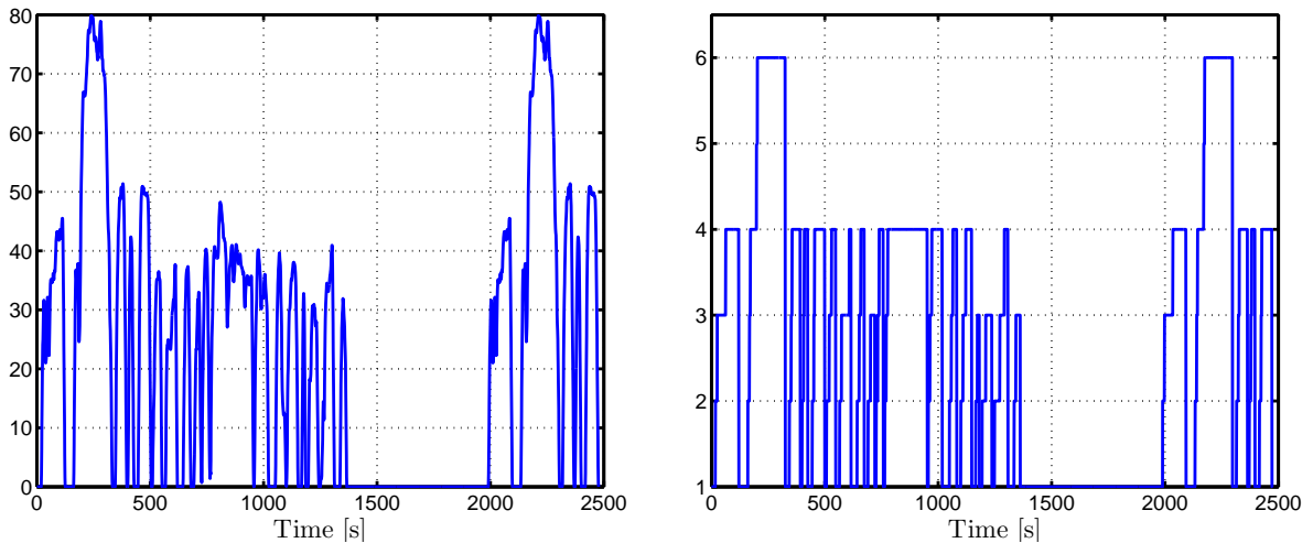
Figure A.1: Wheel speed [km/h] (left) and gear-box ratio (right) for FTP-75 cycle
