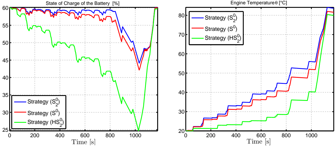
Figure B.7: SOC [%] (left) and engine temperature \theta_e [°C] (right) trajectories for NEDC
