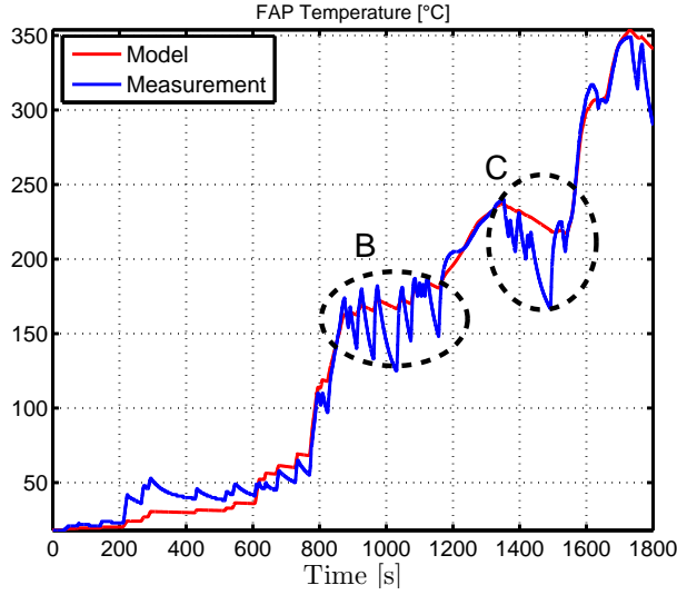
Figure 7.19: Temperature \theta_{dpf} [°C] for Vc 1 -Test
