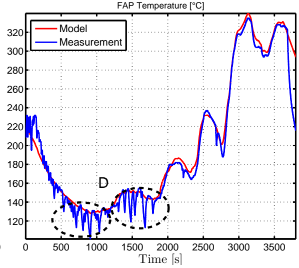
Figure 7.20: Temperature \theta_{dpf} [°C] for Vc 2 -Test
