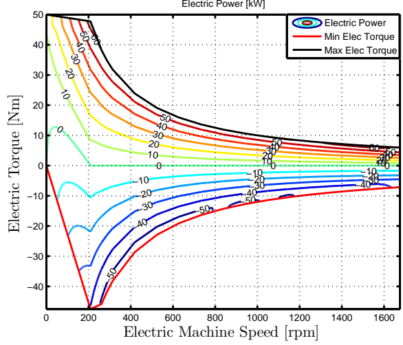
Figure 7.7: Electric power map P_m [kW]
