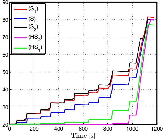
Figure 4.6: Histories of simulated engine temperature \theta_e [°C] obtained from optimal input calculated for \alpha = 0.8
