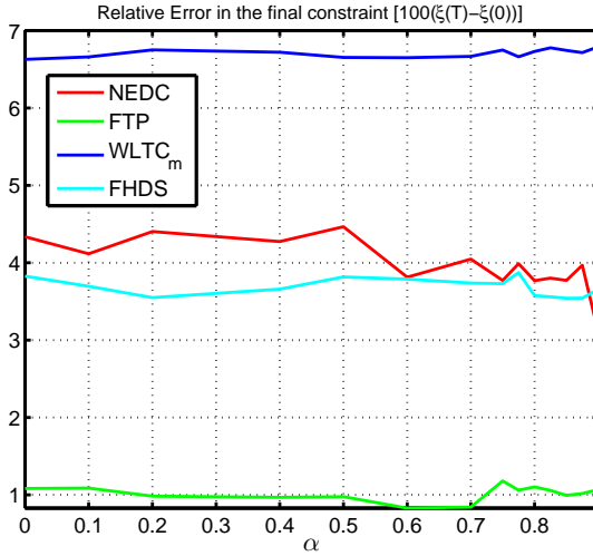
Figure 6.12: Final constraint satisfaction
