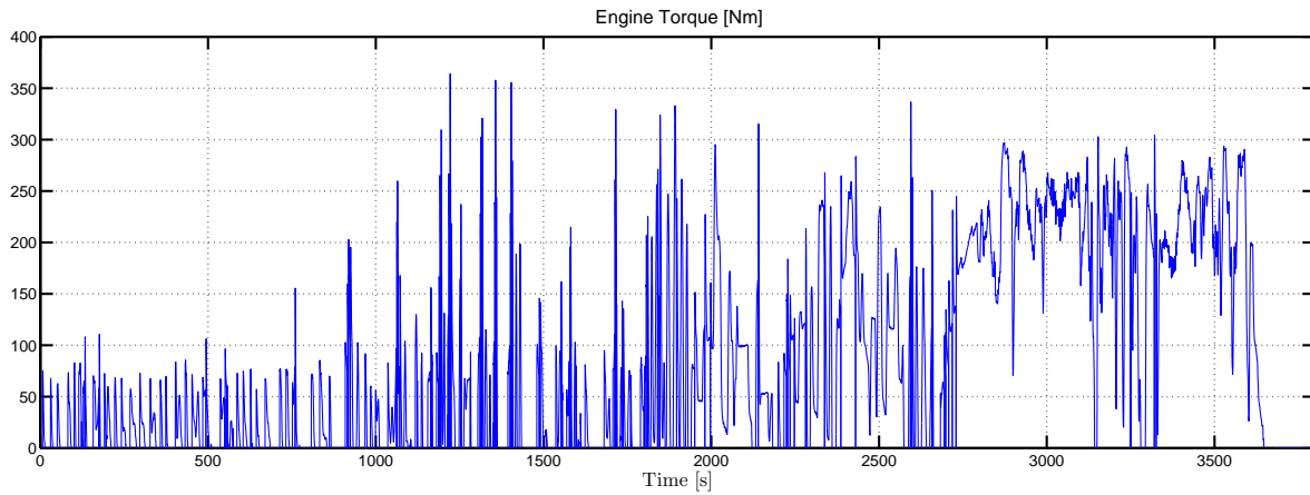
Figure G.14: Engine torque set points [Nm] for Vc 2 -Test
