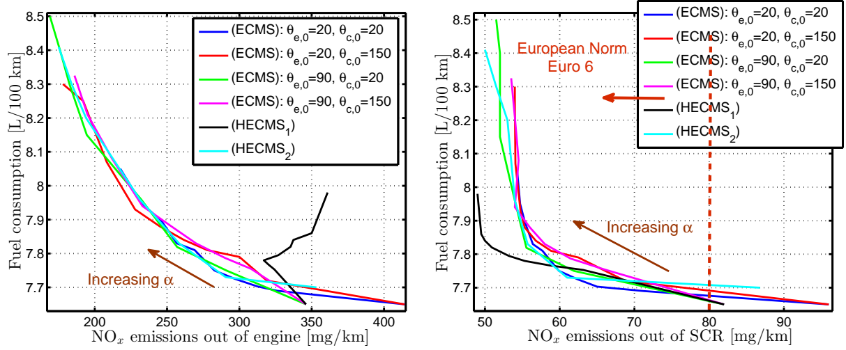
Figure 7.32: Fuel Consumption [L/100 km] as a function of NO x emissions [mg/km] out of the engine (left) and out of the SCR (right) from ECMS (xMOD platform).
