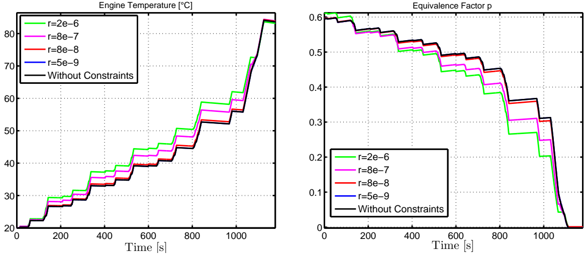
Figure B.5: Engine temperature \theta_e [°C] (left) and equivalence factor p (right) for NEDC in the constrained case
