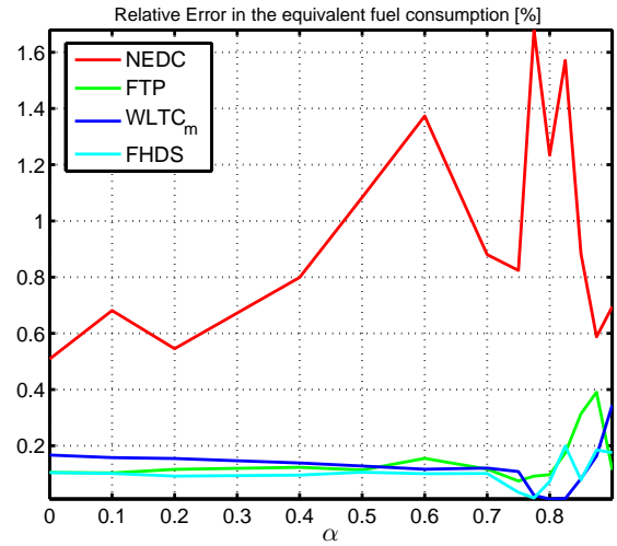
Figure 6.13: Relative error in equivalent fuel consumption [%]
