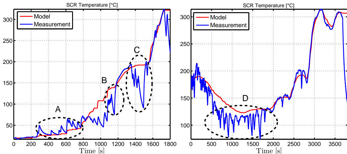
Figure 7.22: Temperature \theta_c [°C] for Vc_1 -Test 7 Figure 7.23: Temperature \theta_c [°C] for Vc_2 -Test
