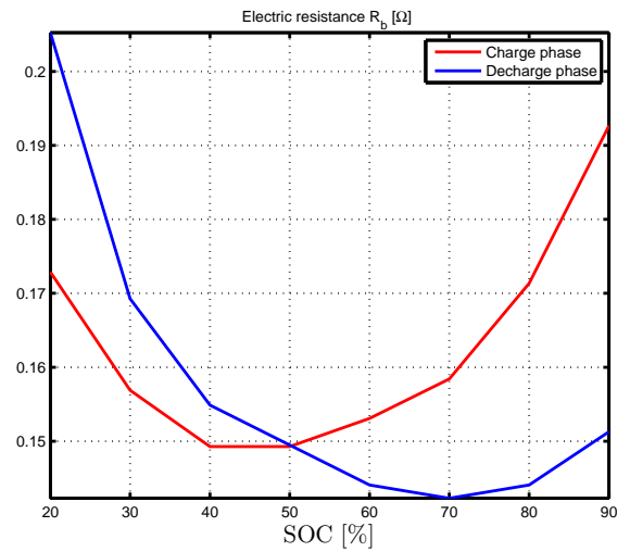
Figure 7.9: Battery internal resistance R_b [Ω]
