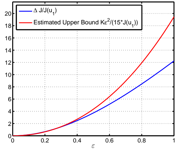
Figure 5.2: Relative error in the optimal cost
