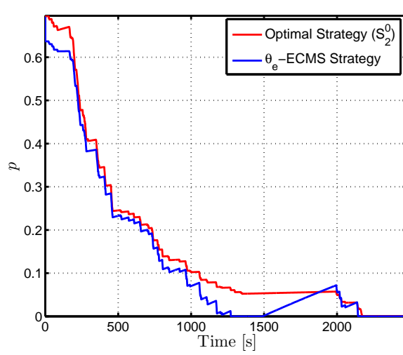
Figure B.14: Equivalence factor p
