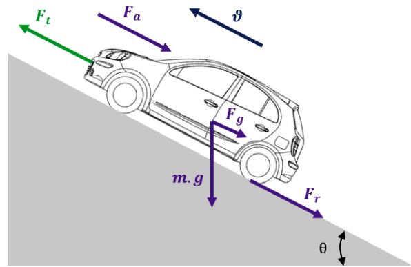
Figure 3.2: Schematic representation of the forces acting on the vehicle
