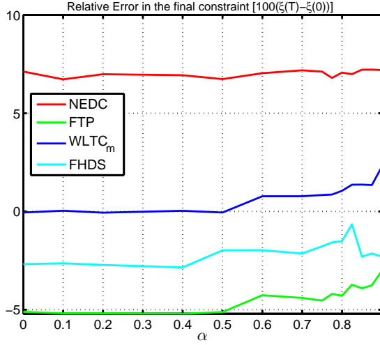
Figure 6.8: Final constraint satisfaction
