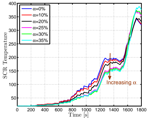
Figure 7.30: SCR temperature [°C] using ( HS_1 )
