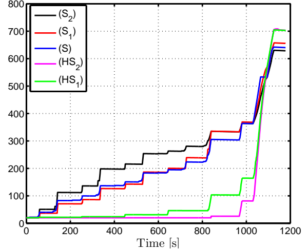
Figure 4.7: Histories of simulated catalyst temperature \theta_c [°C] obtained from optimal input calculated for \alpha = 0.8
