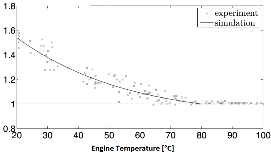
Figure 1.2: Typical excess fuel consumption of the engine as a function of engine temperature [87].
