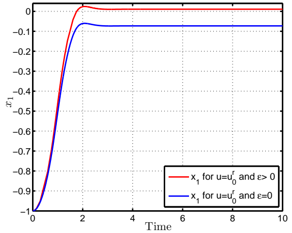
Figure 5.15: x_1 for \varepsilon = 0.09 and r < r_0
