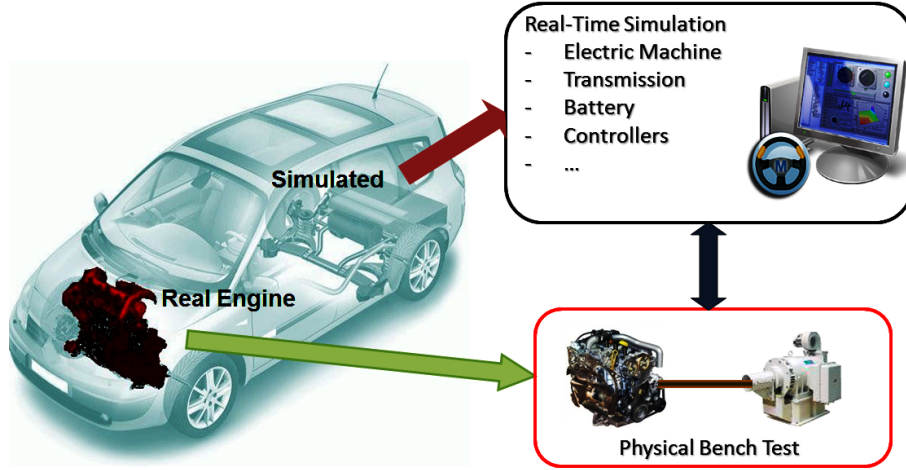
Figure 7.1: Schematics of the Hy-HiL concept
