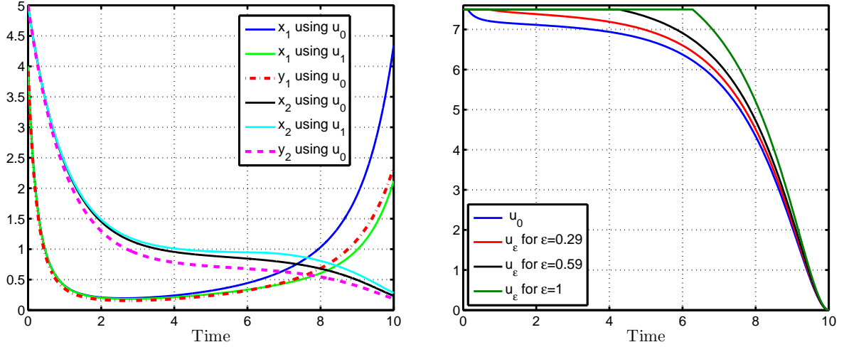
Figure 5.5: State trajectories (left) and optimal controls (right) for \epsilon = 1 for the NL problem
