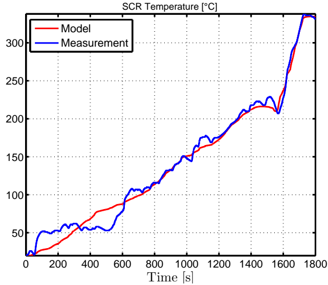
Figure 7.21: Temperature \theta_c [°C] for Ic-Test
