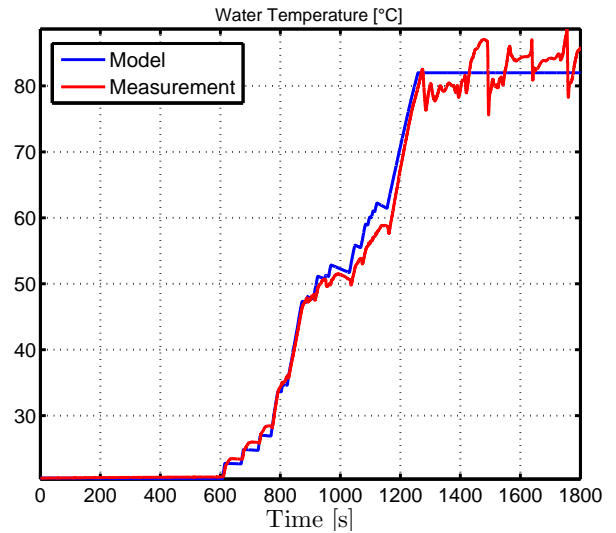
Figure 7.11: Temperature \theta_e [°C] for Ve 1 -Test 3 Figure 7.12: Temperature \theta_e [°C] for Ve 2 -Test
