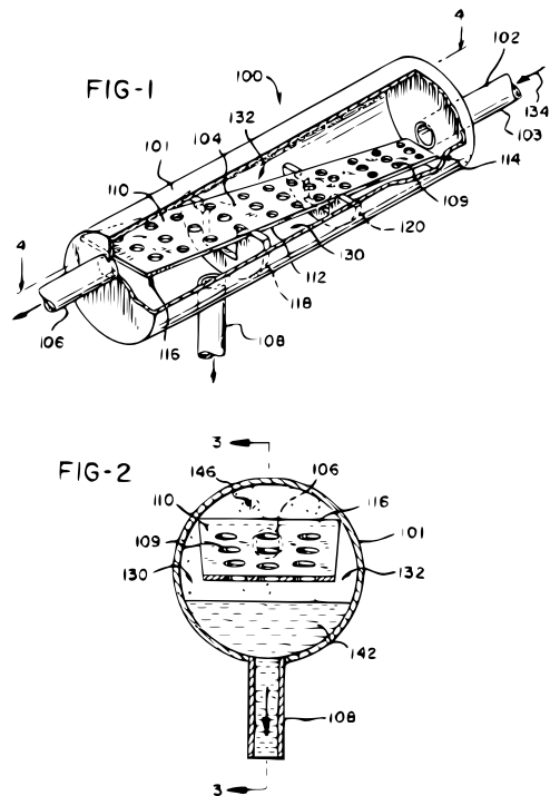
Figure 50 Brevet US5507858A (1996): gestion des transitoires
