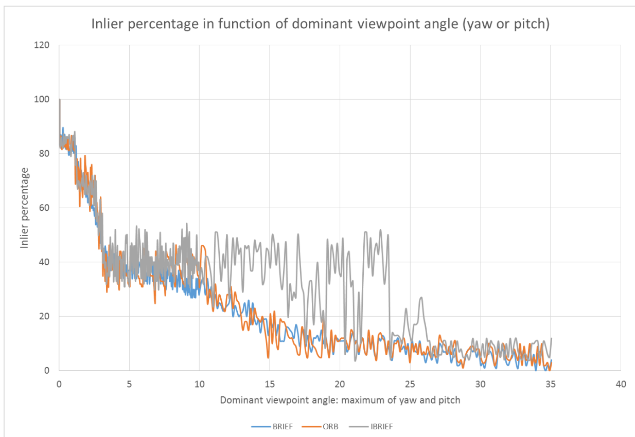
Figure 2-15: Inlier percentage in function of the highest viewpoint angle (max of yaw and pitch) for sequence 2.
