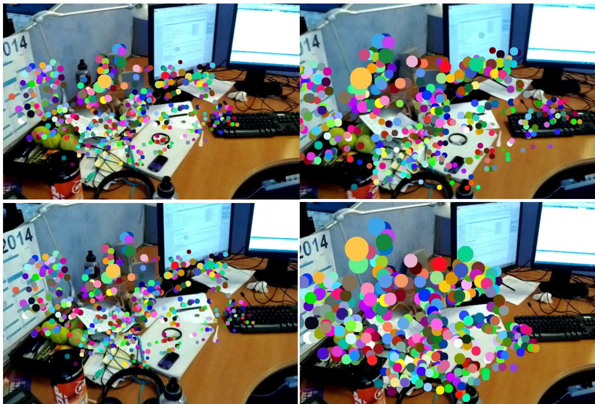
Figure 4-6: Two frames from the same video as Figure 4-4. Top shows the first frame, bottom row the second. Left frames show the UKF-SLAM results, right frames show the PnP RANSAC results.
