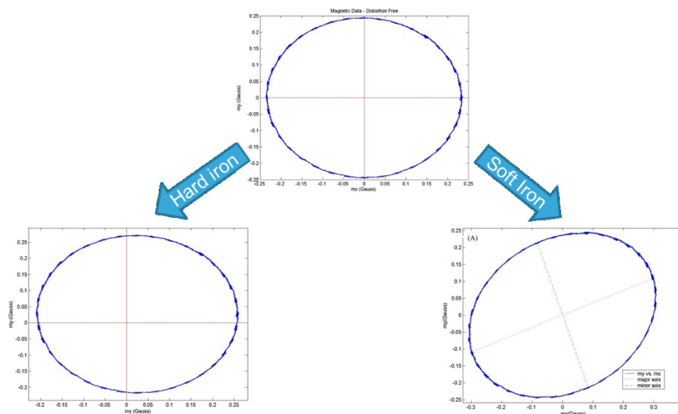
Figure 1-5: The effect of soft and hard iron on a magnetometer when performing a 360° turn.
