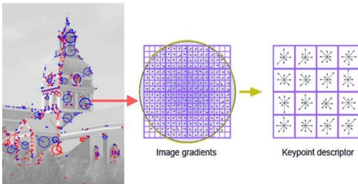
Figure 2-3: Feature description with SIFT, courtesy of 7 .
