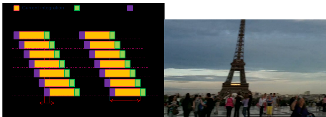
Figure 1-3: Left: Rolling Shutter readout system. Right: Example of skew due to Rolling Shutter distortions.
