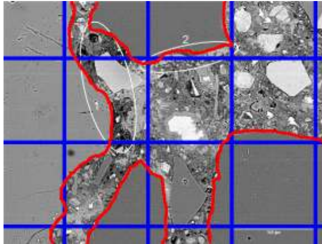
FIGURE 2.11 – A blue 100 \mu\text{m} grid is put on top of a SEM image from Scrivener et al. (2004). The red lines indicate the largest inclusions. The cement paste is clearly heterogeneous over a 10 \mu\text{m} voxel.
