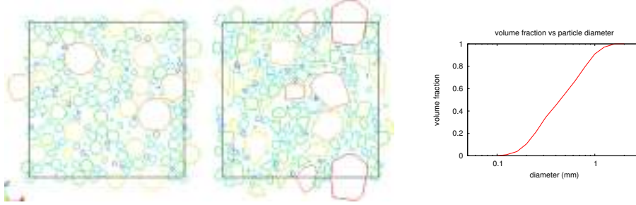
FIGURE 2.4 – On the left, polyhedra are rather round whereas polyhedra feature sharp edges in the middle. The RSA algorithm has been used. The sieve curve of the corresponding mortar is presented on the right.
