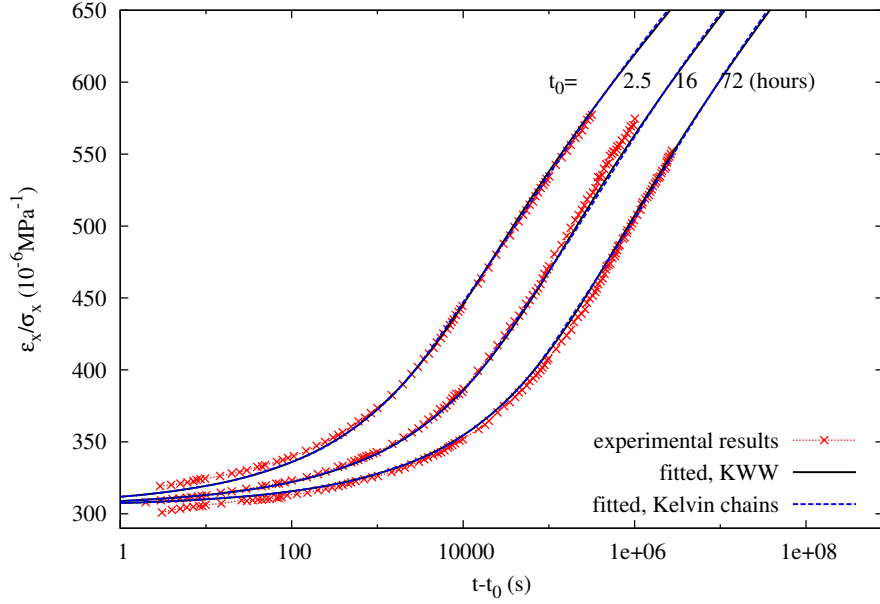
FIGURE 5.3 – The experimental results of Read et. al. Read et al. (1992) on hard polyvinyl chloride (PVC) at T=23^\circ\text{C} are digitalized. First parameters of aging \mu and of the KWW function are fitted according to these curves. Then a series of Kelvin chains is adjusted to the KWW function to enable 3D numerical computations (blue).
