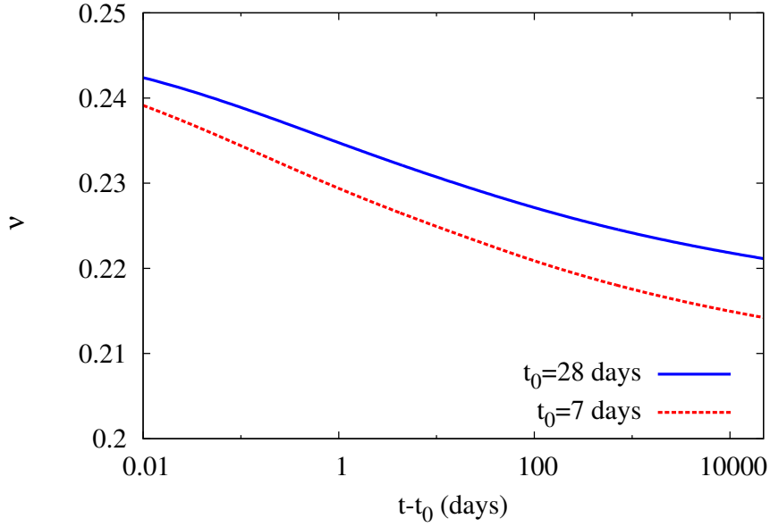
FIGURE 6.4 – The viscoelastic Poisson's ratio \nu of the cement paste is estimated : a bulk relaxation test and a shear relaxation test are performed based on the relaxation tensor estimated by the Mori–Tanaka scheme and equation (6.7) is applied. The viscoelastic Poisson's ratio \nu changes with time of loading t_0 and time elapsed since loading t . Consequently, the approximated viscoelastic Eshelby's tensor is needed at the mesoscopic scale.
