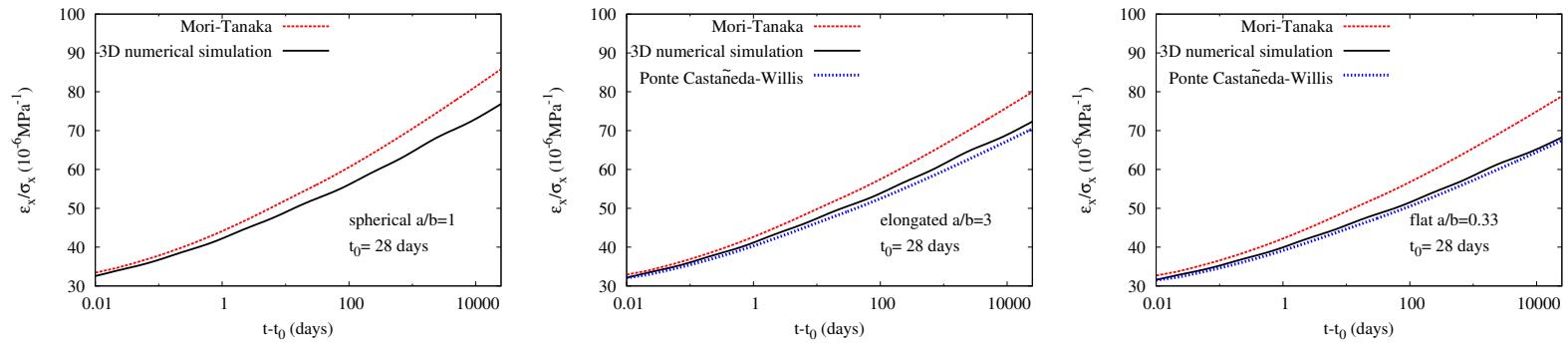
FIGURE 3.8 – The normalized creep strains \epsilon_x/\sigma_x of concretes estimated by the Mori-Tanaka scheme, the Ponte Castañeda-Willis scheme and full 3D numerical simulations are displayed as functions of the time elapsed since loading t - t_0 . Considered aspect ratios of aggregates for these uniaxial creep tests are a/b = 1 (left), a/b = 3 (center) and a/b = 0.33 (right). The time of loading is t_0 = 28 days. In case of spherical inclusions a/b = 1 , the estimate of the Ponte Castañeda-Willis scheme is equal to the one of the Mori-Tanaka scheme.
