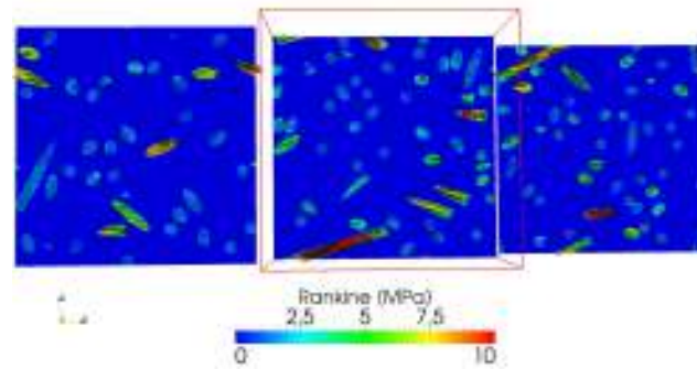
FIGURE 5.19 – The Rankine criteria in fibers as computed by 3D numerical computation of an uniaxial creep test \sigma_x = 1\text{MPa} . Three slices are displayed. Fibers parallel to axis x feature larger Rankine criteria. Black lines correspond to the direction of the maximal principal stress in fiber. This direction is parallel to the axis of the fiber.
