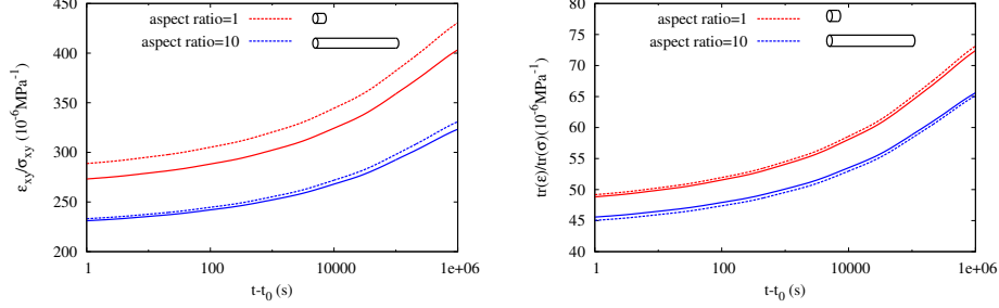
FIGURE 5.12 – Overall responses estimated by the Mori-Tanaka scheme (dashed lines) and 3D numerical computations (solid lines) for fiber-reinforced polymers featuring different lengths of fibers. A shear creep test \sigma_{xy} = 1 (left) and a hydrostatic creep test tr(\sigma) = 1 (right) are performed. The Mori-Tanaka scheme manages to capture the influence of the aspect ratio. The volume fraction of fibers is 20%.
