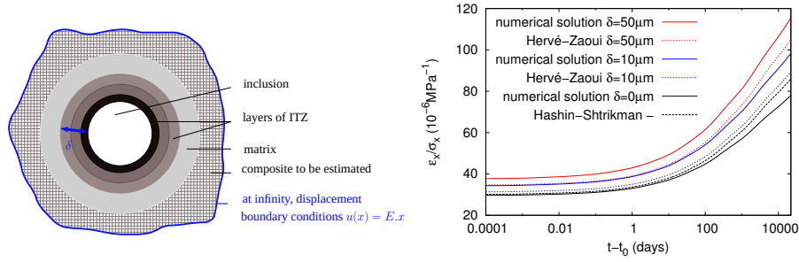
FIGURE 2.16 – Results of the n+1 phase spherical model (left) Hervé and Zaoui (1993) for a mortar is compared to numerical estimates for different thickness of ITZ \delta . The n+1 phase spherical model underestimates the time dependent strain in case of a creep test (right).
