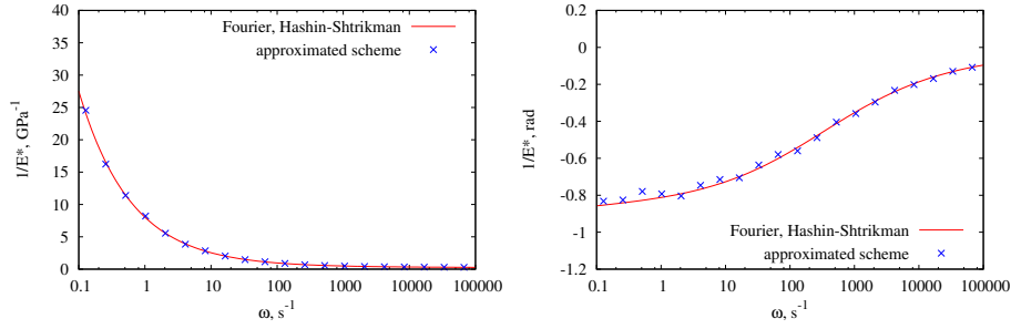
FIGURE 6.2 – The magnitude (left) and phase (right) of the inverse of the complex Young modulus estimated by the Fourier method and the proposed homogenization scheme coincide at all frequencies. \omega .
