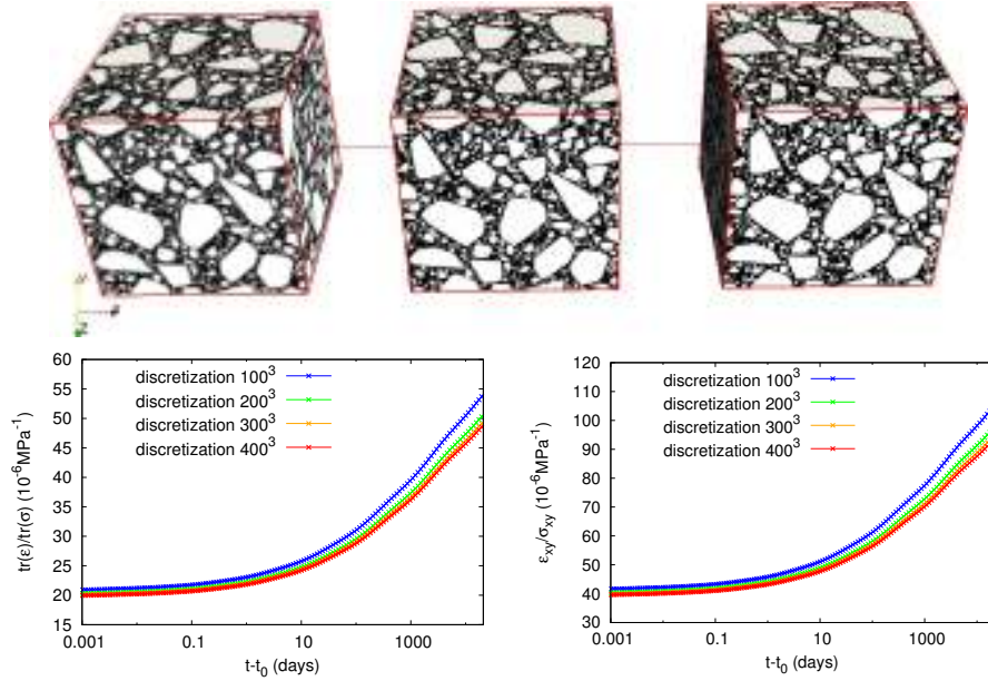
FIGURE 2.7 – Top : One microstructure of concrete of size 40 mm made of 63% of inclusions at discretization 100^3 , 200^3 and 400^3 . Bottom : The delayed responses to hydrostatic (left) and shear(right) creep tests are computed.
