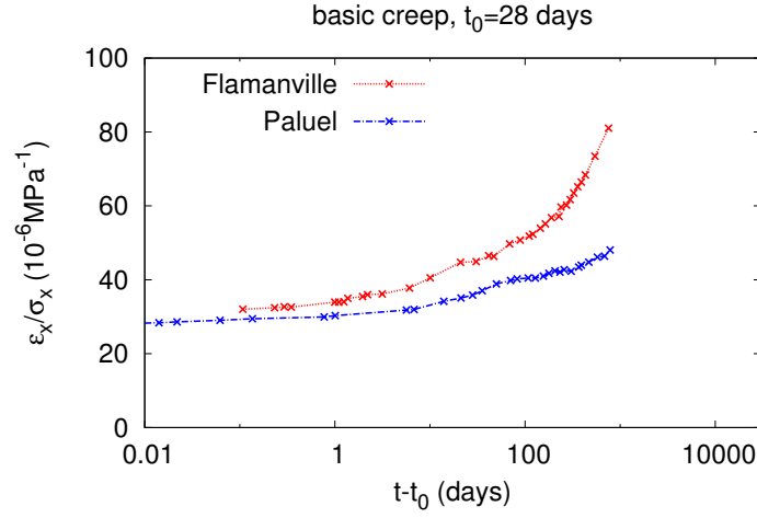
FIGURE 2.1 – Results of uniaxial compressive creep tests reported by L. Granger (1995). Although the formulations of concretes from Flamanville and Paluel were comparable, the basic creep strain ( 10^{-6}\text{MPa}^{-1} vs days) proved different. The compressive stress was 12 MPa and the concrete was loaded at t_0 = 28 days.
