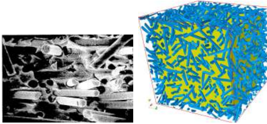
(a) Photomicrograph of a cross section of a fiber-reinforced plastic, the cross section being of a fractured tensile dumb-bell Rahrig (1985). The distribution of the orientations of fibers does not seem isotropic and this particular sample exhibits fiber-matrix debonding. The failure mode highly depends on the coupling agent Rahrig (1985). (b) a 400\mu\text{m} -wide sample of a fiber-reinforced plastic by the RSA algorithm is shown. The volume fraction of fibers in the cubic cell is 15%. Fibers are 10\mu\text{m} in diameter and 100\mu\text{m} in length.
