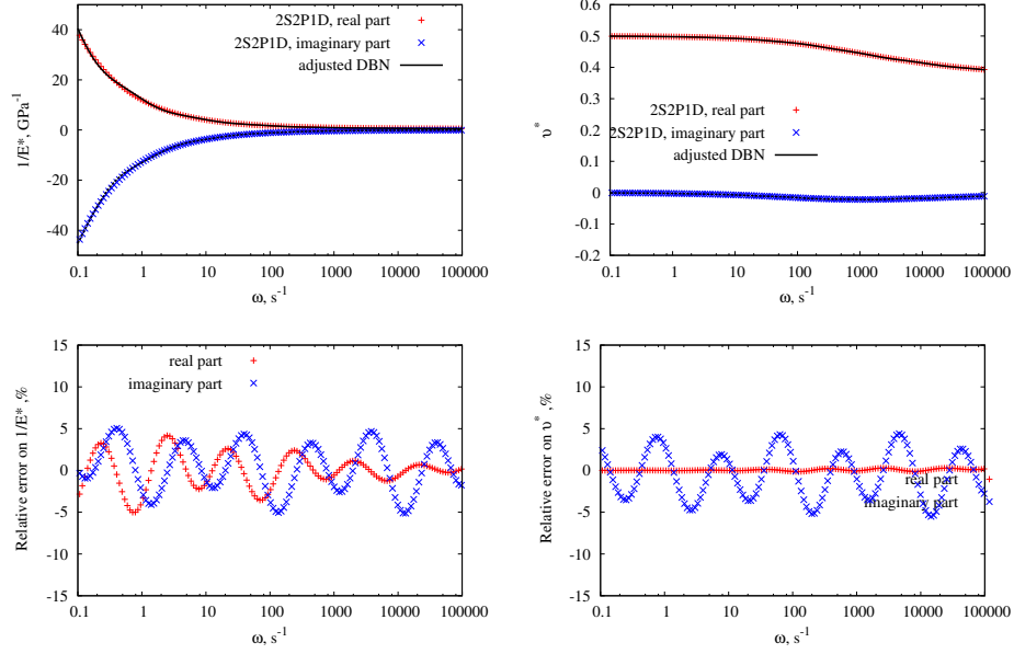
FIGURE 6.1 – The DBN model is adjusted to the 2S2P1D model of a bitumen (Di Benedetto et al., 2007) in the range [0.1\text{Hz}; 1000\text{Hz}] . The obtained real and imaginary parts of the complex Young Modulus (top left) and Poisson's ratio (top right) are displayed as functions of the pulsation \omega . The corresponding relative error are displayed below.
