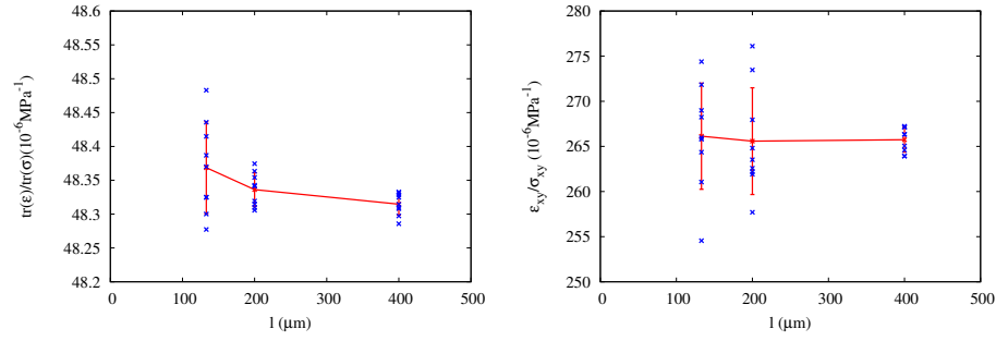
(b) On the left, the overall responses to an hydrostatic stress is displayed as a function of the size of the unit cell. On the right, a shear stress is considered. The red lines and error bars correspond to averages and standard deviation respectively. As the size of the unit cell increases, the estimate of the overall response becomes less variable.
