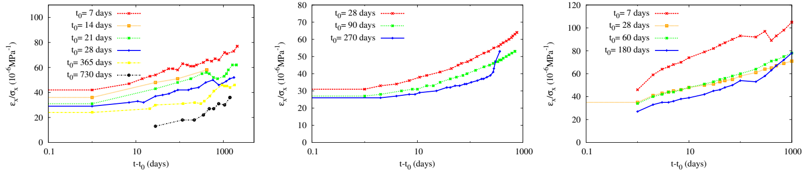
(a) w/c = 0.49 , a/c = 4.814 (L'Hermite and Mamillan, 1969) and (b) w/c = 0.381 , a/c = 4.339 (Kommendant et al., 1976) (c) w/c = 0.42 , a/c = 4.4 (Browne and Blundell, 1969)
