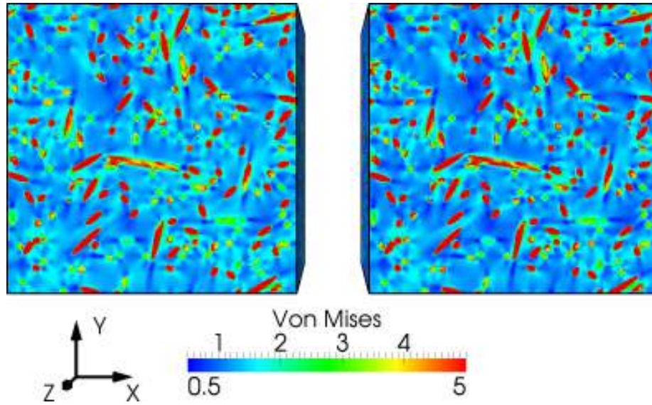
FIGURE 5.14 – Stress concentrations in a fiber-reinforced polymer may be estimated by 3D numerical computations. A numerical shear creep test \sigma_{xy} = 1 is performed and the Von Mises stress is displayed at t - t_0 = 0 (left) and t - t_0 = 50 days (right). It is noticeable that the Von Mises stress is highly variable in the matrix. These stress concentrations do not change much over time : the fibers already bear much of the loading at the time of loading. N = 384 , l = 200\mu\text{m}
