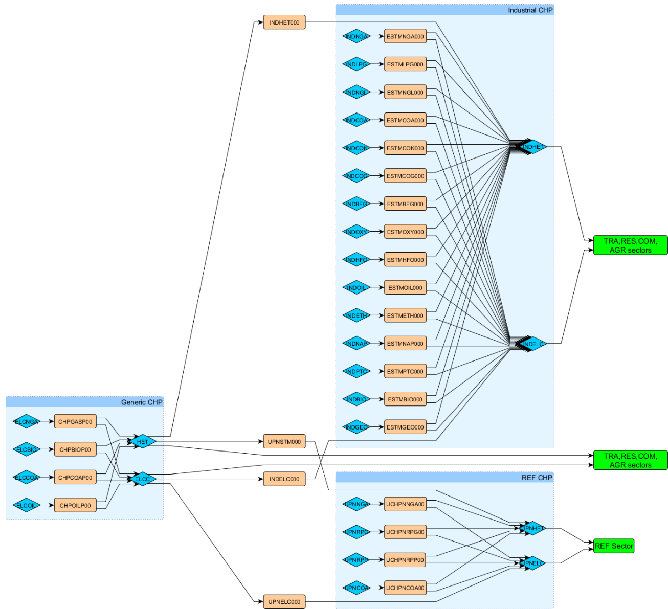
Figure 0-1: CHP representation in T-ALyC
