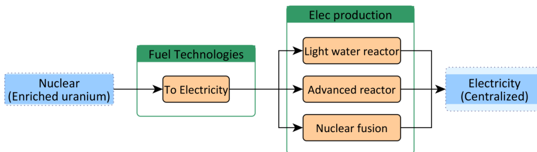
Figure 3-24: Structure of the nuclear module in T-ALyC
