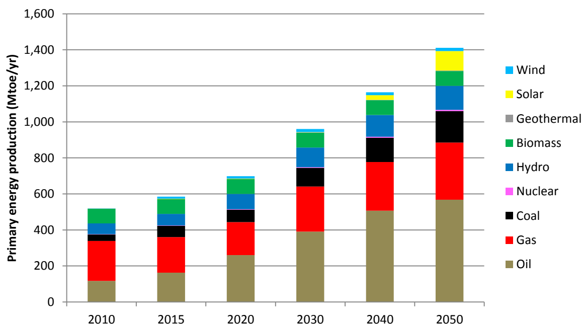
Figure 5-14: Primary energy consumption in BAU case, 2010-2050 – Net of trade
