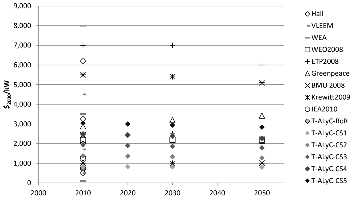
Figure 3-19: T-ALyC hydro costs – comparison with existing literature (adapted from Kumar et al., 2011)
