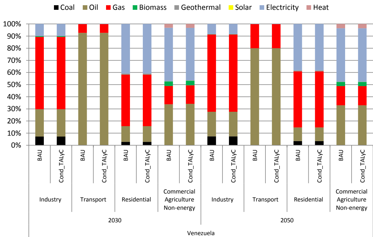
Figure 0-2: End-use consumption according to consumptions sectors, in BAU and Cond_TALyC scenarios (subregion detail)
