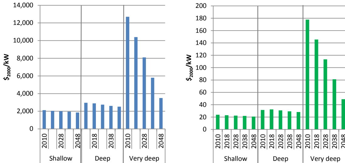
Figure 3-23: Investment costs (left) and O&M costs (right) for geothermal-based electricity production in T-ALyC
