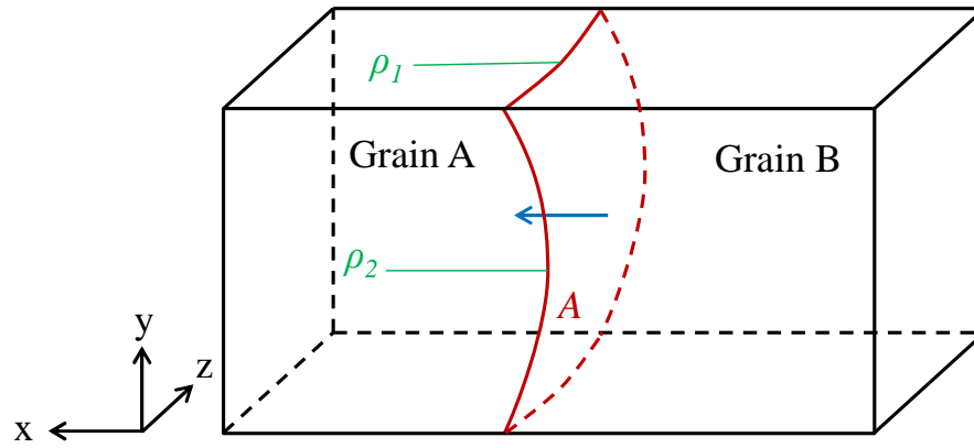
Figure 3.1: Schematic diagram of a grain boundary of area A and principal radii of curvature \rho_1 and \rho_2 moving in order to reduce interfacial energy.
