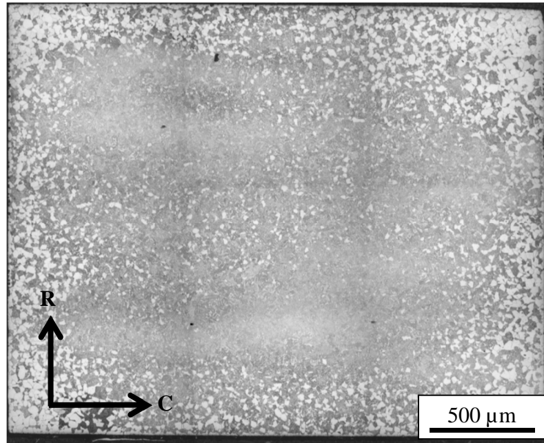
Figure 2.16: Optical micrography showing change in microstructure due to microsegregations. Equiaxial ferrite is bright. The fully bainitic dark bands along the radial-circumferential plane correspond to the chemically enriched zones. Horizontal and vertical dark lines are artifacts due to stitching of multiple images.
