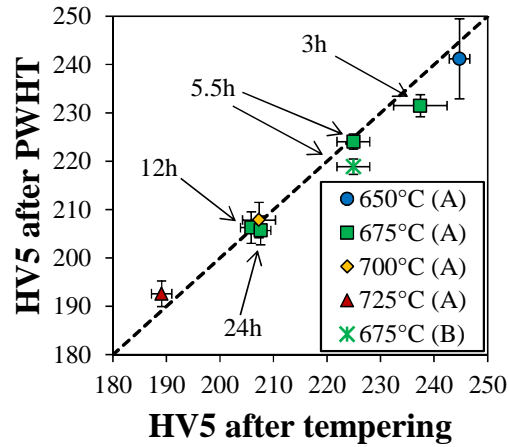
Figure 6.13: Comparison between hardness before and after PWHT. The 650°C, 700°C and 725°C correspond to 5.5 hours of tempering at these temperatures. A and B refer to the applied PWHT.
