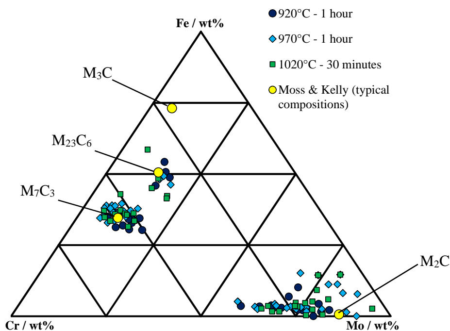
Figure C.1: Carbide chemical composition in metallic elements after three different austenitization conditions, followed by cooling at 0.3^{\circ}\text{C}/\text{s} , tempering at 675^{\circ}\text{C} for 5.5 hours and stress-relieving heat treatment at 625^{\circ}\text{C} for 16 hours.
