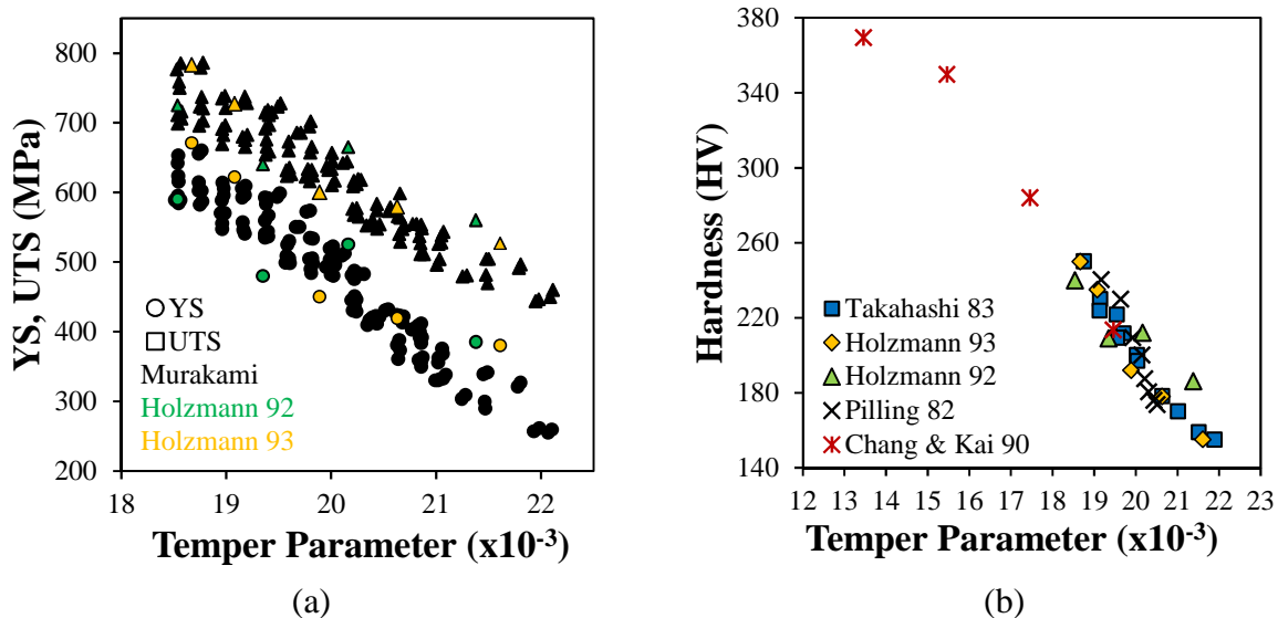
Figure 6.2: Relationship between tempering conditions and (a) Yield strength (YS) and ultimate tensile strength (UTS), (b) Vickers hardness of 2.25Cr – 1Mo steels. From [4, 84, 101, 116–118]
