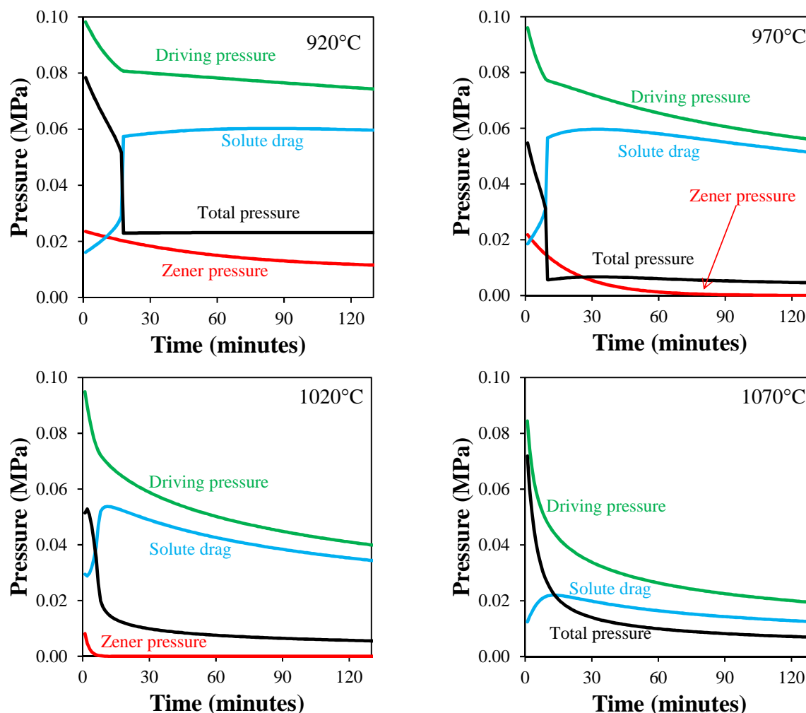
Figure 3.23: Contributions from the different pressures exerted on the grain boundary at different temperatures.
