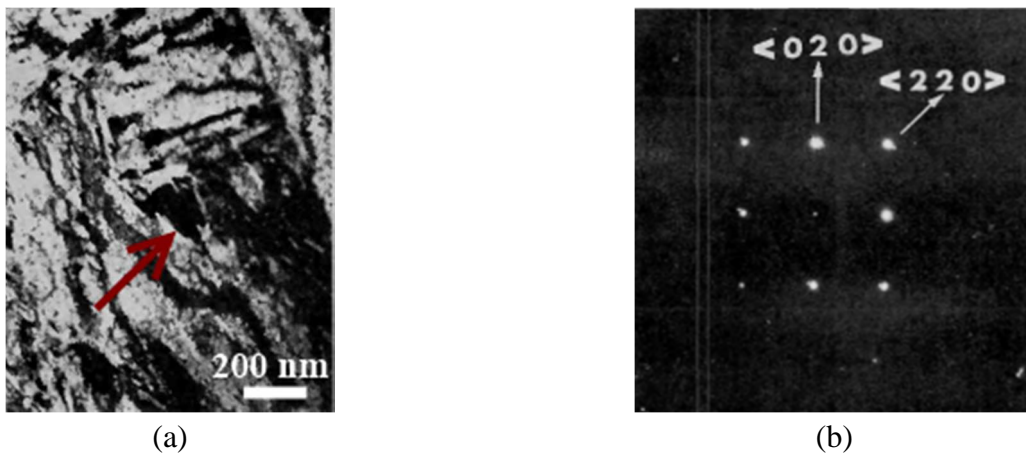
Figure 5.4: (a) TEM thin foil observation of cubic M_2C within bainitic laths (b) Corresponding electron diffraction pattern. B = (001) . From [109].
