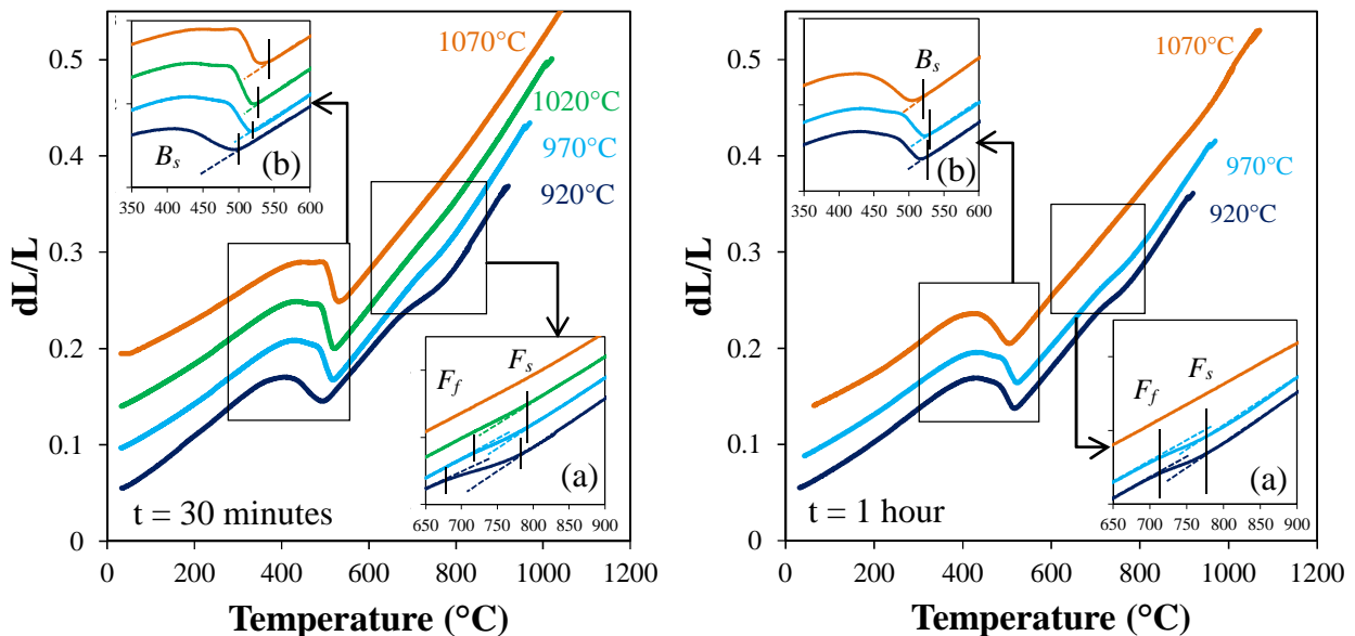
Figure 4.3: Dilatometric curves upon cooling at 0.3^\circ\text{C/s} from different austenitization temperatures for 30 minutes and 1 hour. Insets (a) and (b) are enlarged views of ferritic and bainitic transformations, respectively.
