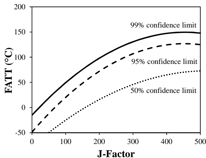
Figure 1.1: Effect of impurities ( J -factor) on the fracture appearance transition temperature ( FATT ). Probability curves based on historical data collection for base and weld metals, aged from 20 000 hours to 200 000 hours. From [2]
