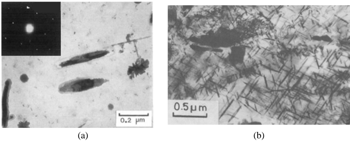
Figure 5.3: TEM observations on carbon extraction replicas: (a) M_2C carbides with the corresponding electron diffraction pattern. B = (10\bar{1}1) (from [98]), (b) Numerous M_2C carbides forming a Widmanstätten pattern in the matrix (from [103]).
