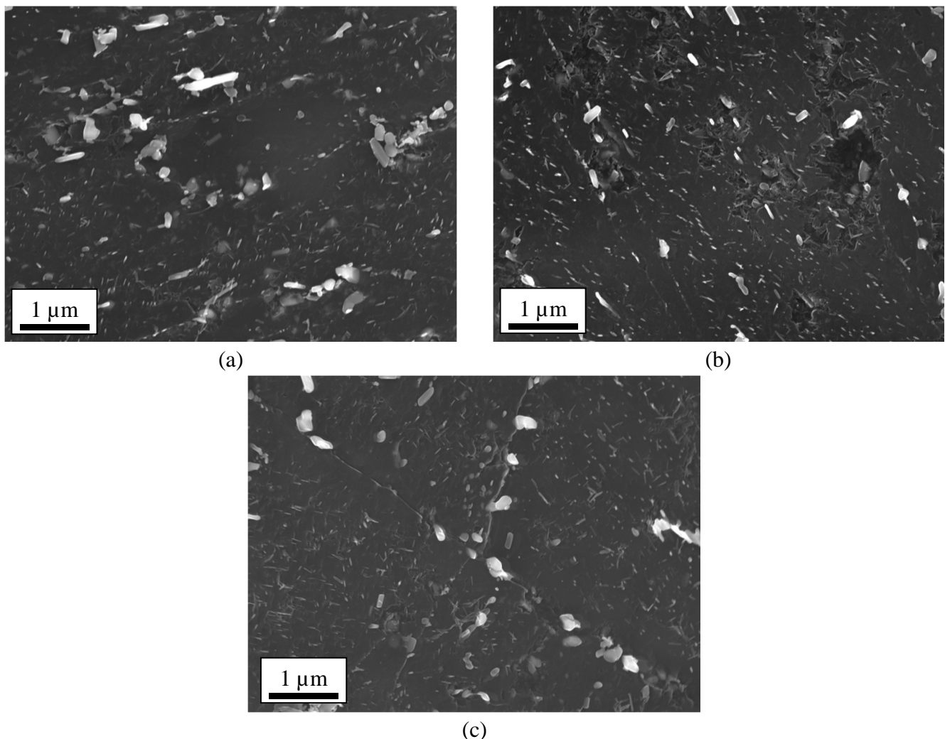
Figure 4.15: SEM Observations on carbon extraction replicas. Tempering condition is 675^\circ\text{C} - 5.5\ \text{h} + 625^\circ\text{C} - 16\ \text{h} . Austenitization conditions are (a) 920^\circ\text{C} - 1\ \text{hour} , (b) 970^\circ\text{C} - 1\ \text{hour} , (c) 1020^\circ\text{C} - 30\ \text{min} .
