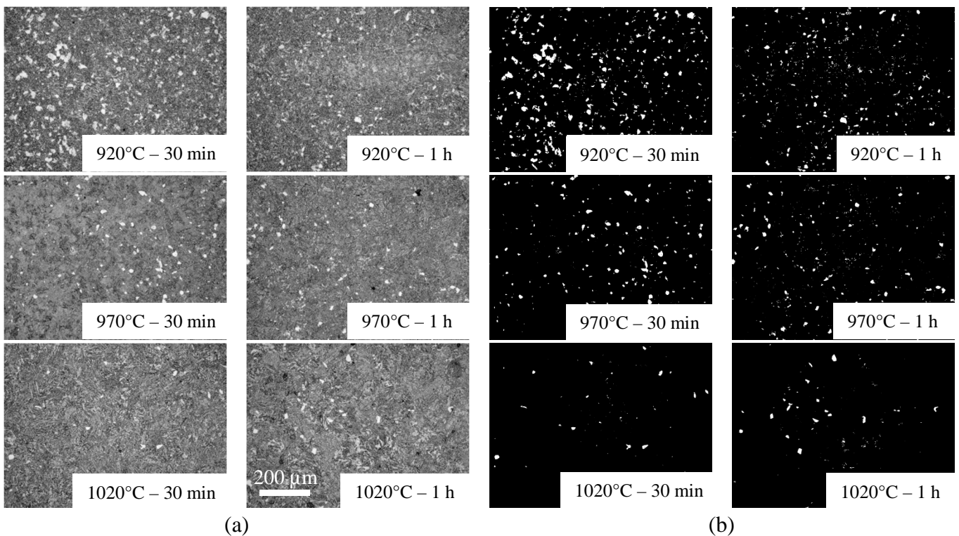
Figure 4.4: Optical micrographs after cooling at 0.3°C/s for different austenitization conditions. (a) Optical micrographs, (b) Binned images using the lower threshold.
