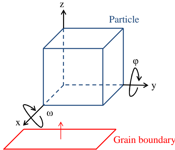
Figure 3.4: Schematic diagram of a cubic particle. The orientation relative to the grain boundary is described by angles \omega and \varphi
