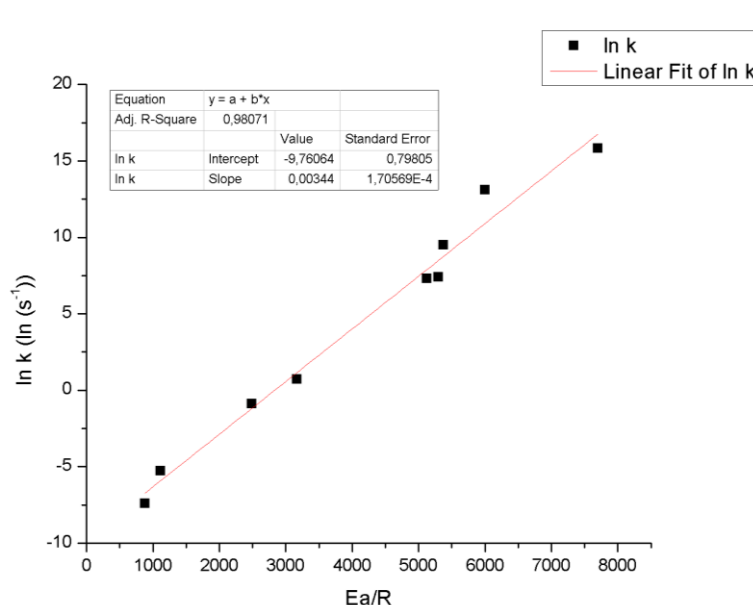
Figure 1.4: Plot of \ln K vs. E/R of the values obtained by Adapted from Tewari et al. (2002)
