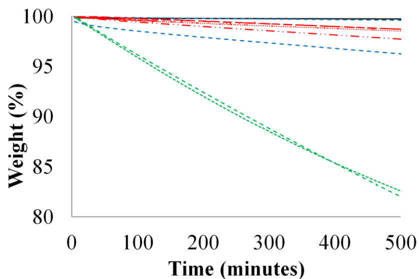
Figure 1: TGA of methyl linolenate at 40 ° C (—), 60°C (—), 80°C (—) and 110°C (—), nitrogen atmosphere
