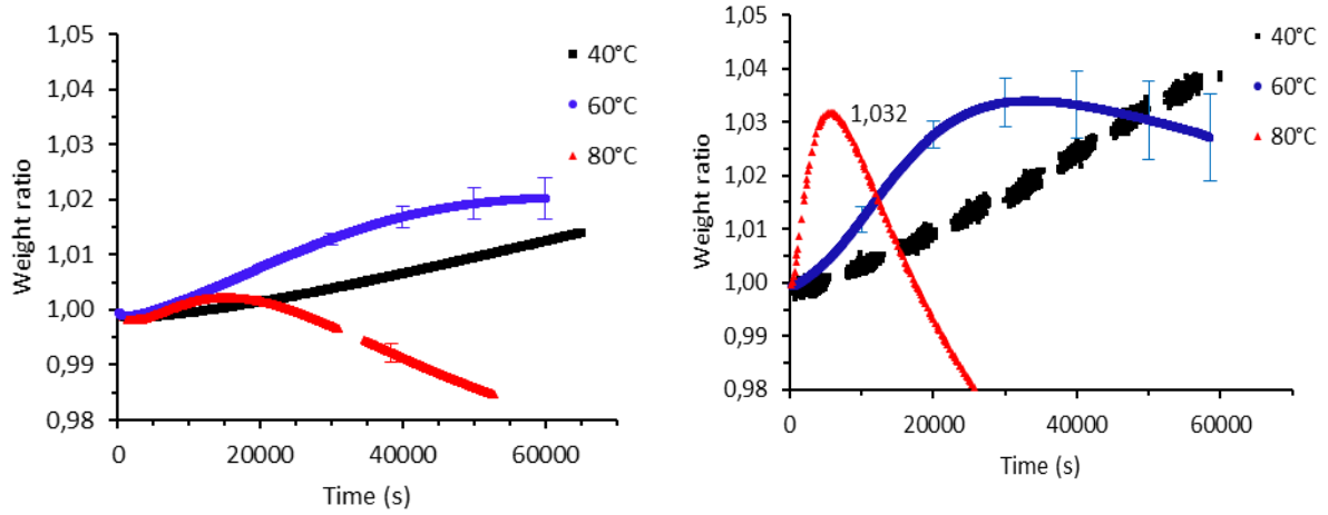
Figure 4.12: comparison of TGA results of methyl oleate in air atmosphere (left) and oxygen atmosphere (right)
