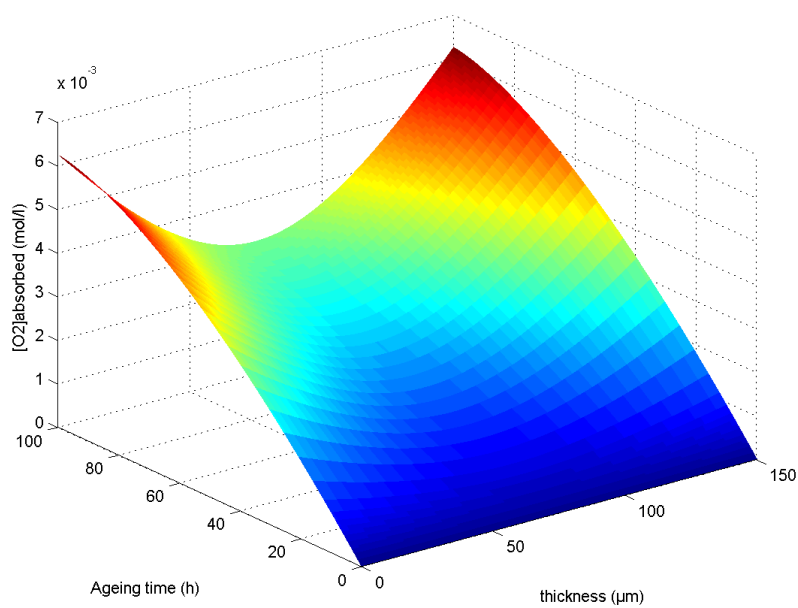
Figure 5.13: Oxygen absorbed simulations of linseed oil/PP in 5% oxygen for 150 \mu\text{m} thick film
