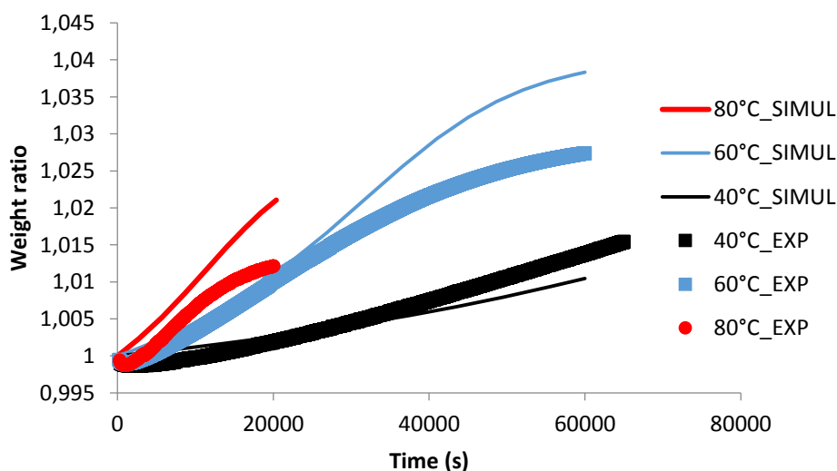
Figure 5.2: Weight ratio simulations of linolenate mass changes in air (solid line) and experimental data.
