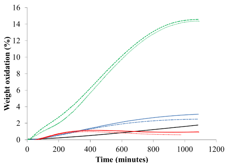
Figure 4: Results from TGA of methyl linolenate on air atmosphere at 40°C (—), 60°C (—), 80°C (—) and 110°C (—), expressed as W_o (equation 7)
