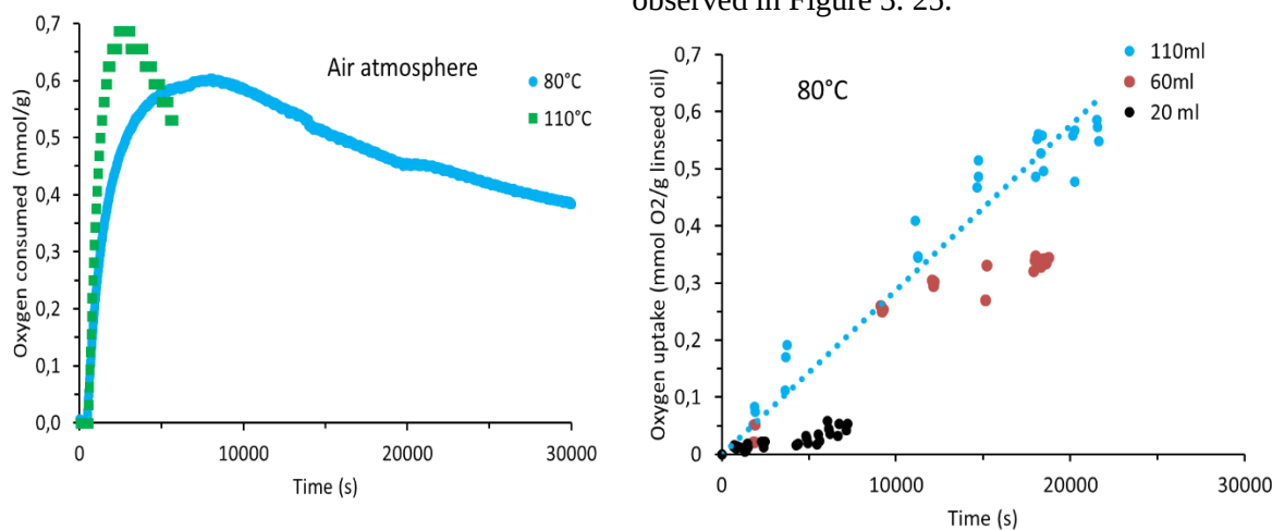
Figure 3.24: Comparison between TGA results, atmosphere of air (left) and headspace measurements (right) in terms of oxygen uptake for linseed oil.
