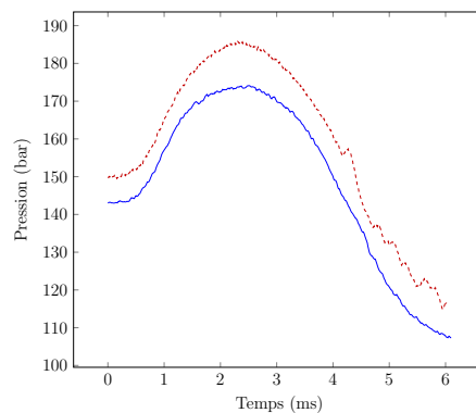
(f) Pression/temps
