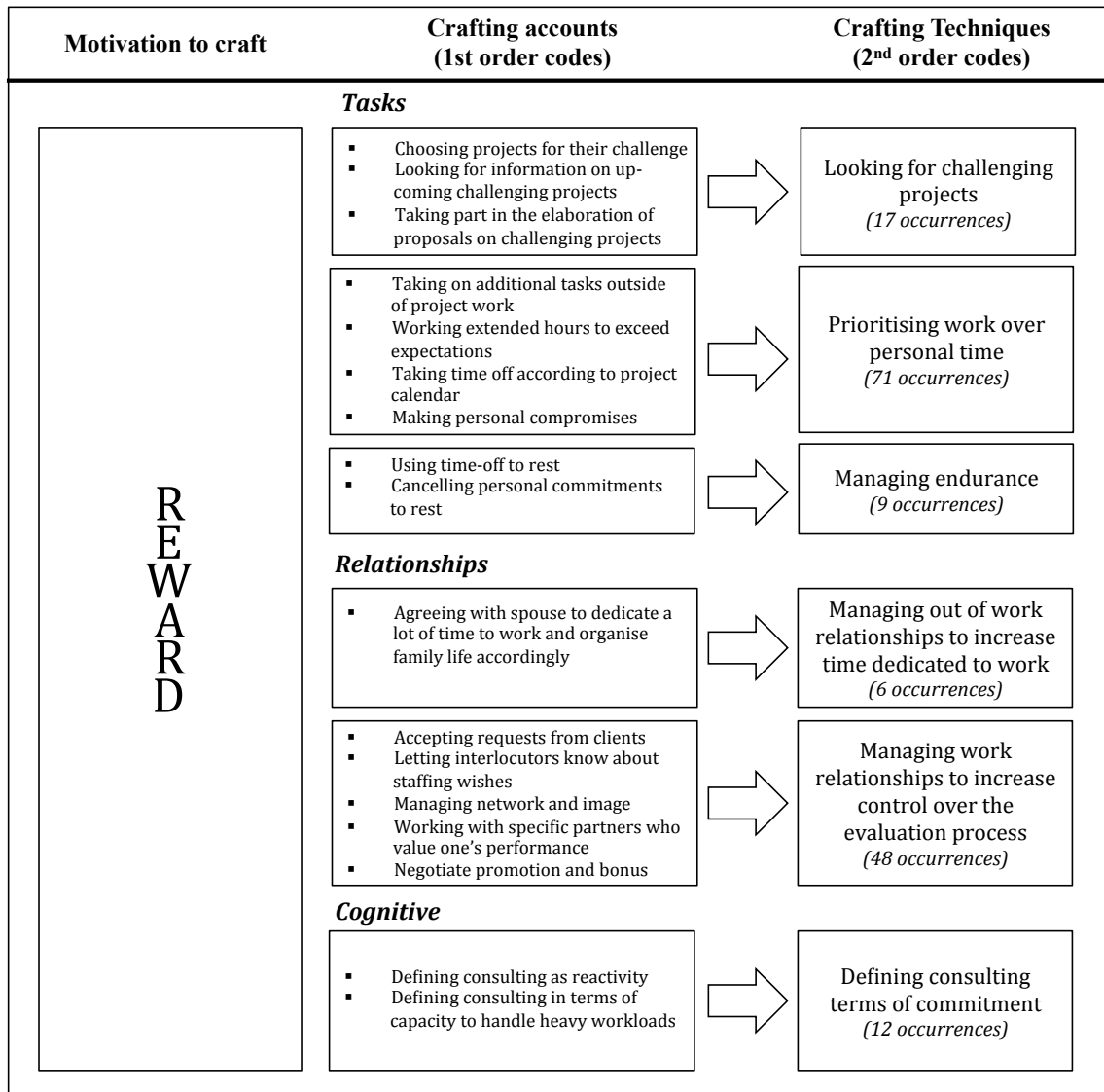
Figure 5.2a: Data structure
