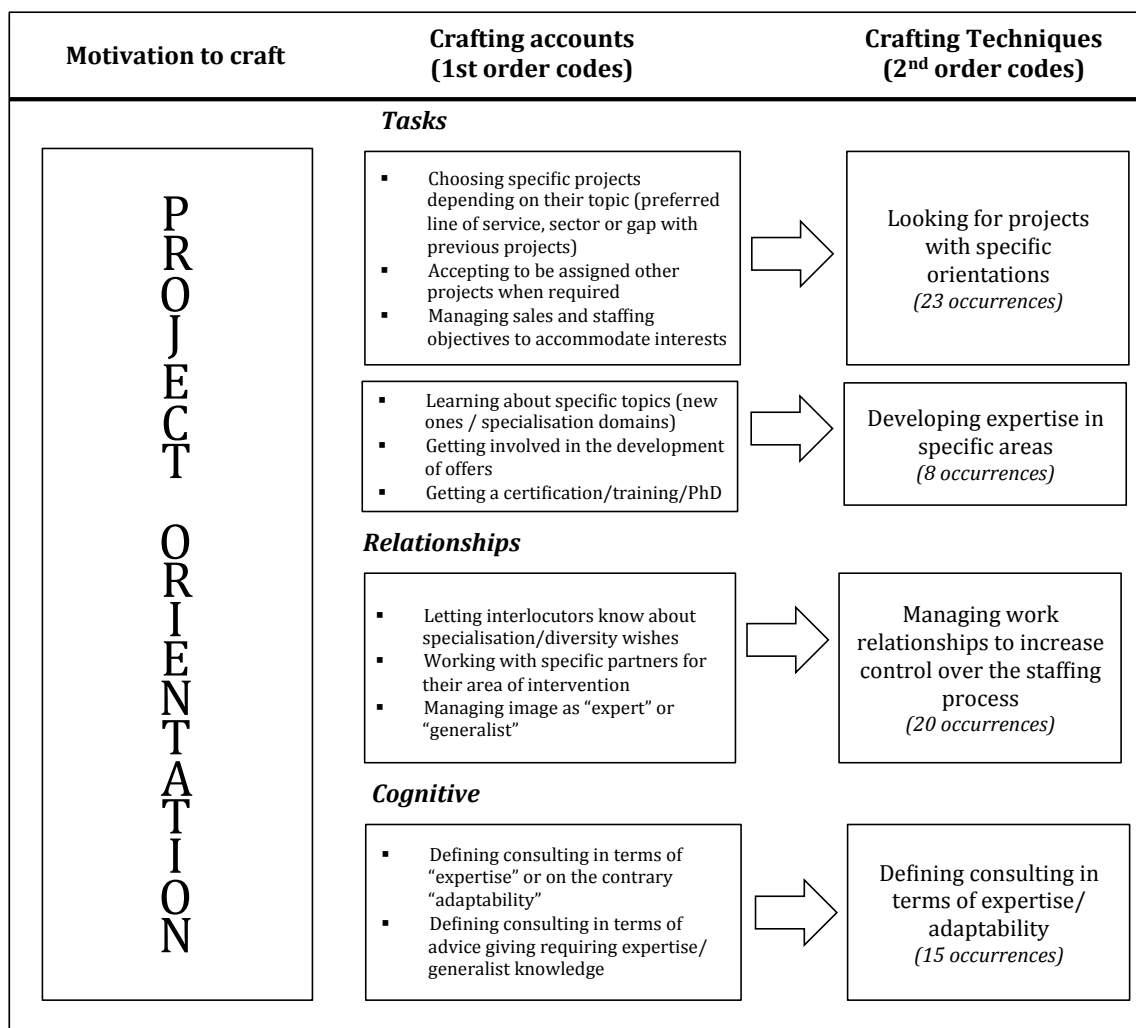
Figure 5.2b: Data structure
