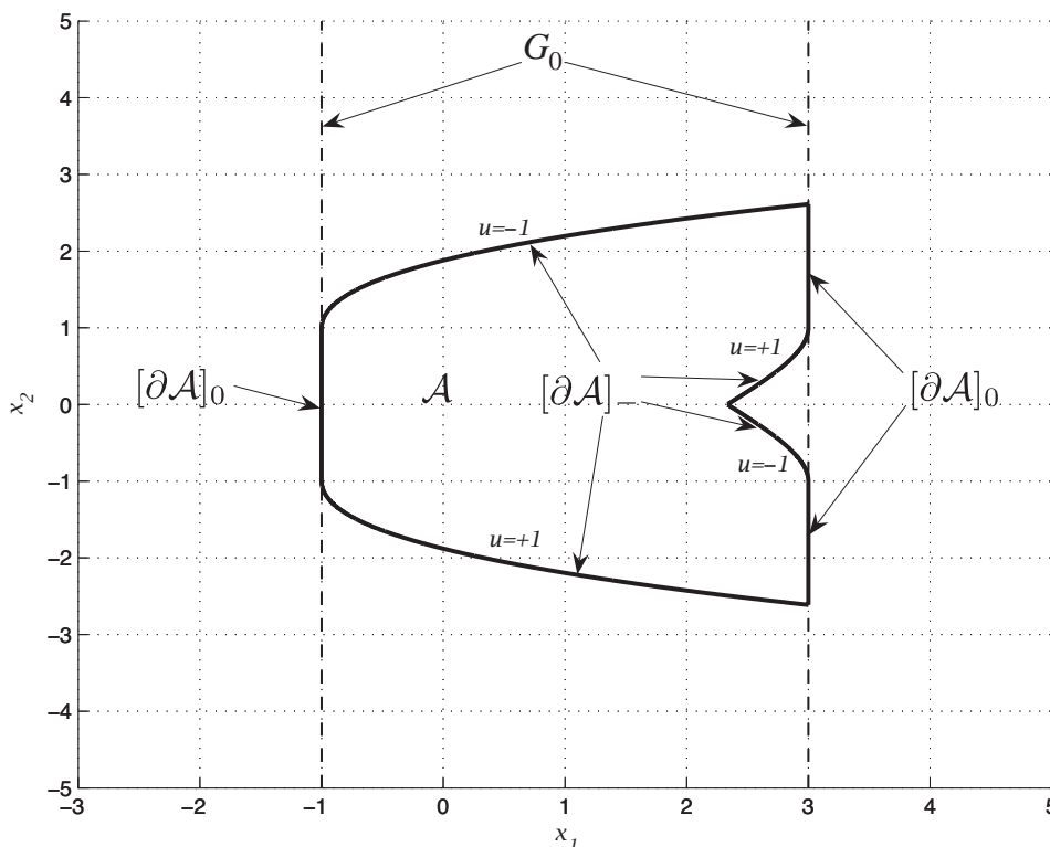
Figure 4.5: Admissible set for Example 4.3.1, from [15]
