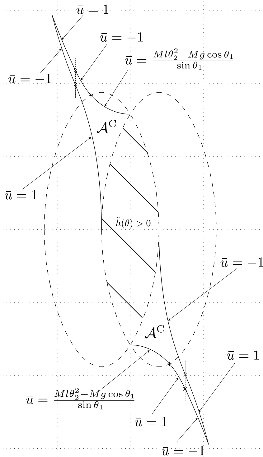
Figure 5.7: A closer look at the control associated with the barrier trajectories from the example in Figure 5.6. The crosses labelled “ \times ” correspond to \theta_1 = \pm \frac{\pi}{2} where the control switches. The crosses labelled “ + ” correspond to the points where the controls associated with the barrier trajectories arriving at (0, \pm \frac{g}{l}) switch to \frac{Ml\theta_2^2 - Mg \cos \theta_1}{\sin \theta_1} .
