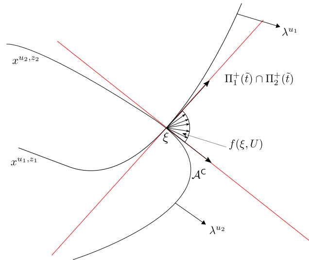
Figure 4.3: Example of a stopping point by intersection occurring in a two dimensional system. The two separating hyperplanes at \tilde{t} are marked in red and f(\xi, U) \subset \Pi_1^+(\tilde{t}) \cap \Pi_2^+(\tilde{t})
