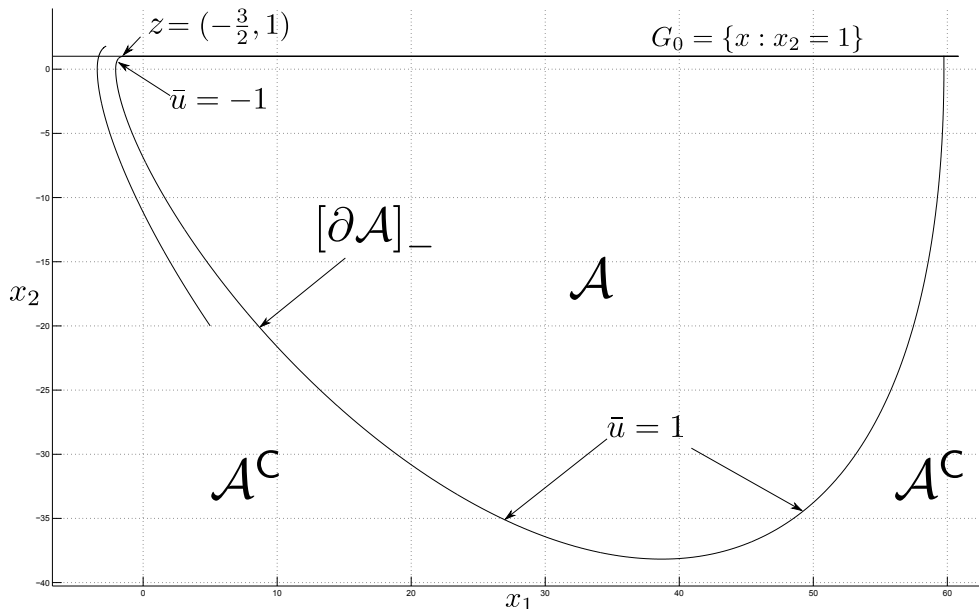
Figure 1.1: Admissible set for (1.1) with a pure state constraint. An integral curve is shown that initiates in \mathcal{A}^c , utilising the control u = +1 for x_2 \leq 0 , u = -1 for x_2 > 0 . This emphasises the semi-permeability property.
