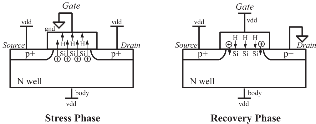
Figure 2.6: Stress and recovery phase of NBTI mechanism.
