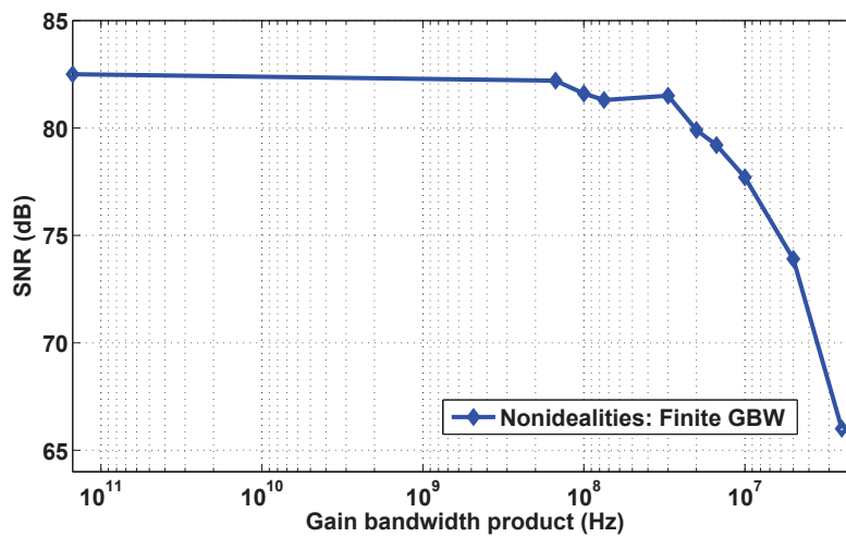
(b) SNR degradation due to nonidealities GBW
