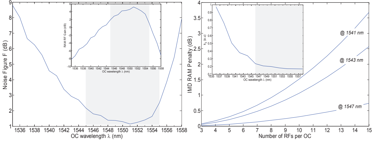
(a) Noise figure of the EAM vs. \lambda at 10mW input optical power. Inset: Modulator RF Gain. (b) IMD penalty at different OCs assuming an equally spaced RF mapping. Inset: 3^{rd} order RAM non-linearity parameter ( k_3 ).
