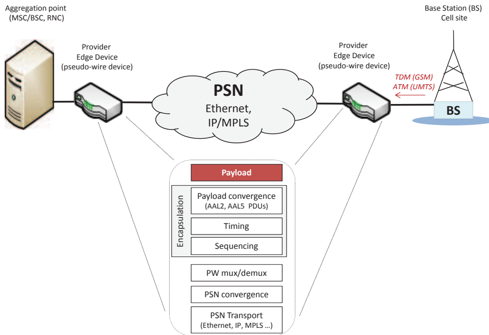
Figure 3.3: Pseudo-Wire Protocol Stack.
