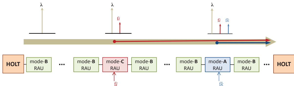
(b) An example of lightpath build as cascaded RAUs as seen by RF f_i .
