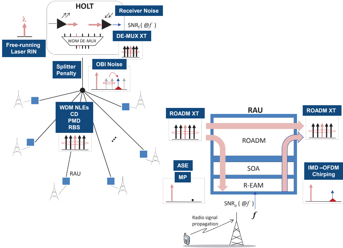
Figure 4.14: Illustration of the different impairments for a GeRoFAN tree network.
