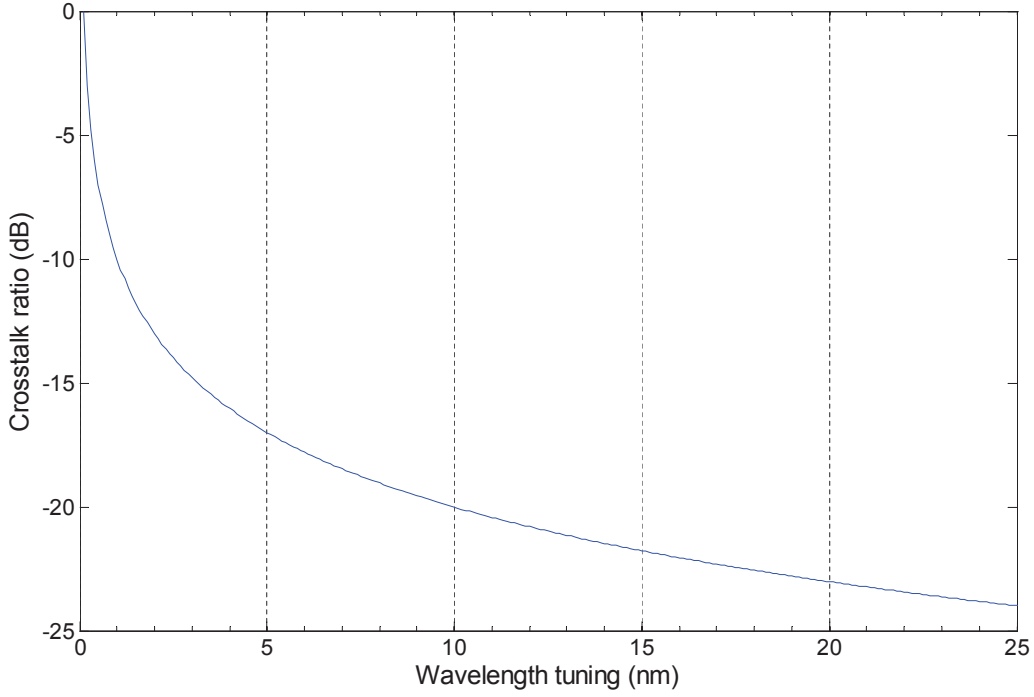
Figure 4.10: Crosstalk coefficient of a uniform BFG vs. wavelength tuning.
