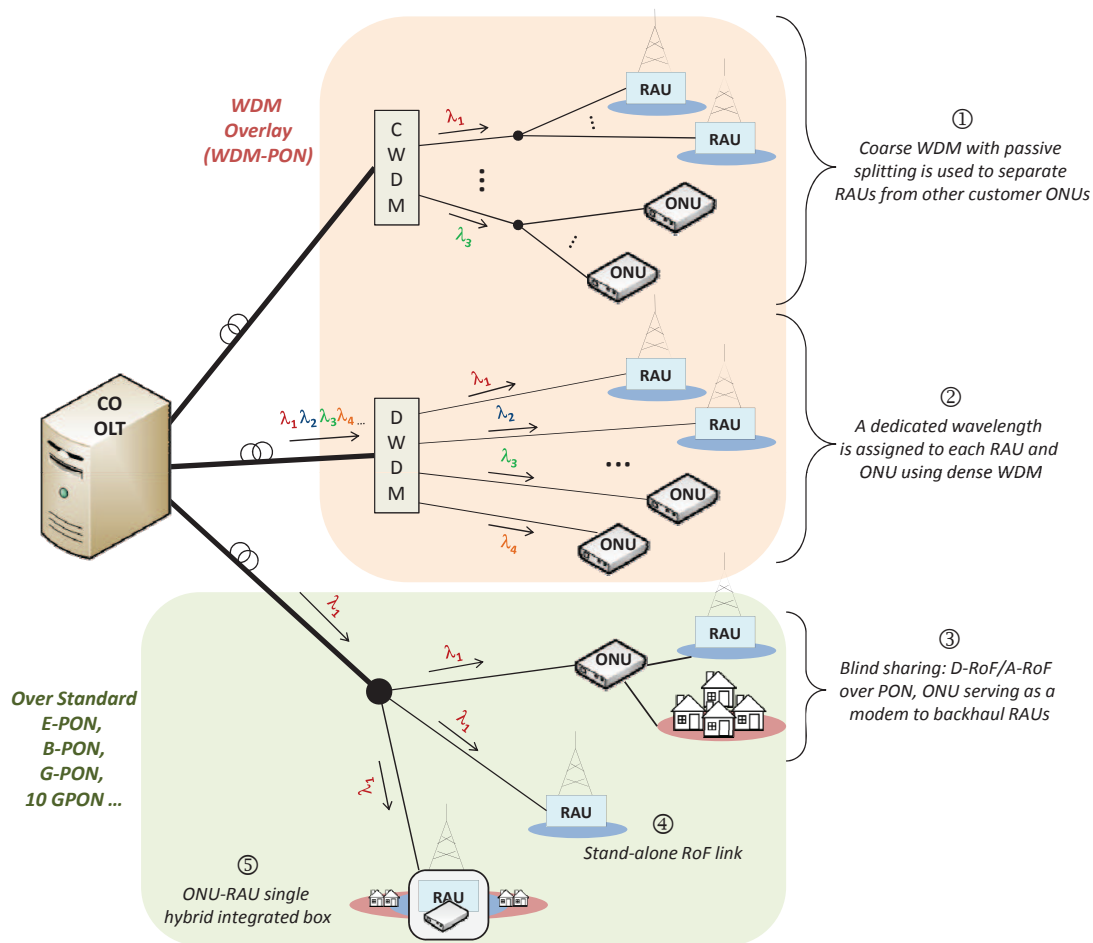
Figure 3.9: Different RoF-fixed optical broadband integration schemes.
