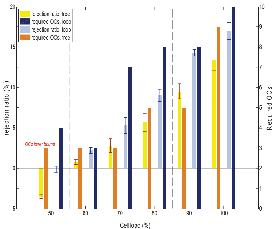
Figure 5.12: Comparison at different traffic loads between GeRoFAN loop and GeRoFAN tree in terms of rejection ratio (left axis) and number of required OCs (right axis). Error bars stand for deviation from the mean value. Negative rejection ratios indicate excess capacity beyond required by the traffic load.
