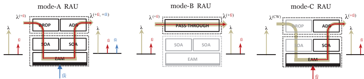
(a) Modeling RAU operating modes.
