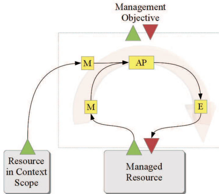
Figure 6.2: Example of modular implementation of an autonomic manager.
