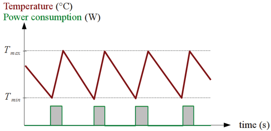
Figure 6.11: Pseudo-periodic heating cycles of a thermostatic heater, with corresponding temperature evolution.
