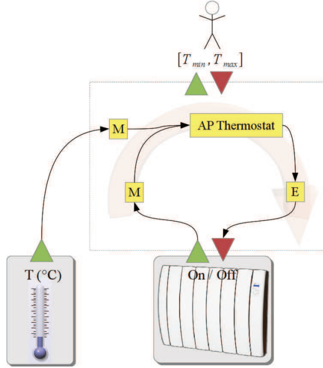
Figure 6.9: Sample design of a basic autonomic manager for a smart heater.
