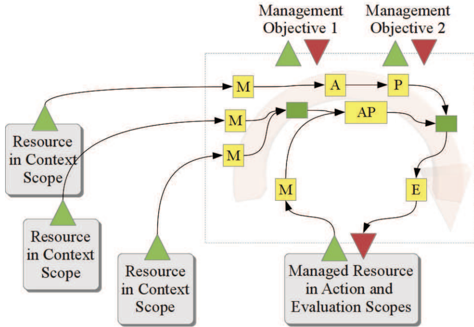
Figure 6.3: Example of a composite autonomic manager mixing control components (yellow) and integration components (green).
