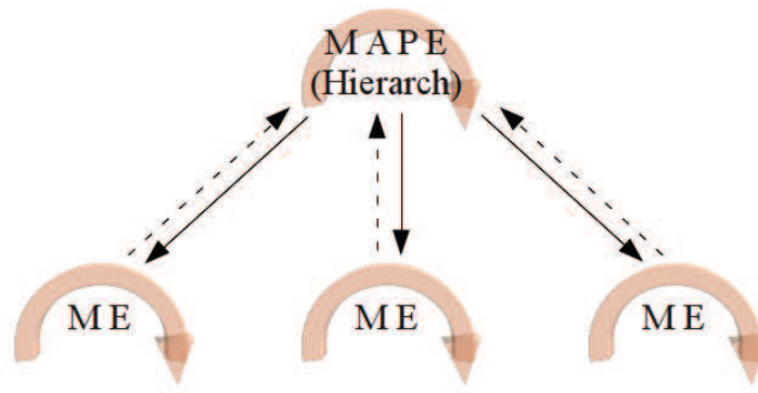
Figure 7.2: The Hierarchy pattern.
