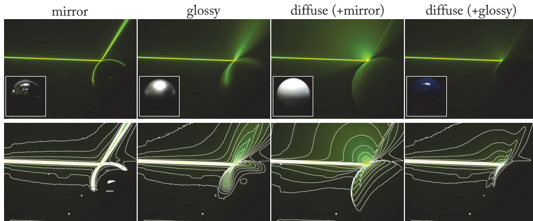
Figure 3.3: Visualization of light transport using a fluorescent fluid. Top row: Interaction of a laser with objects of different materials. Bottom row: Superimposed intensity iso-lines to visualize the lobes . Images taken from [Bor+08].
