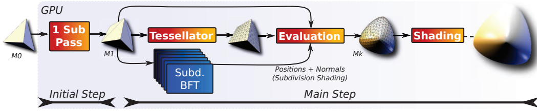
Figure 2.5: Our GPU subdivision mesh synthesis pipeline.
