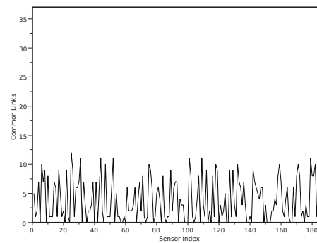
Figure 6.7: Interference on channel 2: Simultaneous communications
