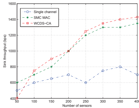
Figure 6.12: Evolution of sink throughput with network density
