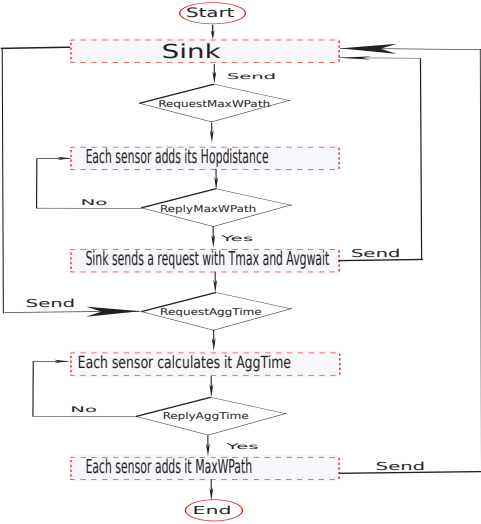
Figure 4.4: ETAPT: Algorithm
