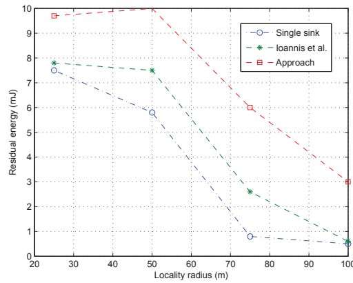
Figure 5.12: Residual energy vs. Locality radius
