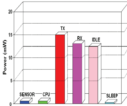
Figure 1.2: Energy consumption level [Est02]
