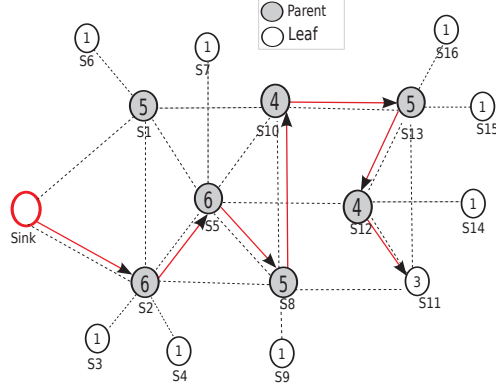
Figure 3.4: DFSA: Tree construction
