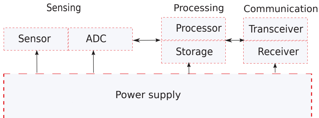
Figure 2.1: Sensor architecture
