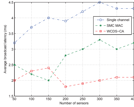
Figure 6.14: Variation of average broadcast latency with sensor density
