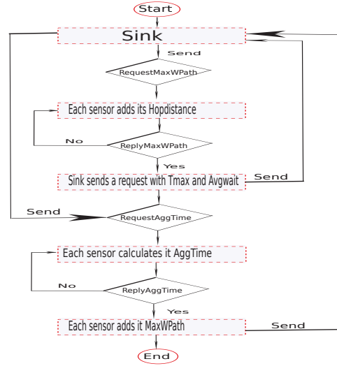
Figure 4.4: ETAPT: Algorithm
