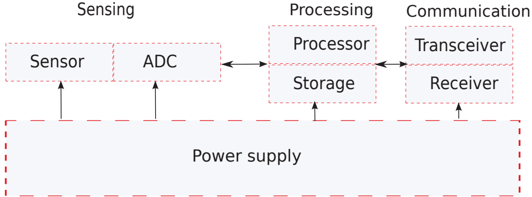
Figure 2.1: Sensor architecture
