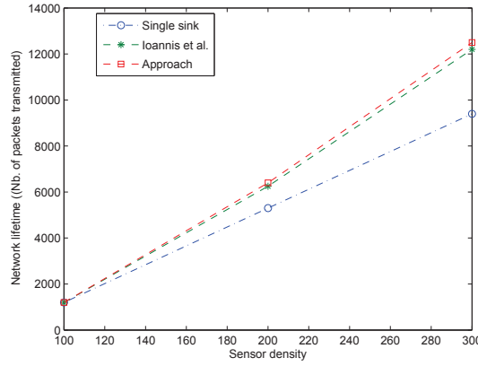
Figure 5.13: Network lifetime vs. Network density
