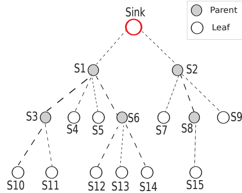
Figure 4.5: WSN: ADAPT calculation
