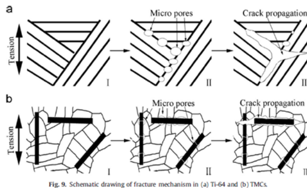
Fig. 9. Schematic drawing of fracture mechanism in (a) Ti-6Al-4V and (b) TMCs.
