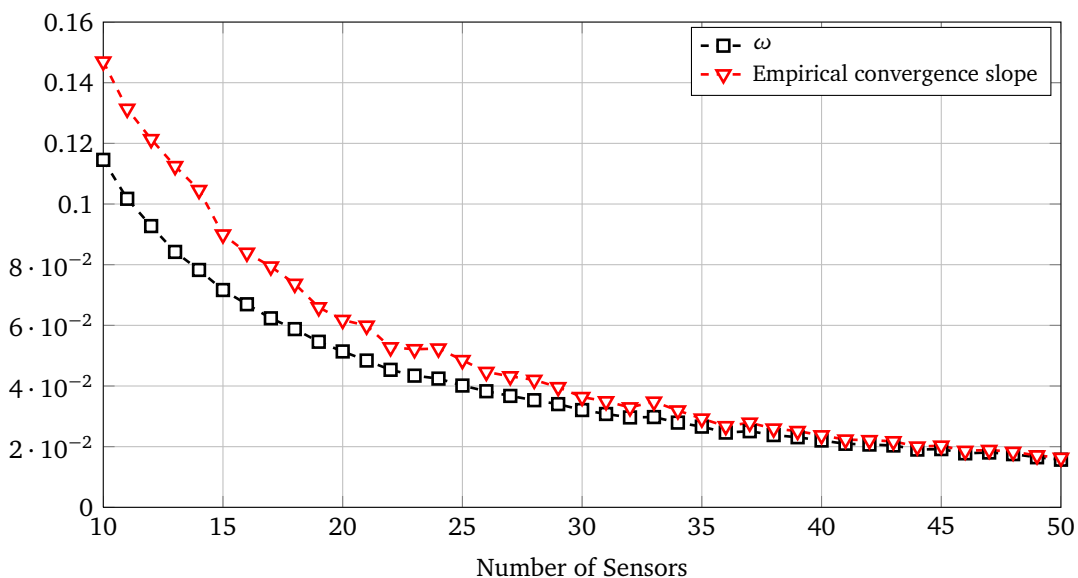
Figure 3.2: Empirical convergence slope of the BWGossip and associated lower bound \omega .
