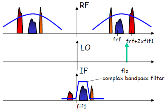
Fig 37. Signal processing operations in a low-IF receiver
