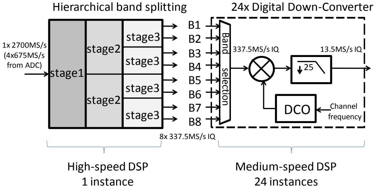
Fig 19. Proposed DCS architecture
