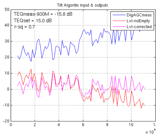
Fig 28. Simulation of the tilt control loop with random channel amplitudes
