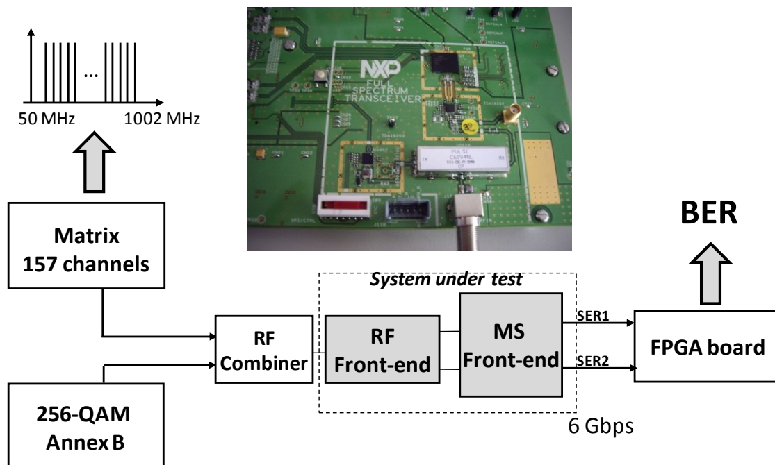
Fig 30. Full receiver board & system test bench
