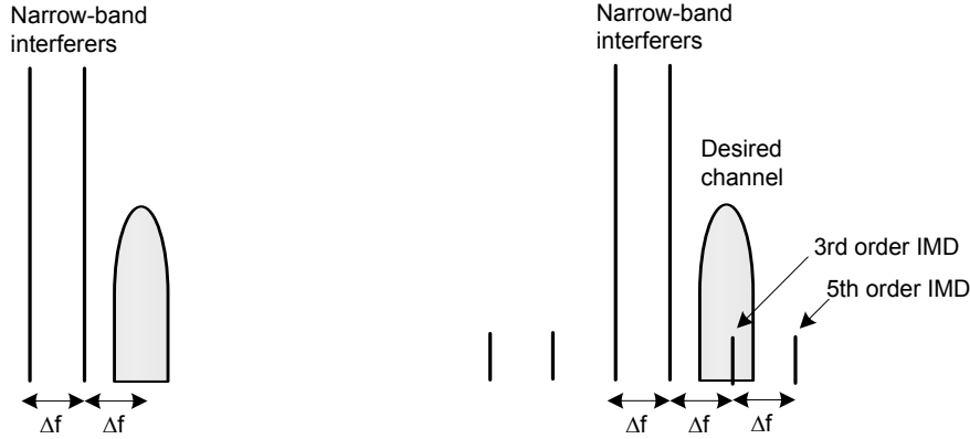
Fig 28. Third-order Intermodulation test – Input signal (left), RF Sampling ADC output signal (right)
