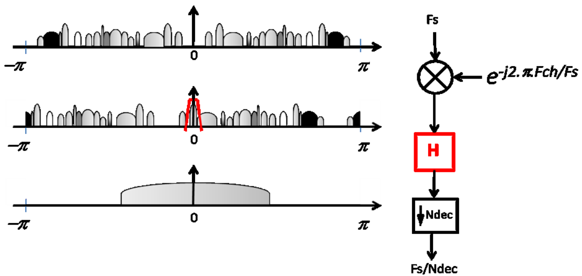
Fig 56. Signal Processing involved in Digital Channel Selection
