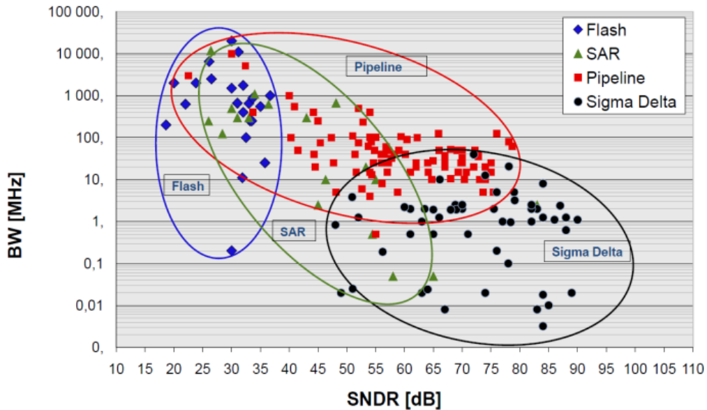
Fig 30. ADC state-of-the-art in a SNDR-BW plane
