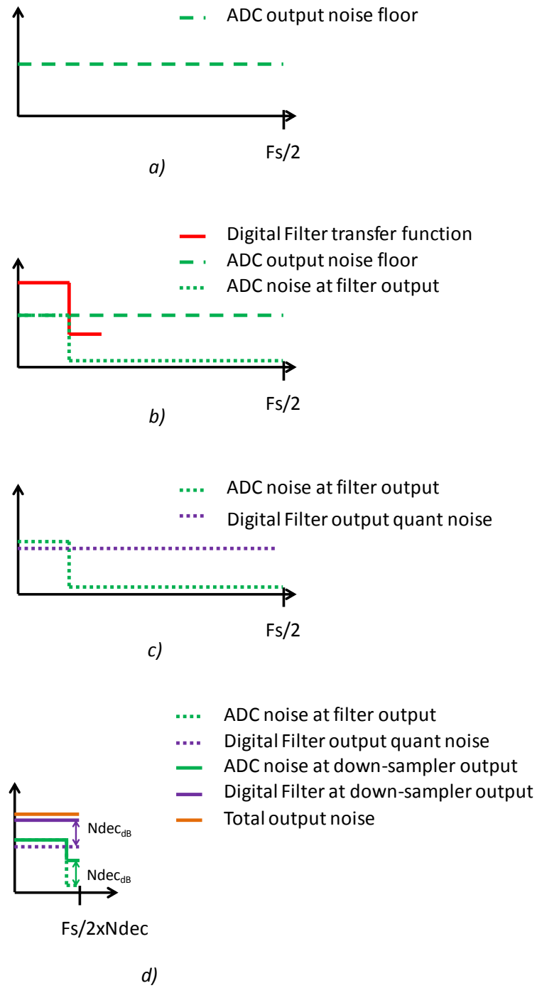
Fig 59. Impact of DSP filters and down-sampling on ADC and DSP noises
