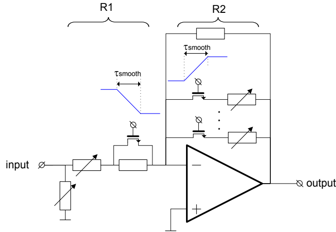
Fig 3. Pseudo-continuous LNA principle diagram
