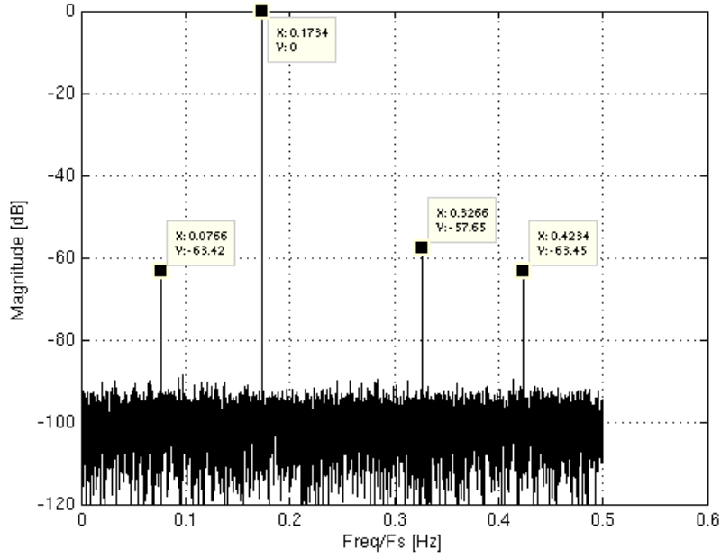
Fig 40. Gain spurs in an ADC with an interleaving factor of four, input=sine wave at 0.1734 \times f_s , \sigma_{\text{gain}} = 0.5 \times 10^{-3}
