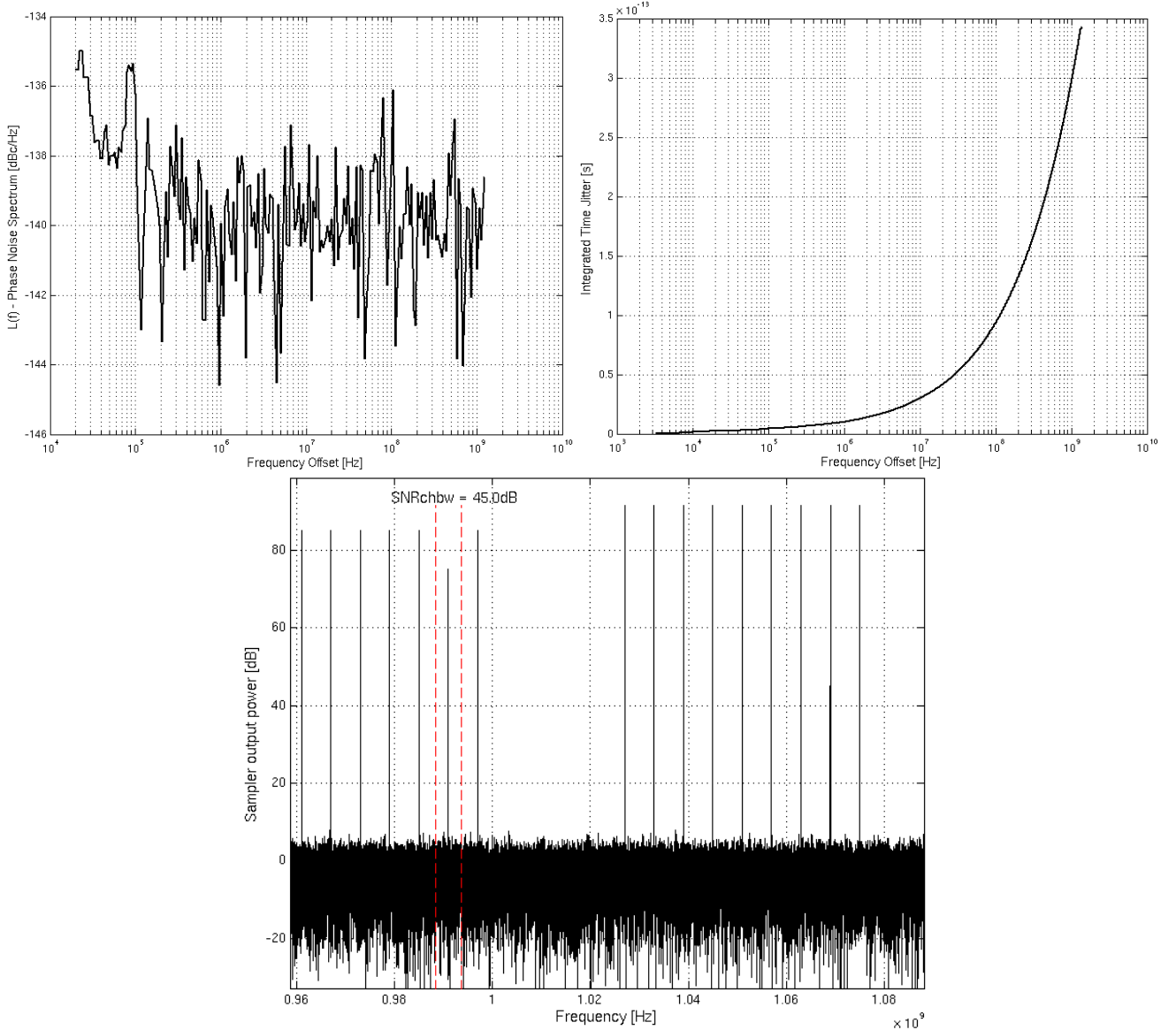
Fig 22. Simulation of distant phase noise. Top left: PLL phase noise density. Top right: PLL integrated time jitter. Bottom: sampler output spectrum with test condition TP2
