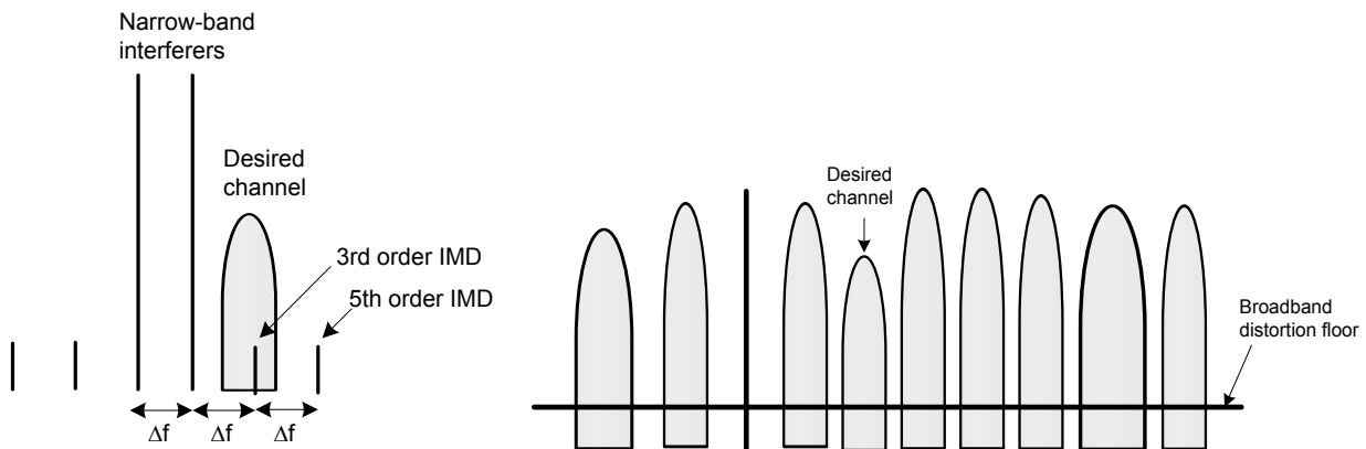
Fig 6. Intermodulation test (left), broadband non-linearity test (right)
