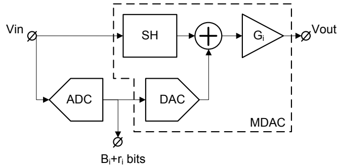
Fig 20. Pipeline sub-stage principle
