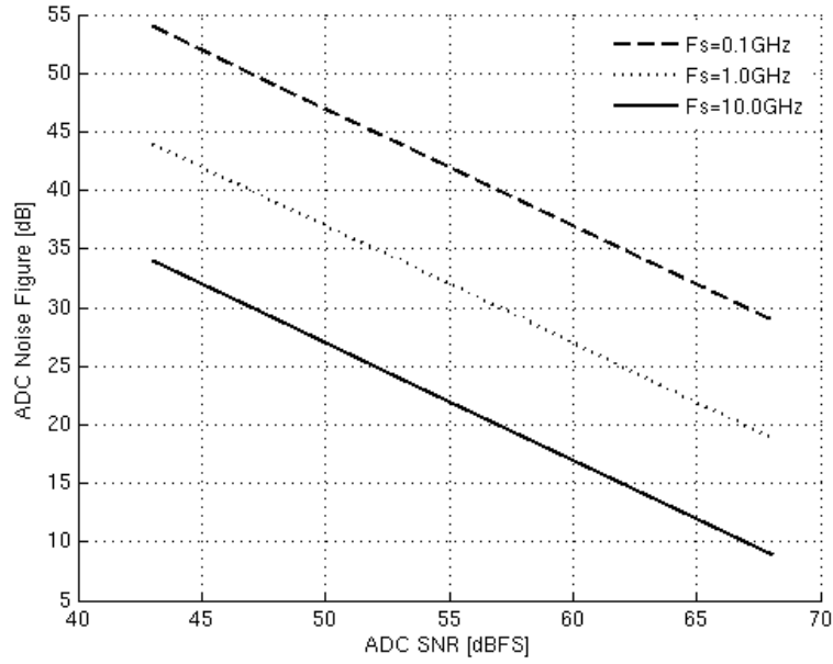
Fig 22. ADC noise figure for different SNR and sampling rates
