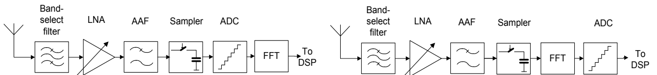
Fig 42. Move from DSP-based FFT (right) to analog-DT-based FFT (left)
