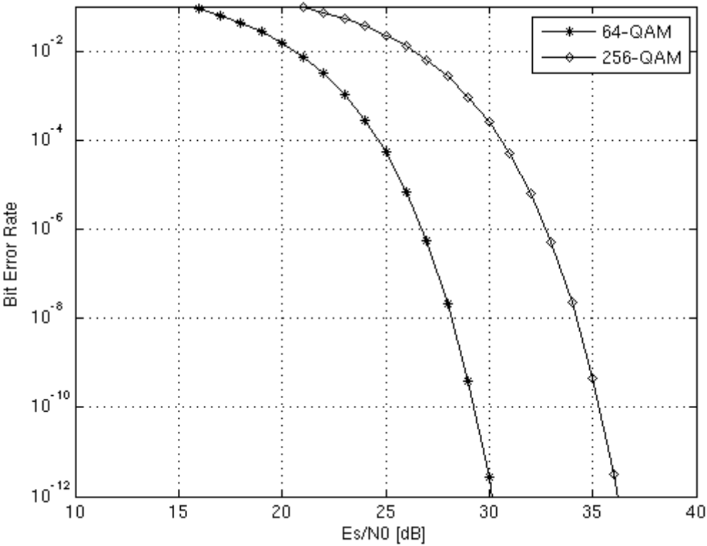
Fig 6. BER as a function of Signal-to-Noise Ratio
