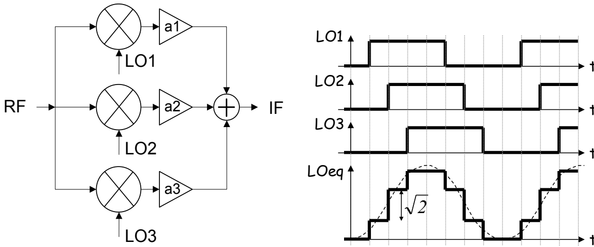
Fig 9. Harmonic-reject mixer
