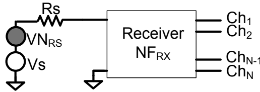
Fig 7. Full receiver and its equivalent Noise Figure
