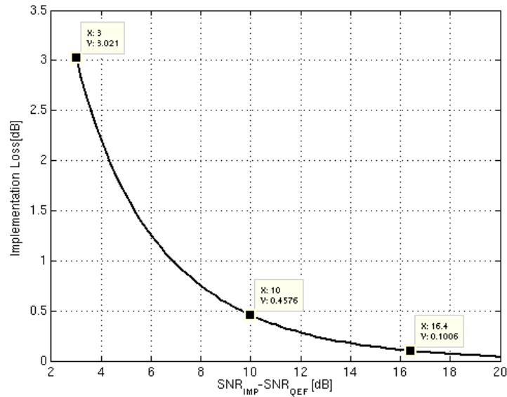
Fig 10. Implementation Loss against delta SNR
