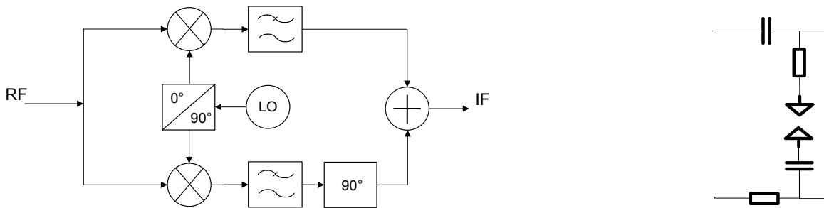
Fig 4. Hartley mixer structure (left), example of 90^\circ phase shift realization (right)
