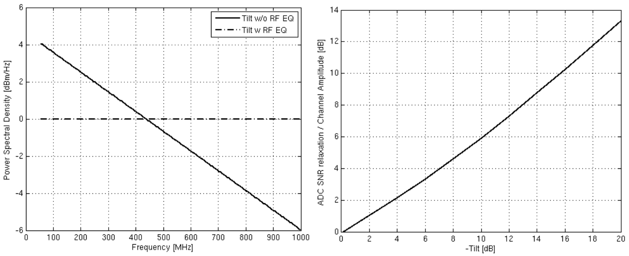
Fig 13. Channels amplitude w/wo RF tilt equalizer (left, -10dB tilt), ADC SNR relaxation with an RF tilt equalizer (right)
