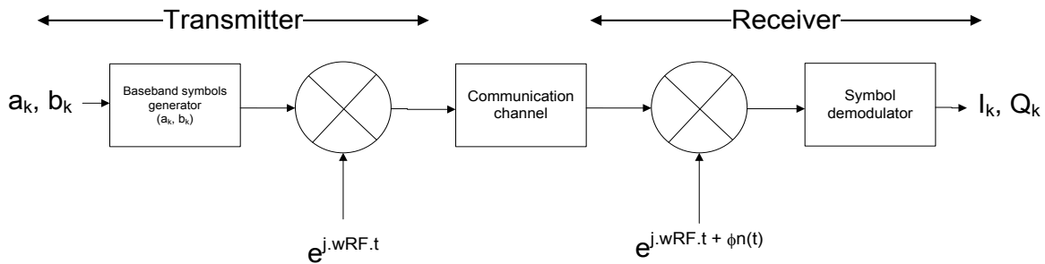
Fig 50. Communication system with phase noise in the receiver
