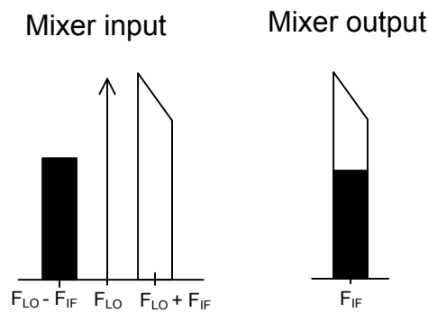
Fig 3. Image frequency in a down-conversion mixer
