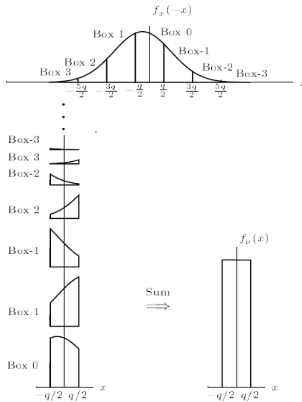
Fig 14. Construction of the PDF of quantization noise
