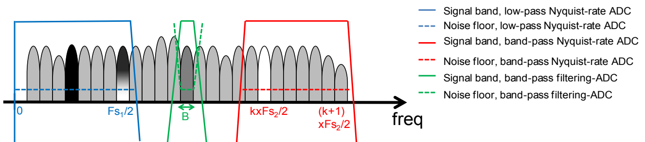
Fig 45. Direct-digitization receivers signal bands and noise floor
