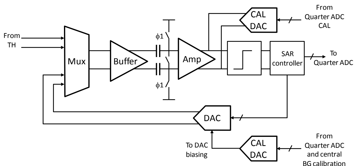
Fig 17. SAR ADC architecture and interface with TH
