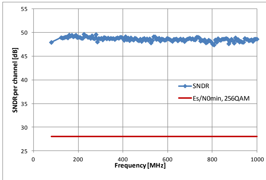
Fig 29. MSFE broadband SNDR performance
