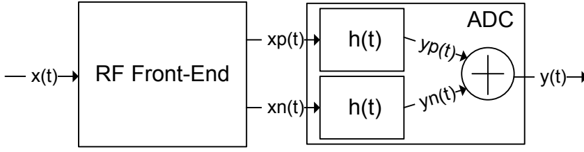
Fig 33. RF Front-End to Sample-And-Hold interface
