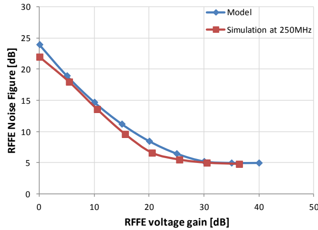
Fig 11. RFFE assumed NF versus voltage gain
