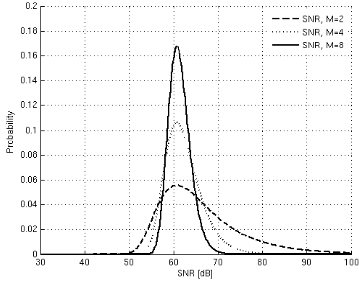
Fig 45. Statistical simulation of SNR induced by offset mismatch in a two/four/eight-channel time-interleaved ADC
