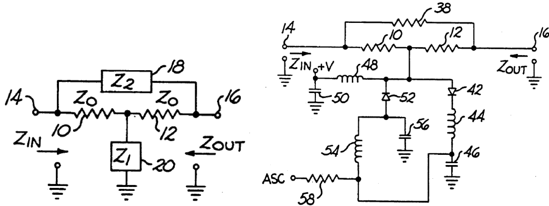
Fig 4. Tilt equalizer state-of-the-art for cable infrastructure
