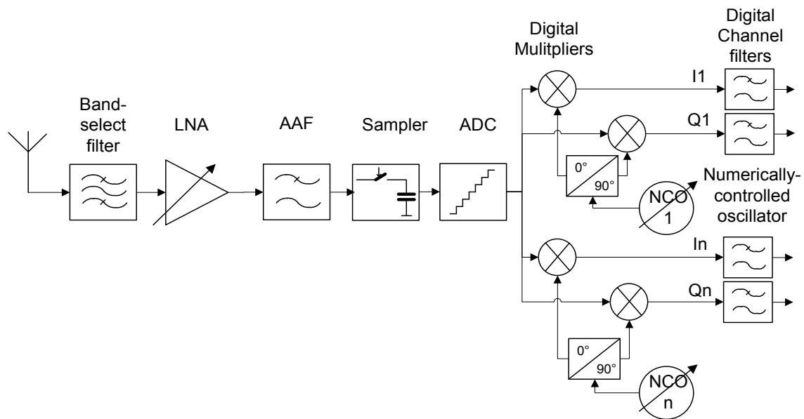
Fig 47. Direct digitization receiver based on Nyquist ADC
