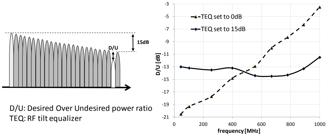
Fig 33. Left: cable input signal containing 15 dB tilt. Right: minimum D/U over frequency, without and with tilt equalizer (BER < 5 \times 10^{-5} )
