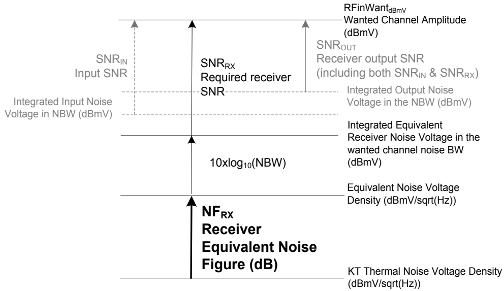
Fig 8. Required Equivalent Noise Figure level diagram
