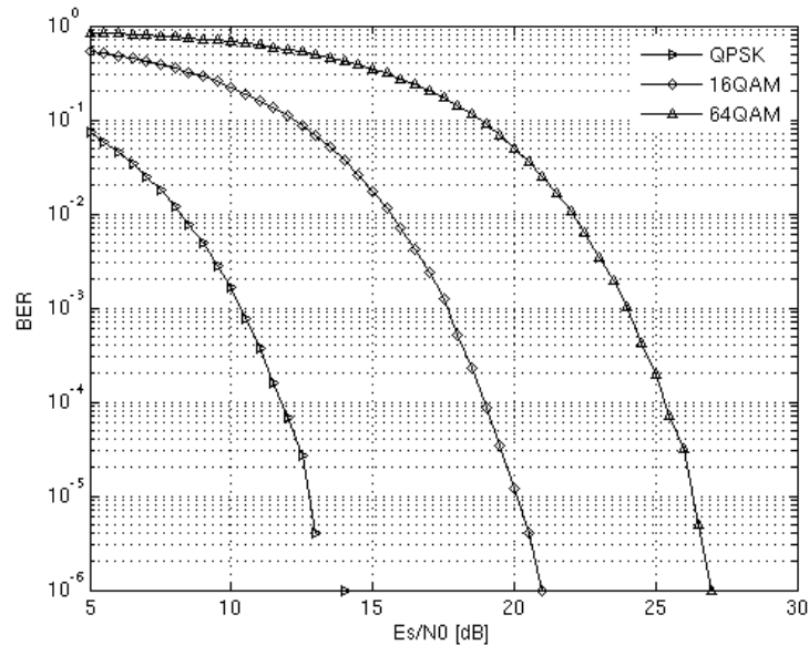
Fig 4. BER versus E_s/N_0 for several QAM modulations
