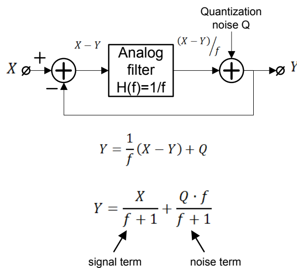
Fig 25. Delta-sigma ADC principle
