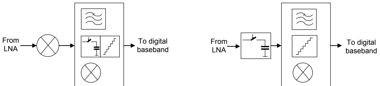
Fig 1. Left: continuous-time receiver (CTRX), right: discrete-time receiver (DTRX)
