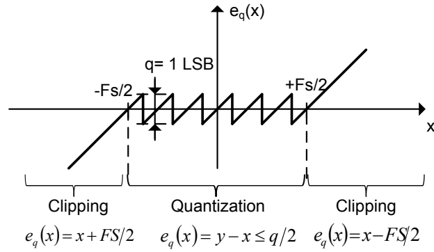
Fig 16. Ideal quantizer errors
