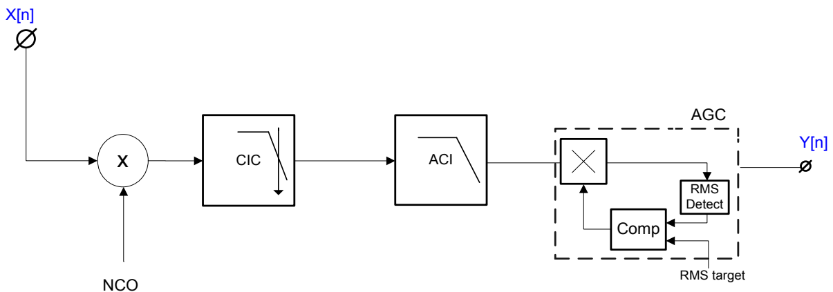
Fig 24. Digital Down-Converter
