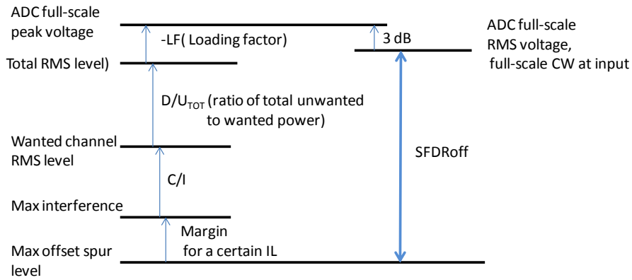
Fig 38. Specification for offset mismatch caused SFDR
