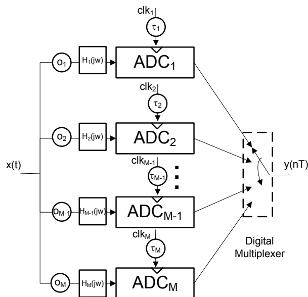
Fig 28. Time-interleaved ADC with channel mismatches
