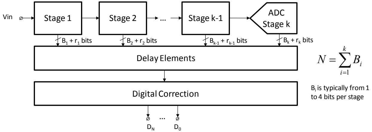
Fig 19. Sub-ranging / Multi-step / Pipeline ADCs principle architecture
