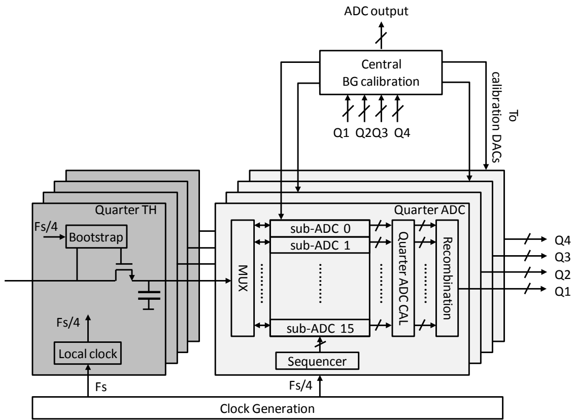
Fig 16. ADC block diagram
