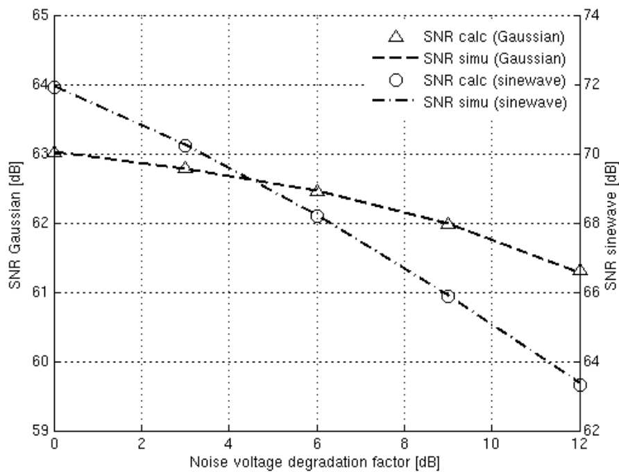
Fig 20. Calculated & simulated Signal-to-Noise versus large-signal noise degradation (left: sine wave; right: Gaussian)
