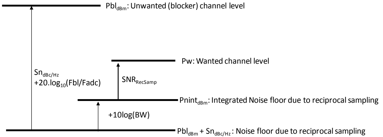
Fig 53. Reciprocal Sampling – Link between phase noise density and SNR
