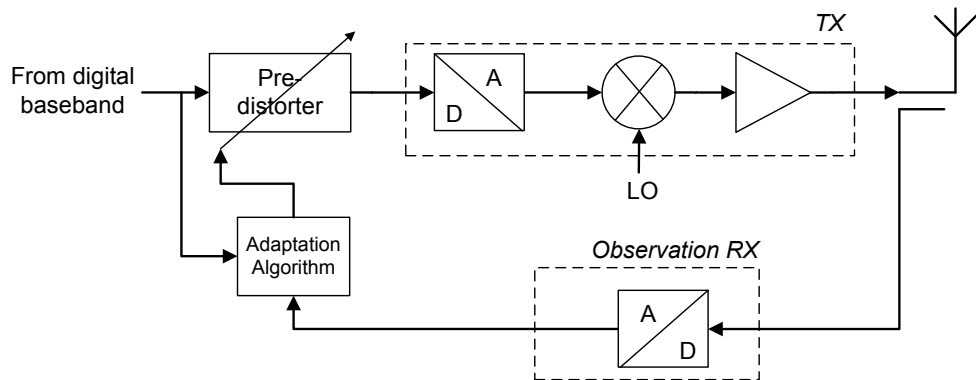
Fig 1. Use of a observation RX in a Digital pre-Distortion loop for PA linearization
