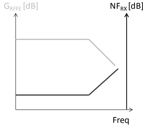
Fig 26. Cascaded Receiver NF, with lowpass RFFE gain, for ADC dominating the RX noise
