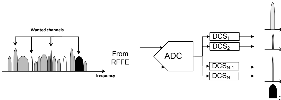
Fig 55. Digital Channel Selection
