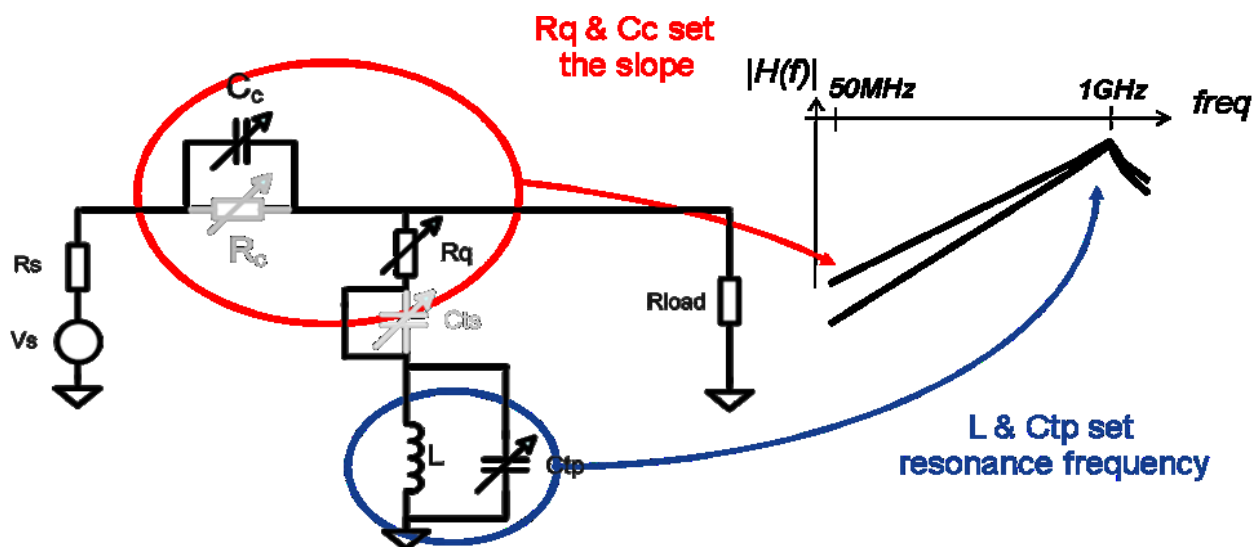
Fig 6. Tilt equalizer configured as a parallel resonator
