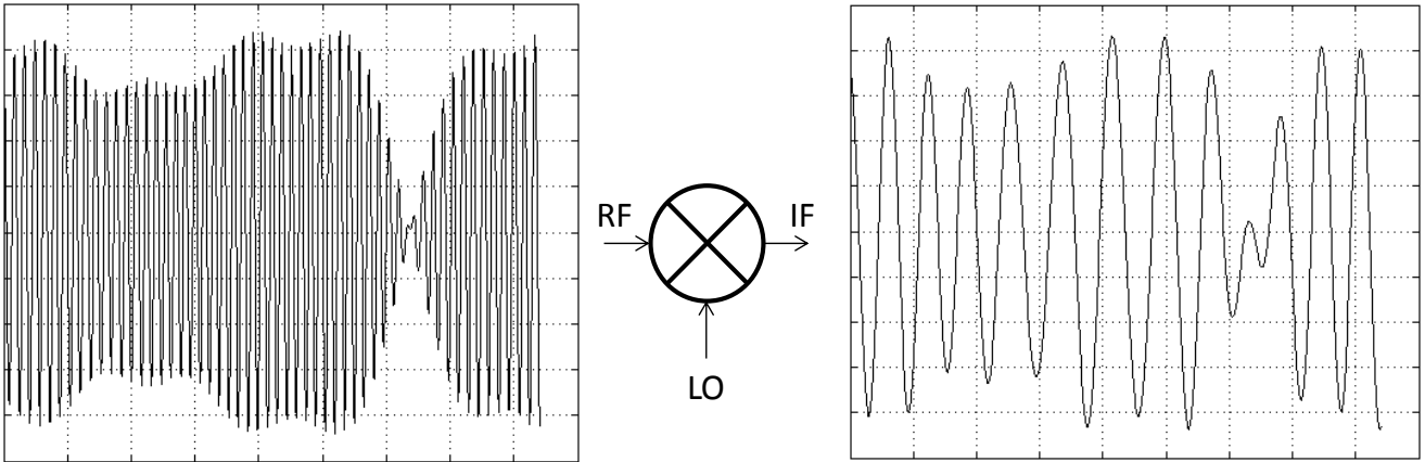
Fig 2. Frequency translation from RF to IF using a continuous-time mixer
