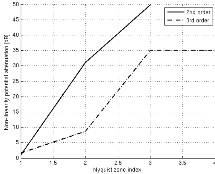
Fig 32. Non-linear distortion potential improvement factor, depending on the sampling strategy
