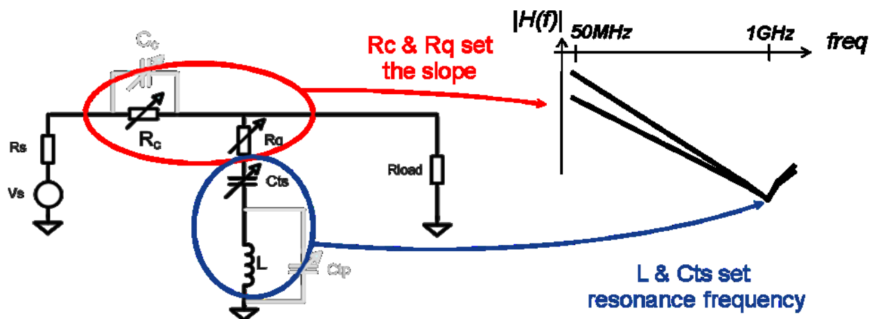
Fig 7. Tilt equalizer configured as a series resonator
