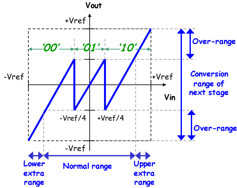
Fig 21. Pipeline ADCs conversion steps, without (left) and with (right) over-range
