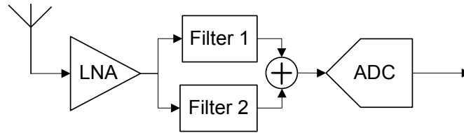
Fig 49. Multiband GNSS sub-sampling receiver front-end
