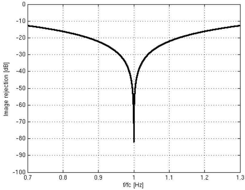
Fig 17. Narrowband image rejection with 2 nd order sampling
