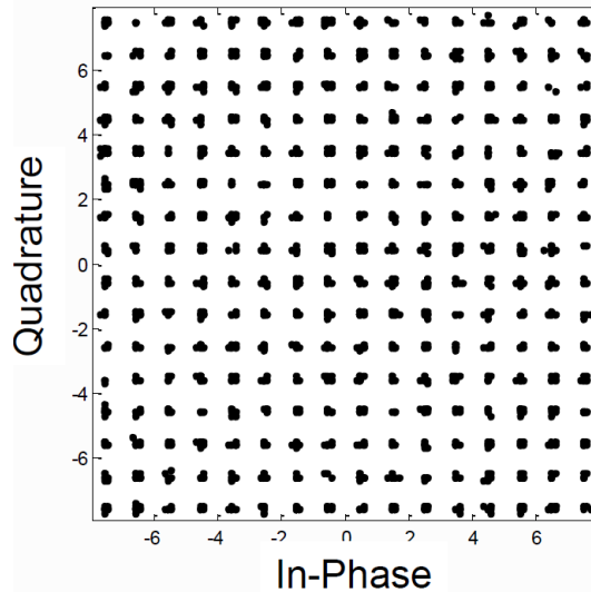
Fig 32. Received 256-QAM constellation captured inside the QAM demodulator, with 157 adjacent channel at +10 dBc
