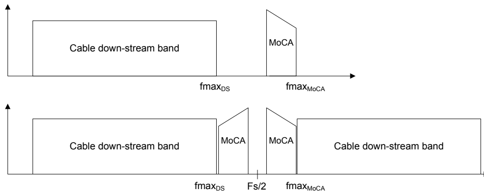
Fig 10. Aliasing of MoCA signals
