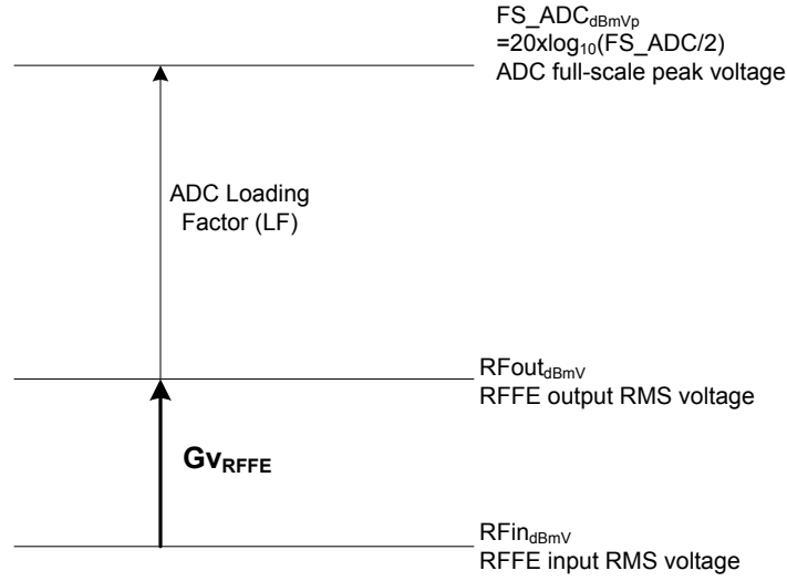
Fig 23. Level Diagram
