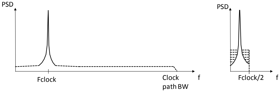
Fig 54. left: clock PSD, right: wideband clock phase noise PSD transferred to the sampled signal (including aliasing)
