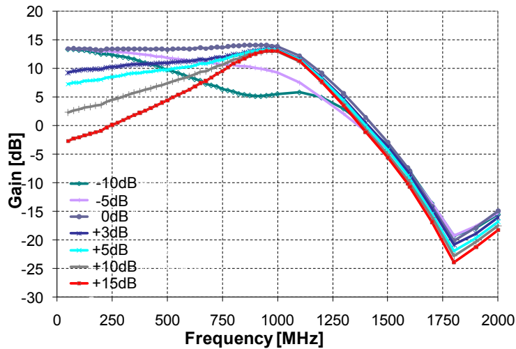
Fig 13. RFFE measured transfer functions for various TEQ settings
