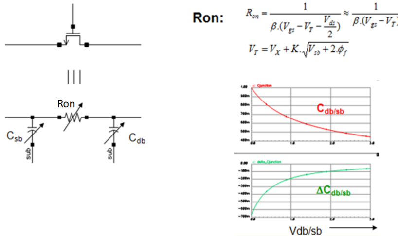
Fig 9. Non-linear R_{on} and junction capacitances in a MOS transistor in triode mode
