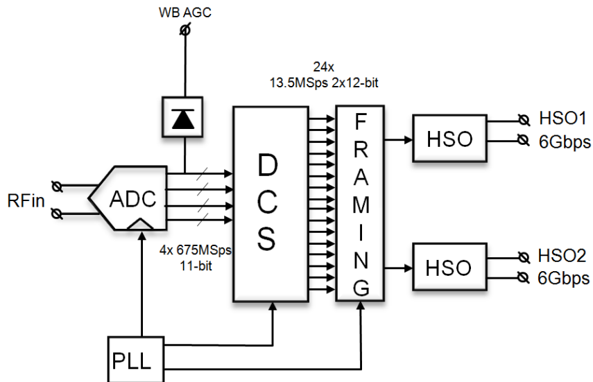
Fig 15. Mixed-signal front-end block diagram (down-stream path)
