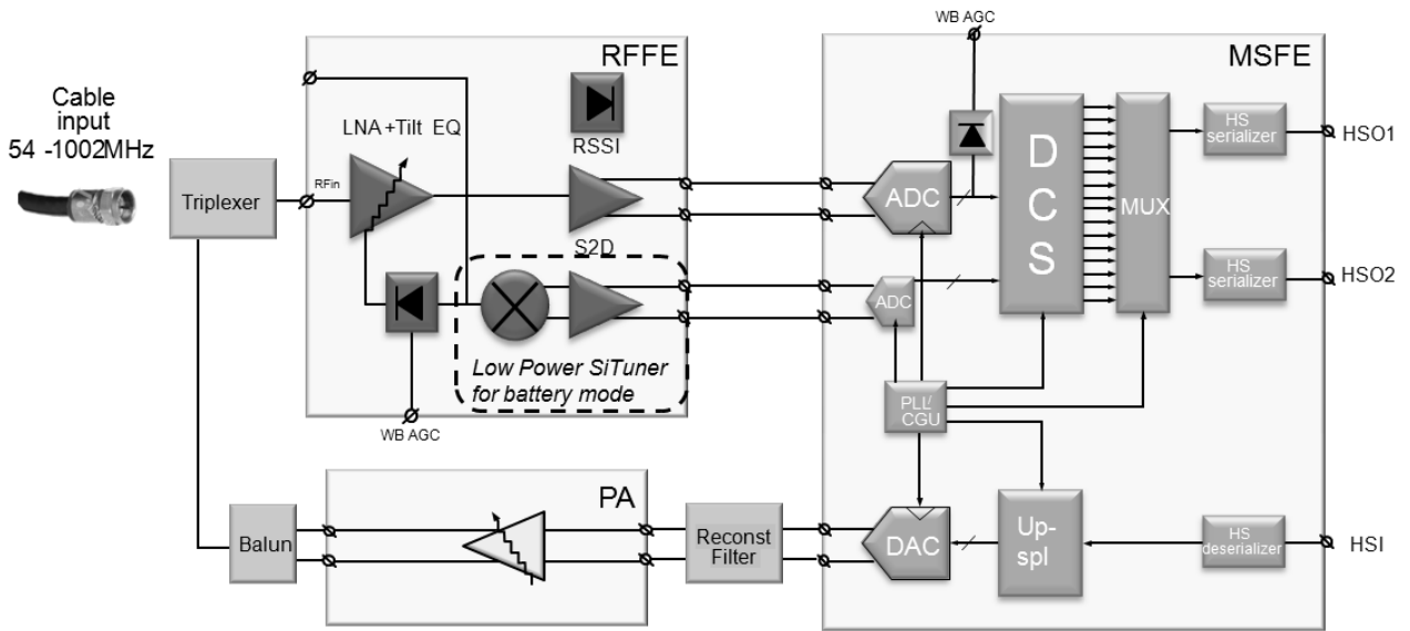
Fig 1. Cable multi-channel receiver system block diagram
