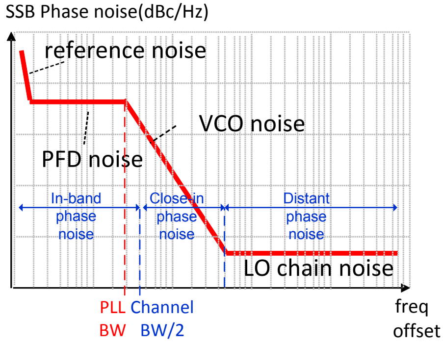
Fig 49. Typical clock phase noise profile
