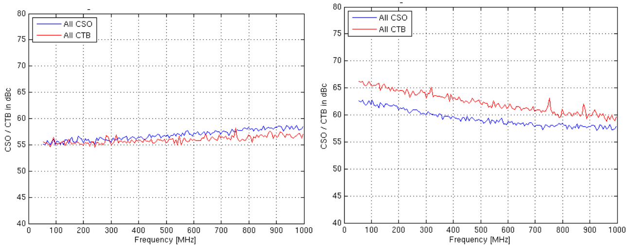
Fig 15. 2 nd and 3 rd order non-linear distortion with TP2, 158 tones, +15dBmV/tone
