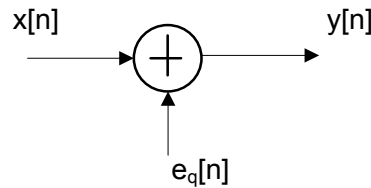
Fig 13. Additive noise model of a quantizer
