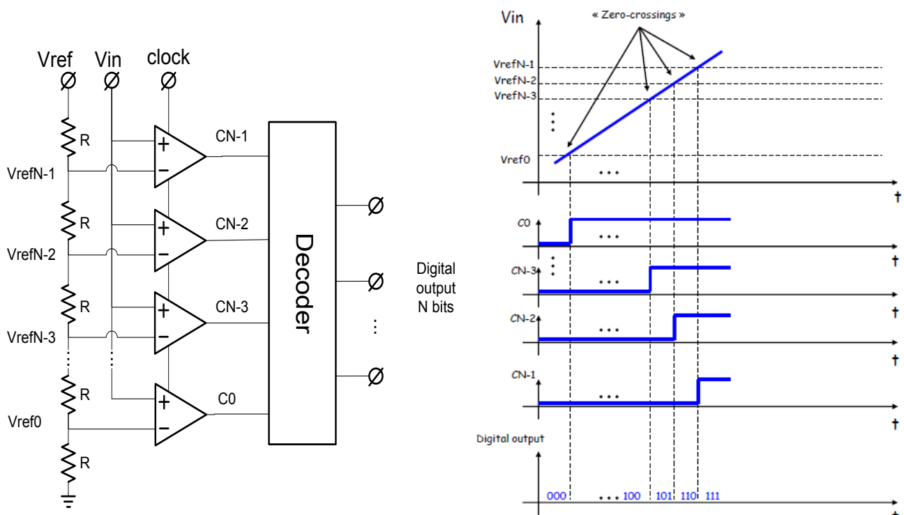
Fig 18. Flash ADC principle architecture
