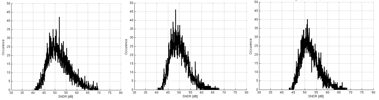
Fig 46. SNDR distribution for offset, gain & time-skew mismatches, four channels, 5000 trials
