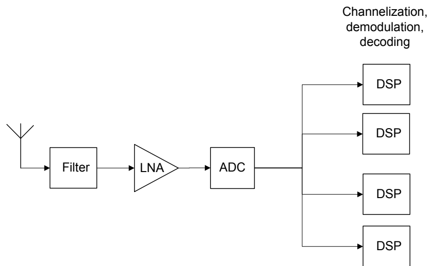
Fig 44. Multi-channel direct RF digitization receiver
