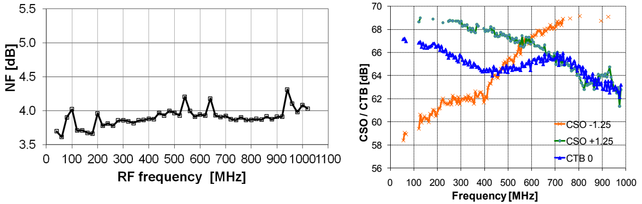
Fig 14. RFFE measured Noise Figure (left), and CSO/CTB (right)
