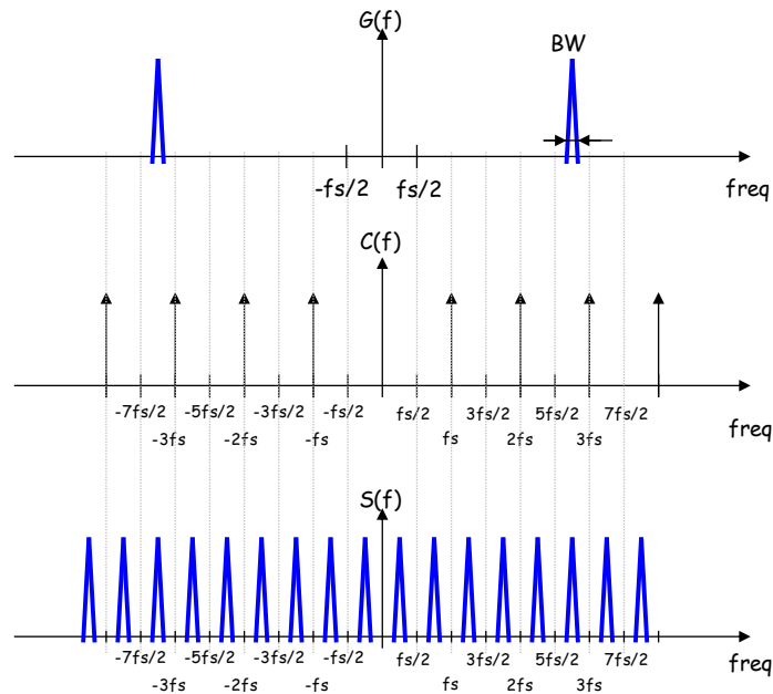
Fig 14. Bandpass sampling in the frequency domain
