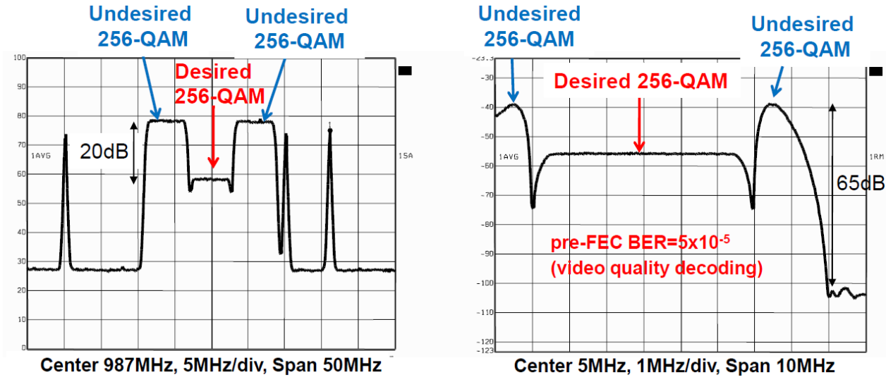
Fig 31. System test with 2 adjacent QAM channels (+20 dBc) and 157 CWs (0 dBc). Left: input signal, Right: output signal
