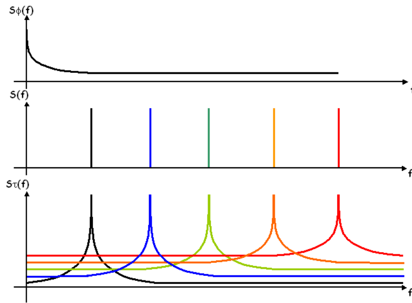
Fig 48. Clock phase noise convolved with multiple carriers input spectrum
