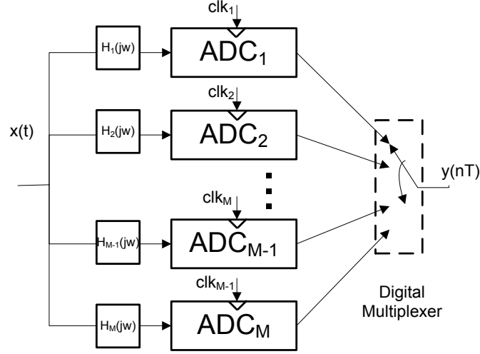
Fig 44. Time-interleaved ADC with transfer function mismatch
