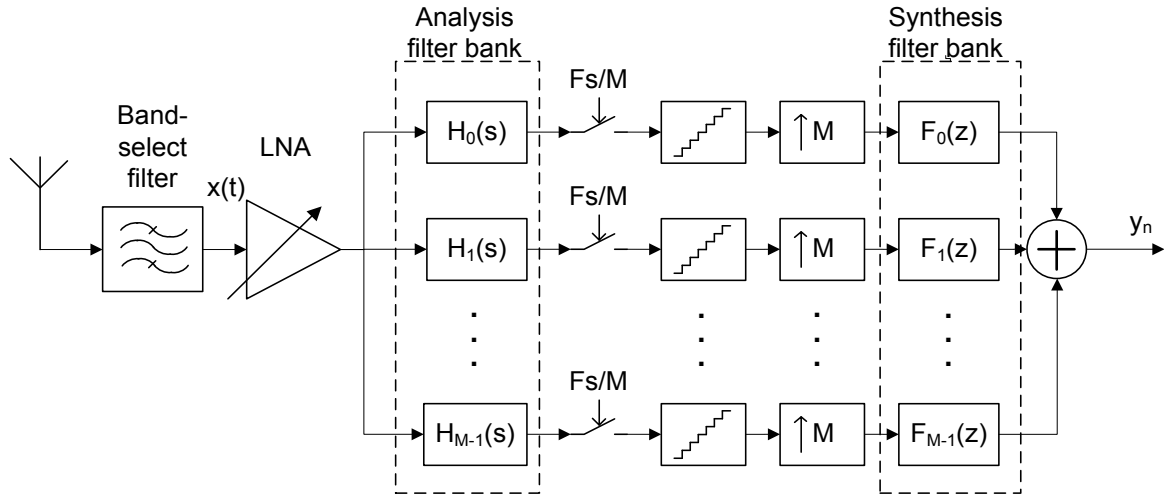
Fig 43. HFB receiver (left). Transfer functions of the analysis filter bank (right)
