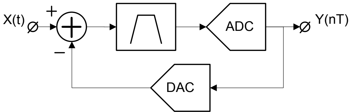
Fig 46. Direct digitization receiver based on bandpass filtering ADC
