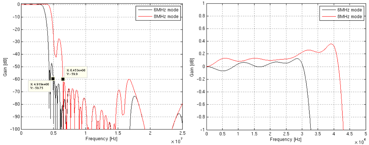
Fig 25. Digital Down-Converter frequency response
