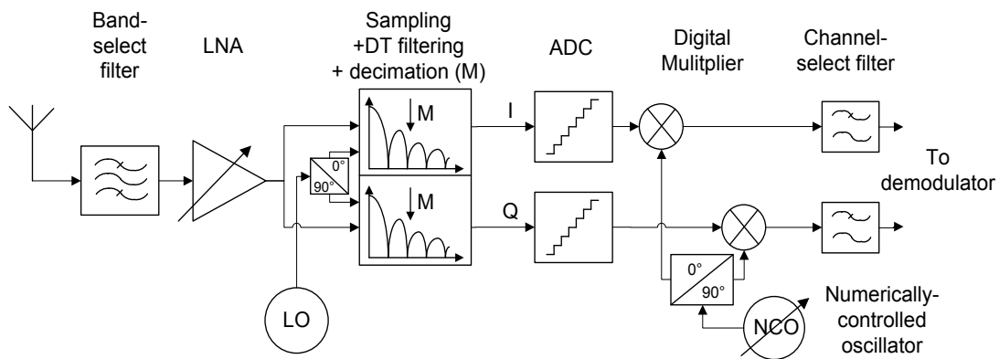
Fig 40. Discrete-time receiver principle diagram
