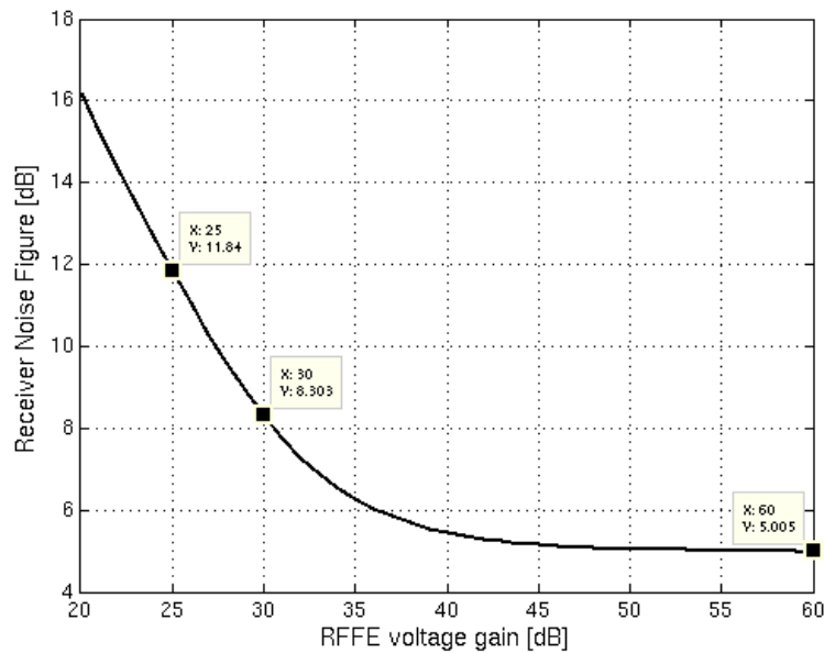
Fig 14. RFFE gain impact on Noise Figure
