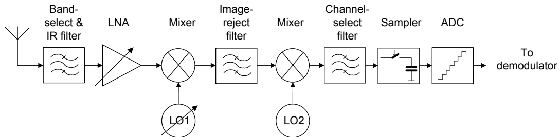
Fig 31. Dual Superheterodyne receiver
