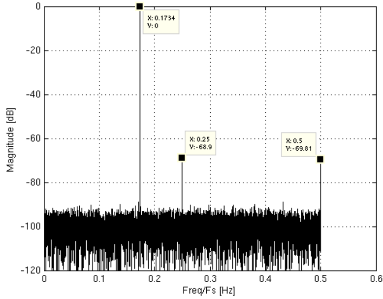
Fig 37. Offset spurs in an ADC with an interleaving factor of four, input=sine wave at 0.1734 \times F_s , \sigma_{\text{offset}} = 130 \mu\text{Vrms}
