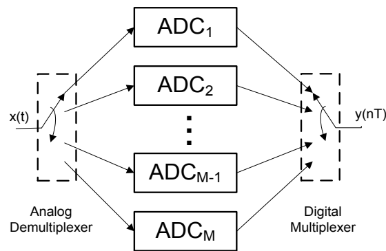
Fig 27. Time-interleaved ADC
