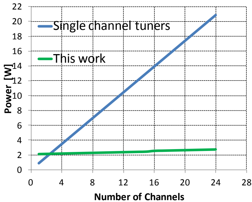
Fig 35. Power consumption against the number of received channels for Single channel tuners and this work
