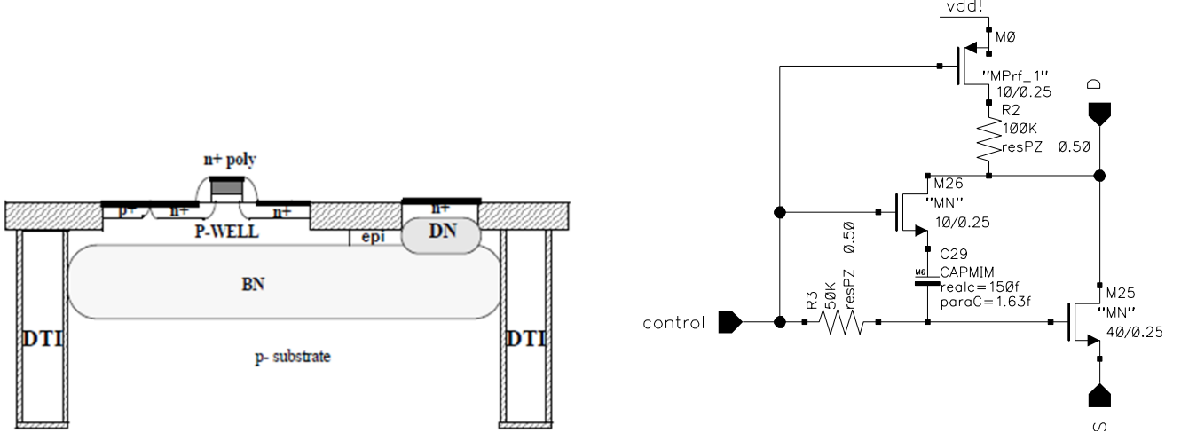
Fig 10. Improved linear RF MOS topology. Left: isolated cross-section, right: bootstrap and drain-biasing switch
