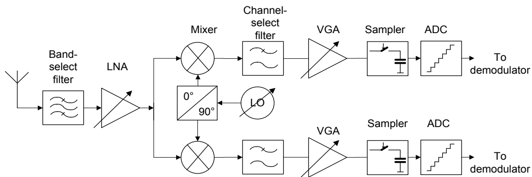
Fig 33. Homodyne receiver
