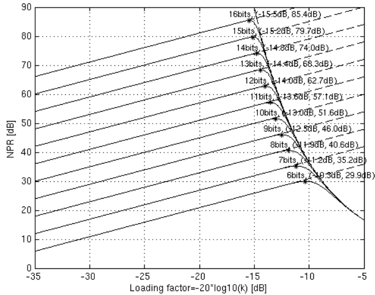
Fig 17. Noise Power Ratio & optimum loading factor for different ADC resolutions (Gaussian signal)
