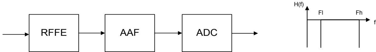
Fig 27. Simplified receiver model for non-linear distortion (left), AAF transfer function (right)
