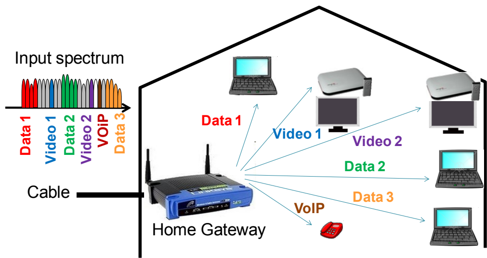
Fig 1. Centralized receiver architecture, articulated around a Home Gateway
