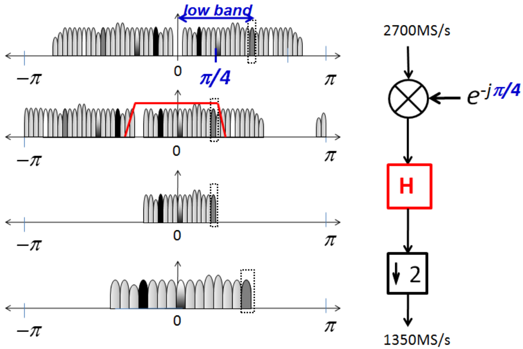
Fig 20. Hierarchical Band Splitting Stage 1: conversion of the input spectrum lower band
