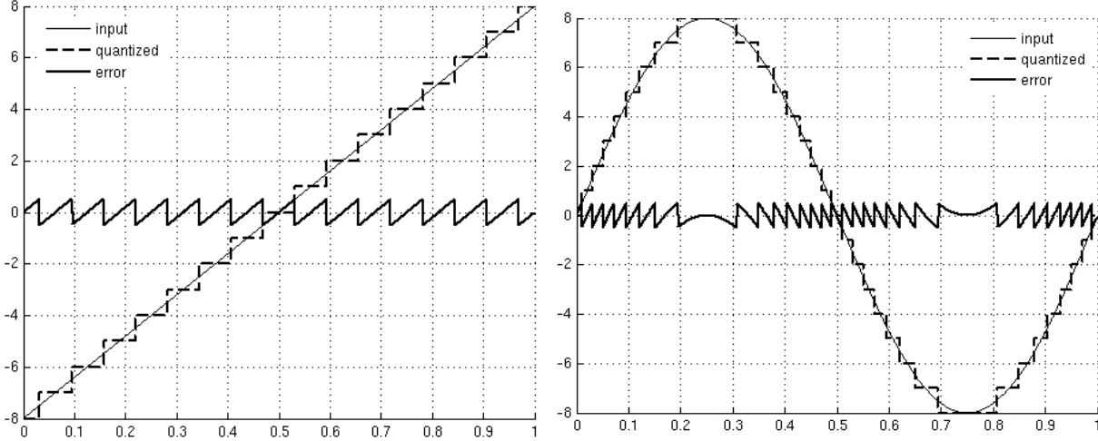
Fig 11. Quantization error with a ramp signal (left), and a sine wave signal (right)
