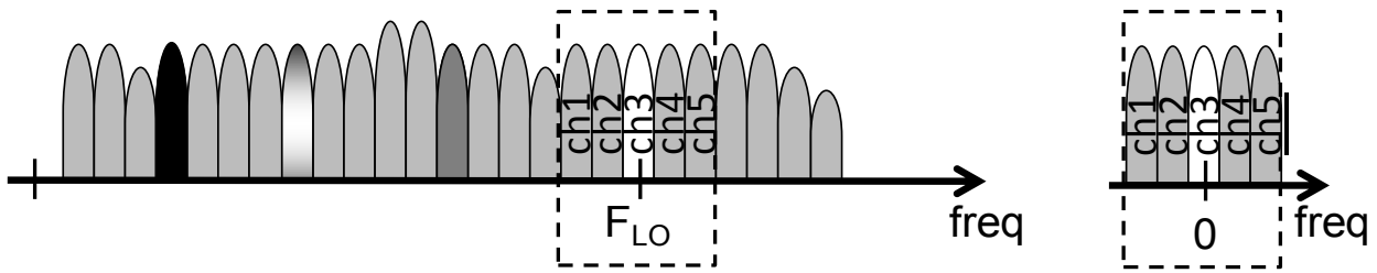
Fig 38. Multiple channels reception a complex low-IF / homodyne in a wideband RX. Left: RF signal. Right: IF signal
