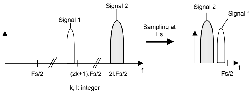
Fig 50. Multi-band GNSS RF spectrum (left). Spectrum after sampling (right)
