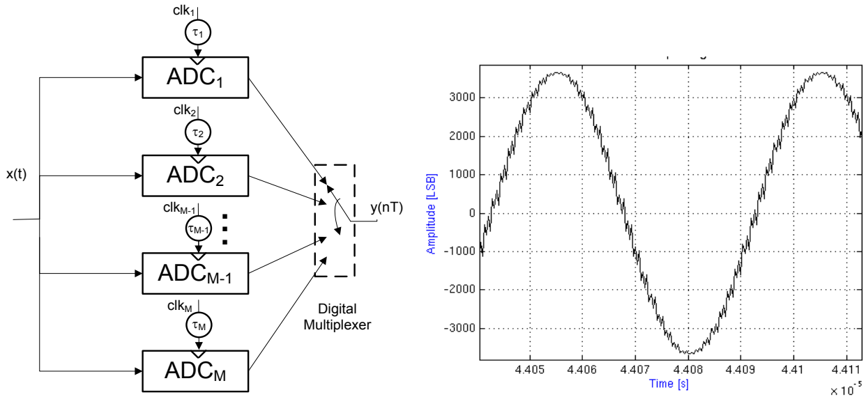
Fig 42. Time-interleaved ADC with time skew mismatch
