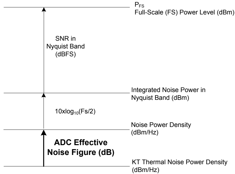
Fig 21. ADC noise figure calculation
