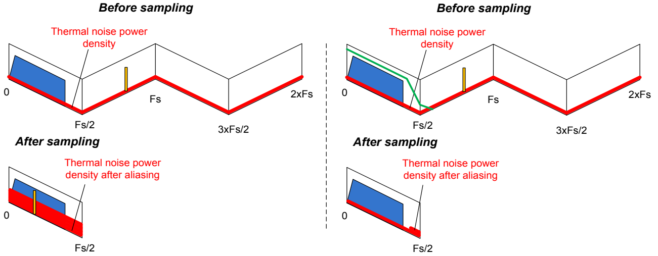
Fig 35. Aliasing of broadband noise and interferers. Left: without AAF, right: with AAF
