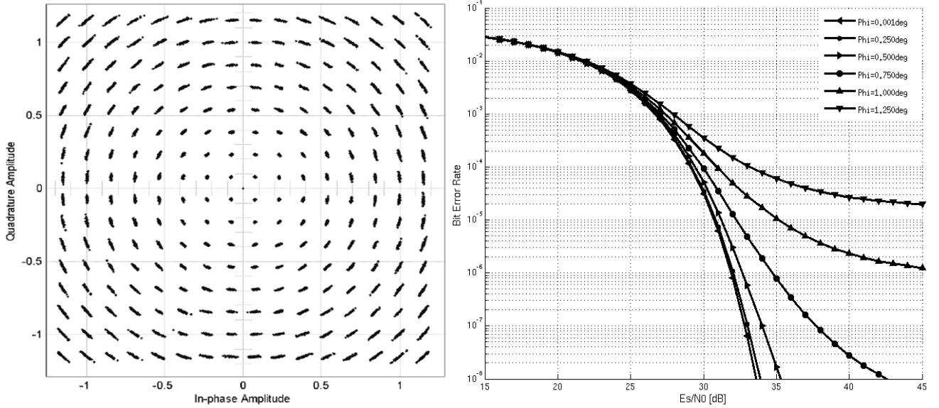
Fig 51. In-band phase noise effect on a complex modulation (left), and on BER (right)
