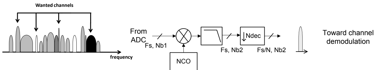
Fig 56. Signal Processing involved in Digital Channel Selection
