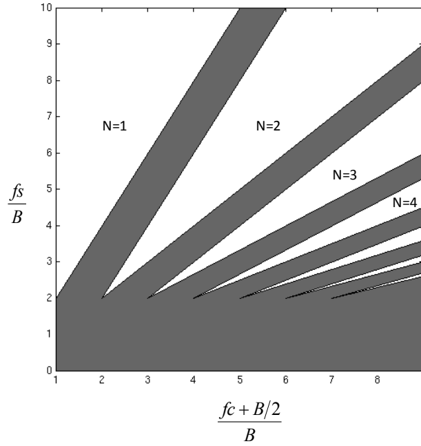
Fig 15. Valid sampling rates and band positions using bandpass sampling
