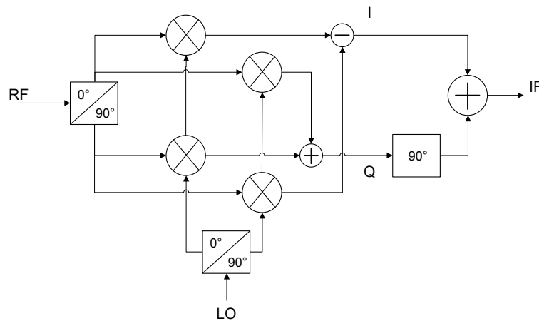
Fig 7. Double-quadrature mixer structure
