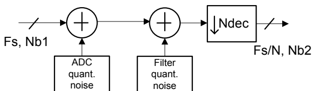
Fig 58. Noise model of a Digital Channel Selection unit
