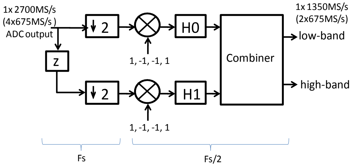
Fig 22. Hierarchical Band Splitting Stage 1
