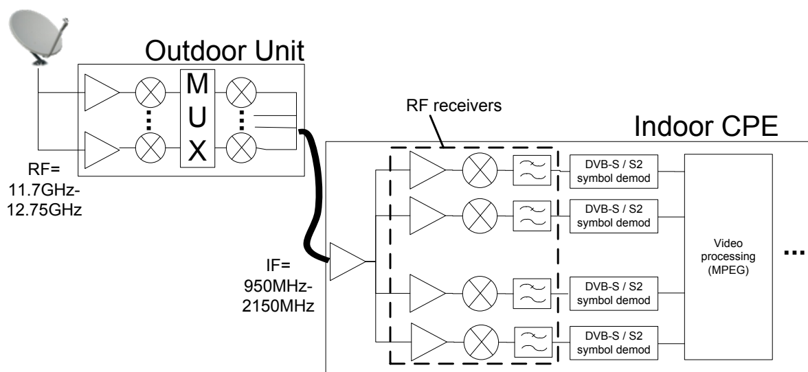
Fig 1. Satellite broadband multi-channel reception
