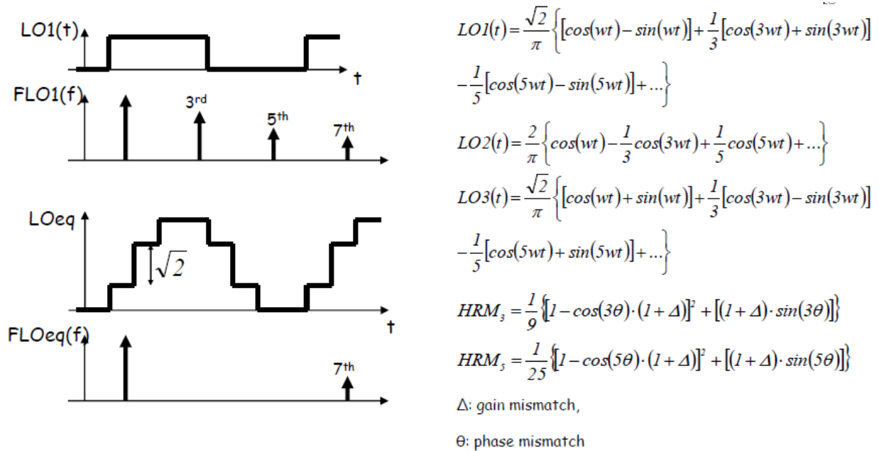
Fig 10. Harmonic-reject response
