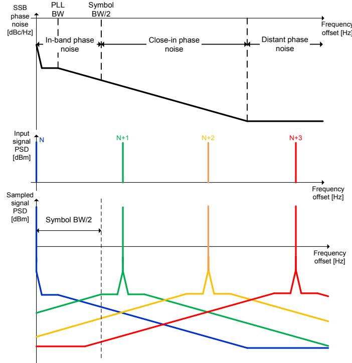
Fig 52. Reciprocal sampling process
