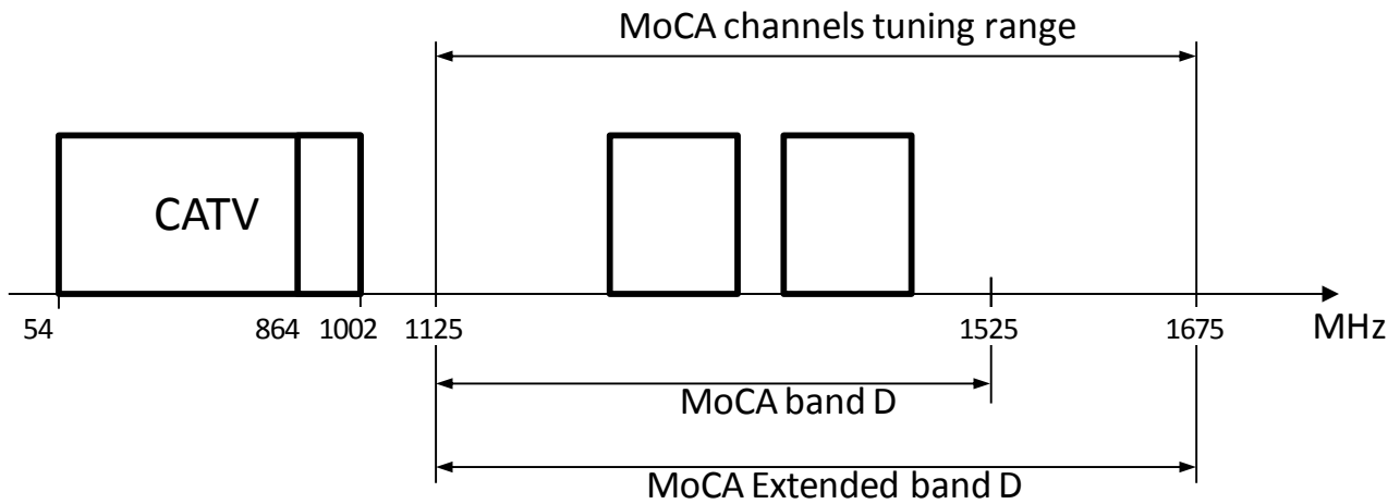
Fig 9. MoCA frequency plan
