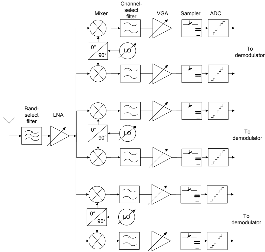
Fig 51. Sub-band splitting with analytic signals and down-conversion
