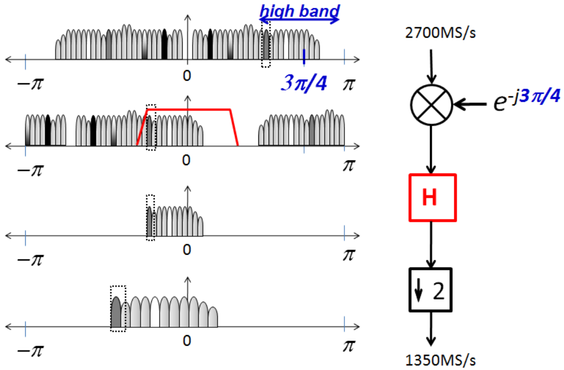
Fig 21. Hierarchical Band Splitting Stage 1: conversion of the input spectrum higher band
