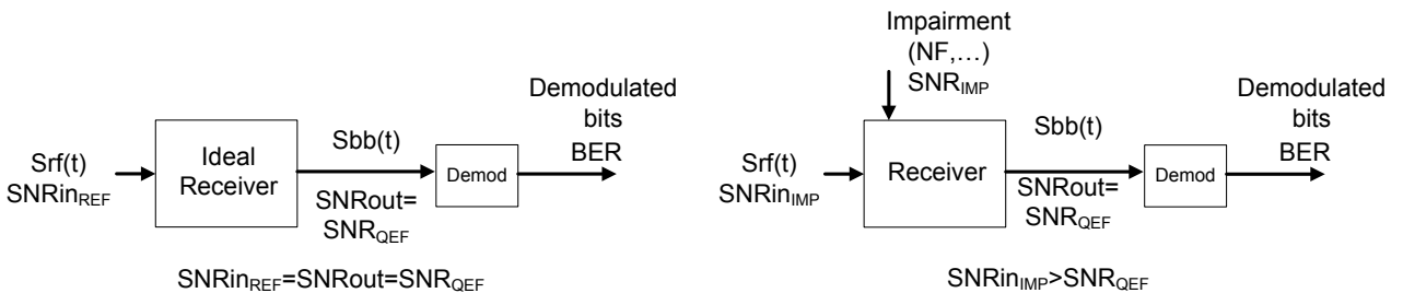
Fig 9. Receiver model for implementation loss characterization. Left: ideal receiver. Right: receiver with one impairment
