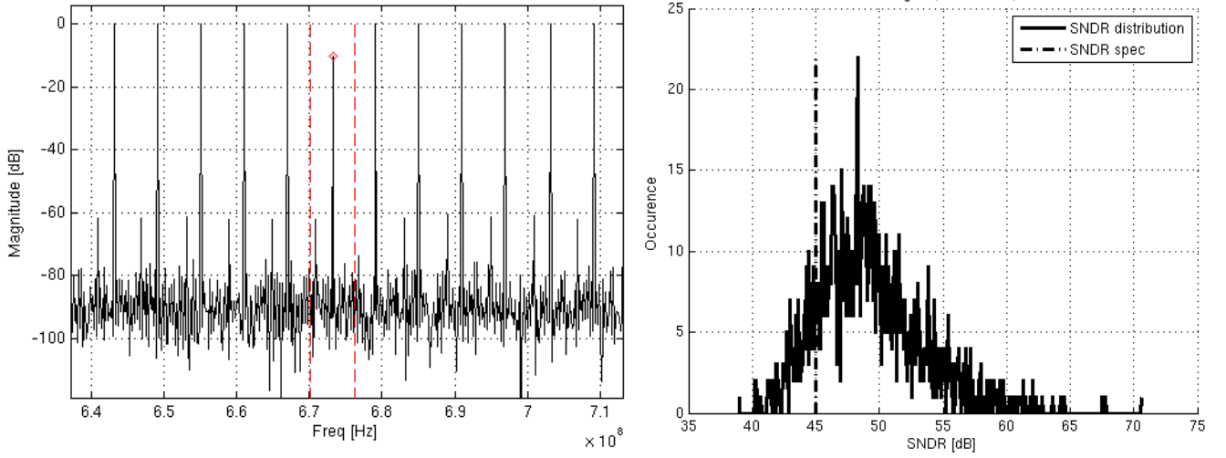
Fig 19. TD simulation with gain mismatch, \sigma_{\text{gain}}=0.9 \times 10^{-3} , Left: zoom on ADC output spectrum, right: per channel-SNDR distribution
