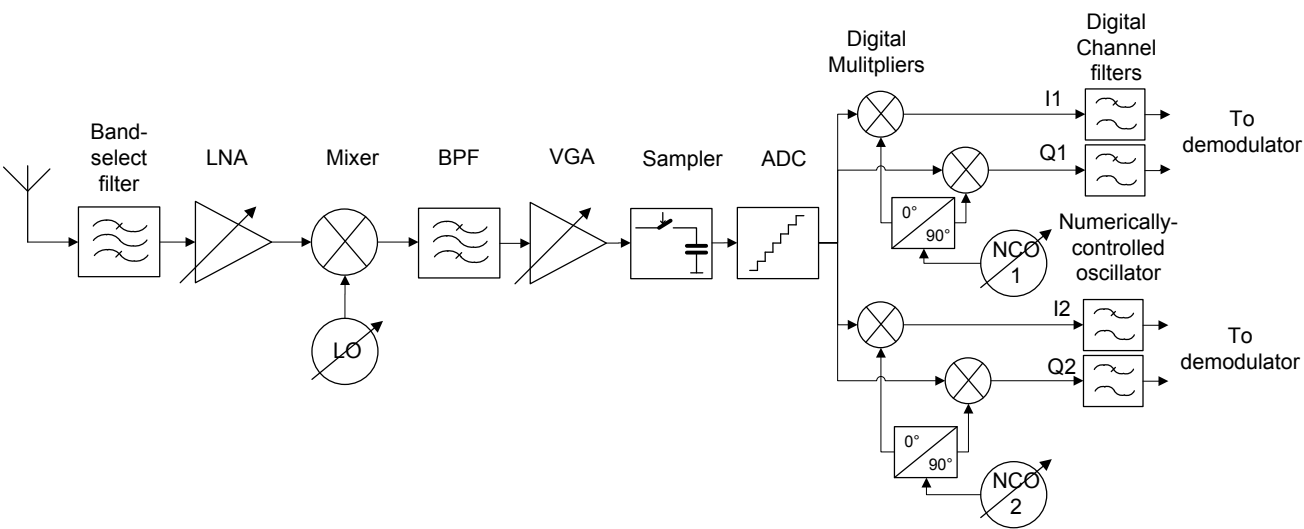
Fig 39. Digital-IF receiver
