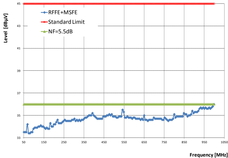
Fig 34. System sensitivity tests with 256-QAM, including RFFE, MSFE and QAM demodulator
