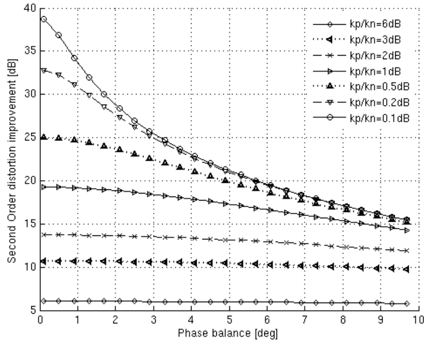
Fig 34. Gain and phase unbalance impact on 2 nd order non-linear distortion
