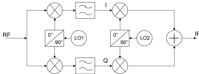
Fig 5. Weaver mixer structure
