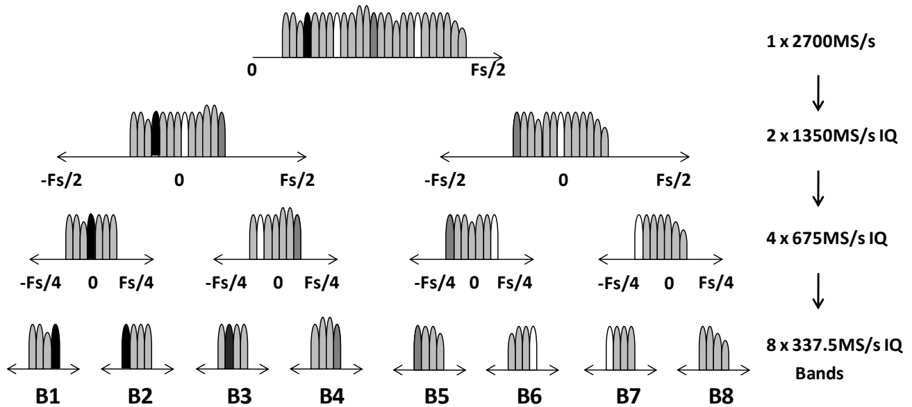
Fig 23. Hierarchical Band Splitting Stage 1, 2 and 3
