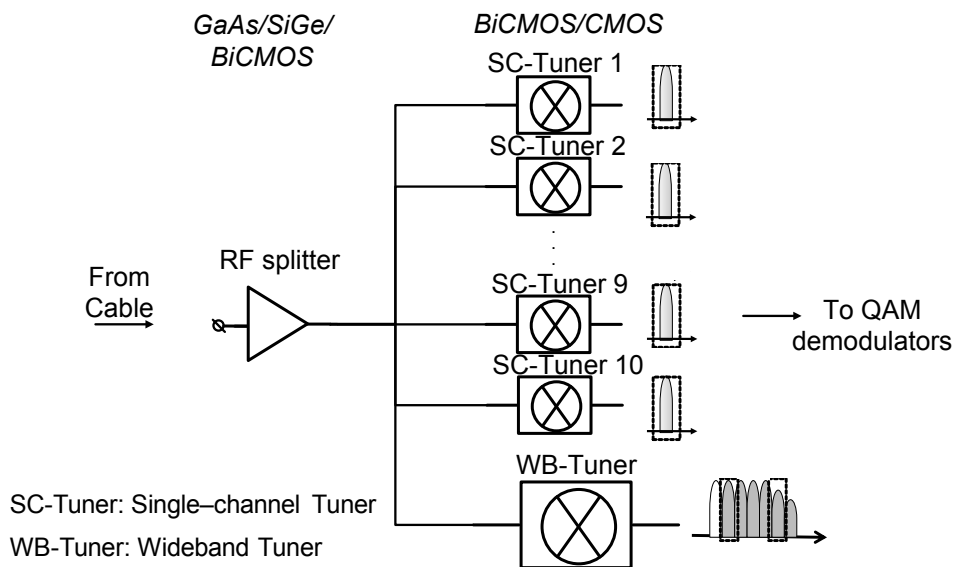
Fig 3. Silicon-Tuner-based Home Gateway front-end
