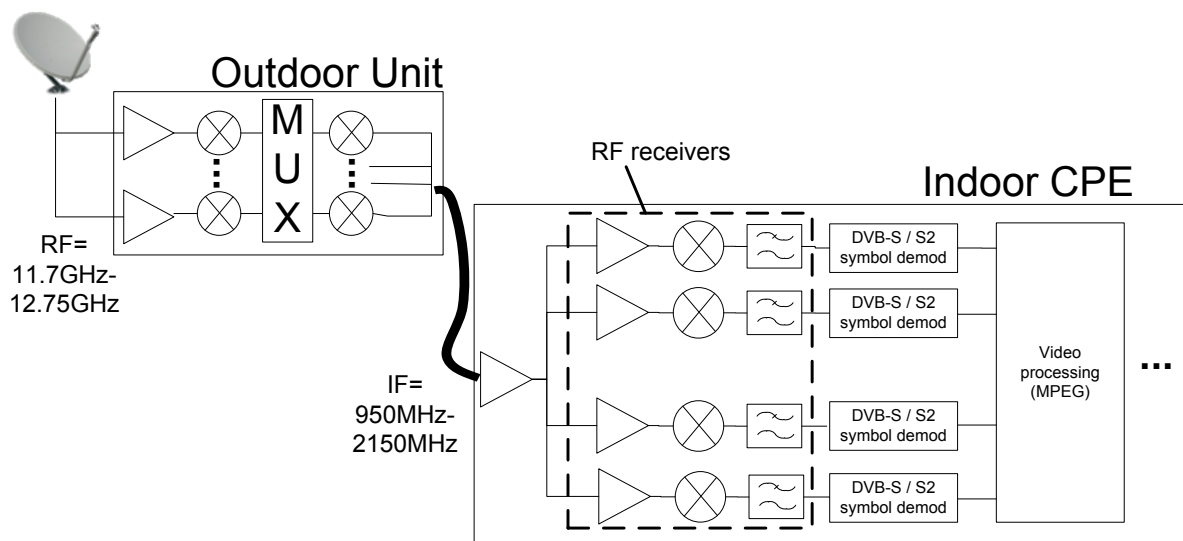
Fig 1. Satellite broadband multi-channel reception
