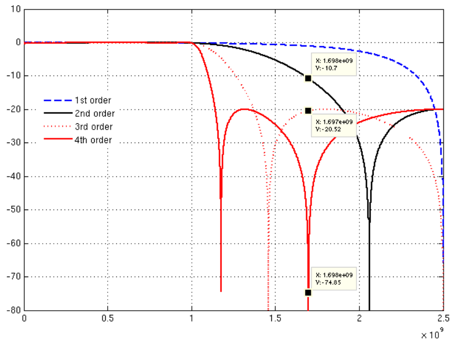
Fig 16. Transfer function modulus of Elliptic filter for several orders
