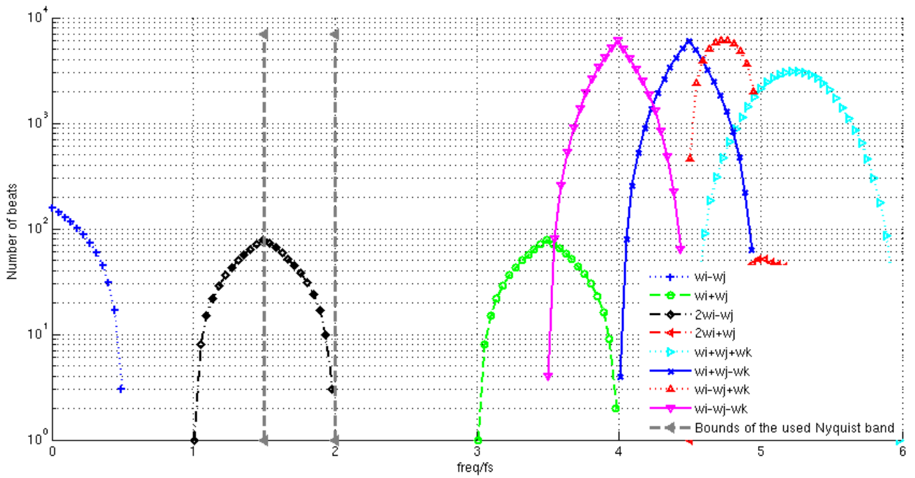
Fig 31. Number of beats across frequency, sampling in 4 th Nyquist band, 158 equally distant tones
