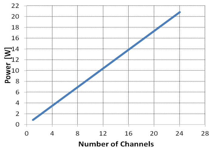
Fig 4. Power consumption of a Silicon-Tuner-based Home Gateway front-end
