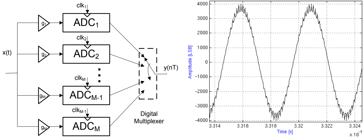
Fig 39. Time-interleaved ADC with gain mismatch (left), time-domain response with four channels & a sine wave input signal (right)
