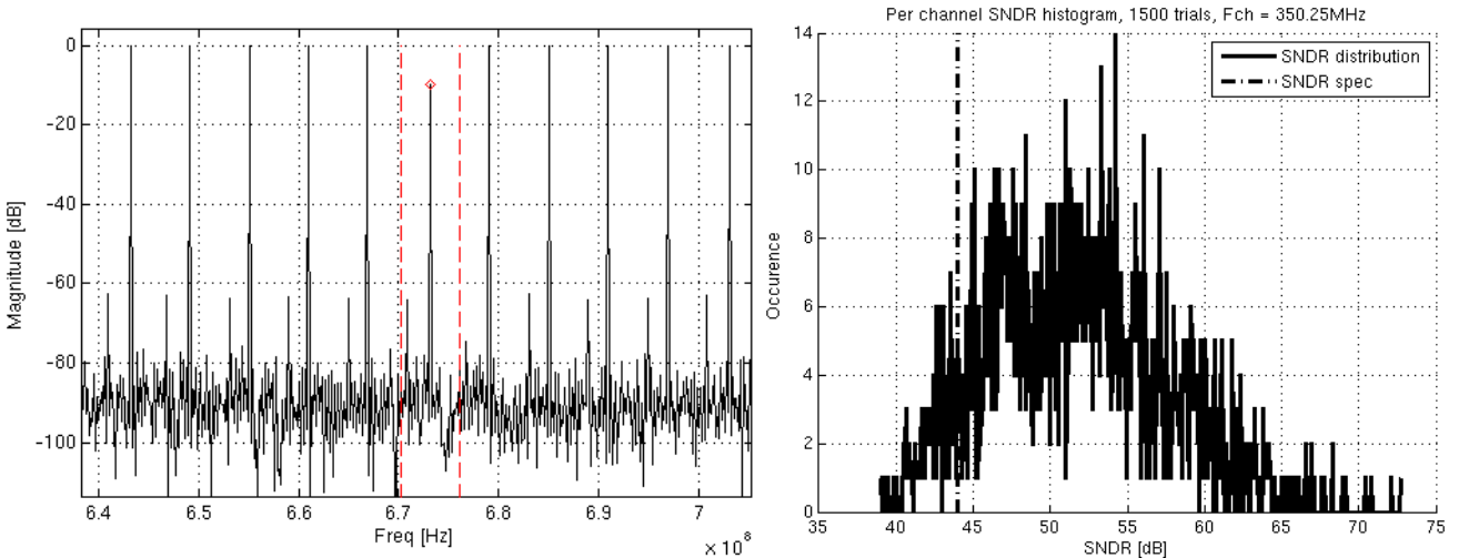
Fig 20. Time-skew mismatch and per-channel SNDR for TP2, \sigma_{\text{skew}}=0.2 ps
