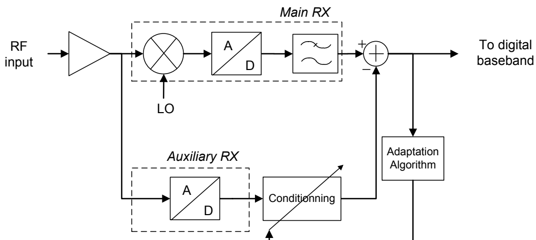
Fig 2. Use of an auxiliary low-resolution broad-band RX to mitigate impairments in a high-resolution narrowband RX
