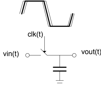
Fig 47. Sampling with a non-ideal clock
