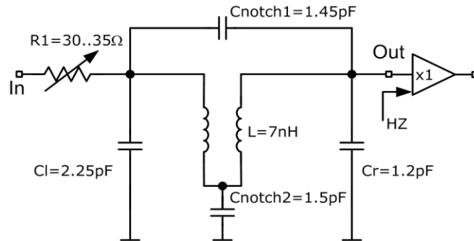
Fig 11. Passive 3 rd order elliptic filter with center tap notch
