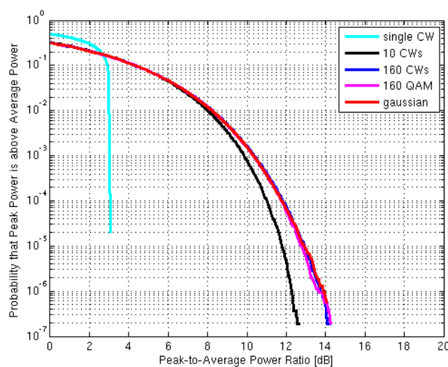
Fig 3. Multi-QAM / Gaussian signals distribution
