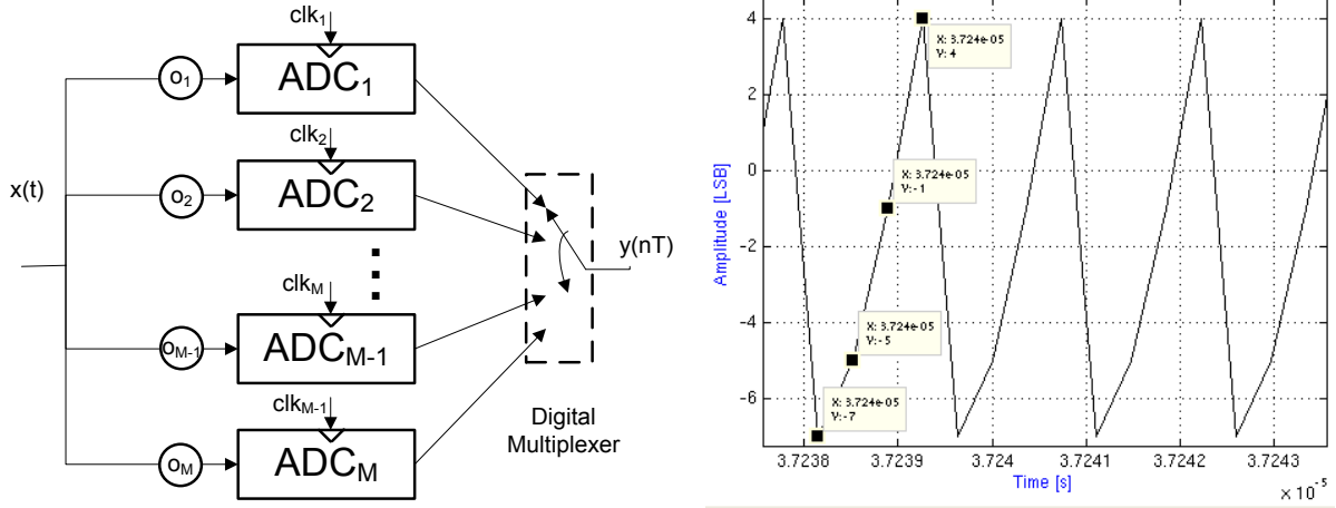
Fig 36. Time-interleaved ADC with offset mismatch (left), time-domain response with four channels & no input signal (right)
