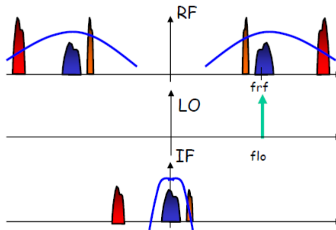
Fig 34. Signal processing operations in a homodyne receiver
