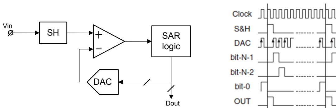
Fig 23. SAR ADC bloc diagram (left), and timing diagram (right)
