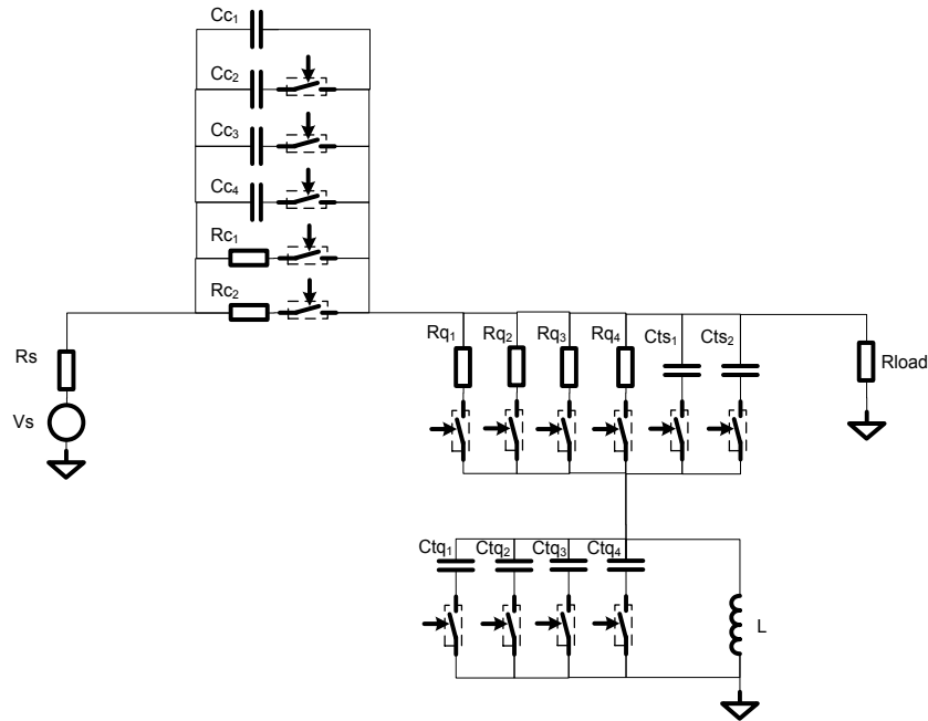
Fig 8. Programmable tilt equalizer principle diagram
