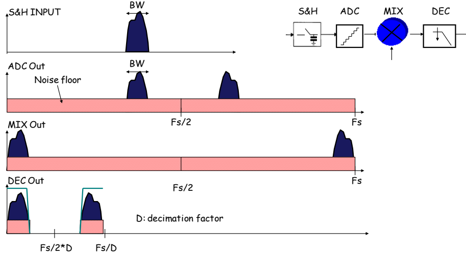
Fig 15. Over-Sampling Factor
