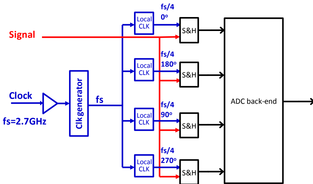
Fig 17. ADC high-level architecture
