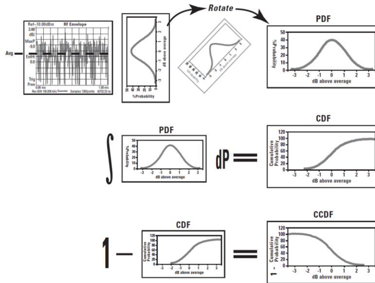
Fig 2. Mathematical origin of the CCDF
