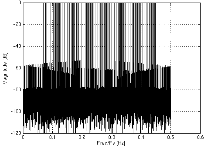
Fig 43. Multi-tone broadband signal digitization with \sigma_{skew}=3.5 \times 10^{-4} \times Fs
