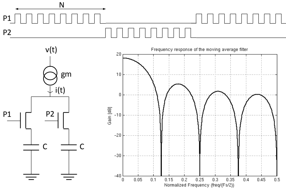
Fig 41. Example of analog FIR filter in the charge domain
