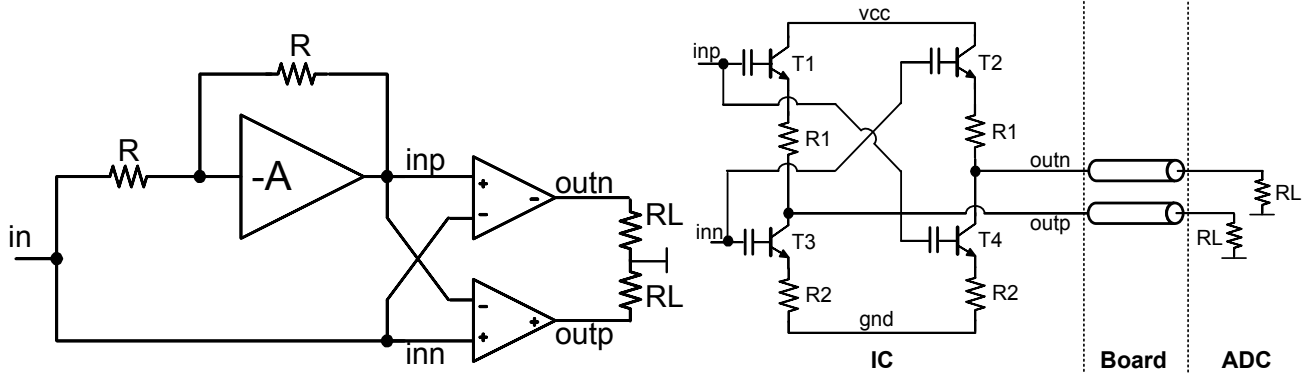
Fig 12. Single-to-differential converter principle diagram (left), Differential-to-differential buffer (right)
