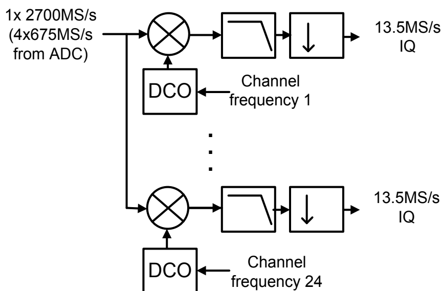
Fig 18. Classical DCS architecture
