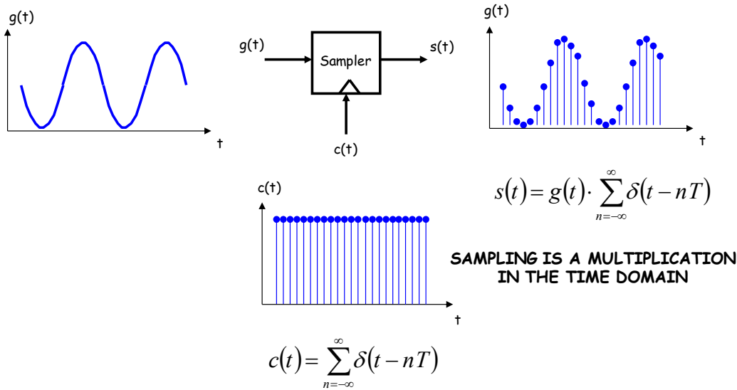
Fig 11. Sampling process
