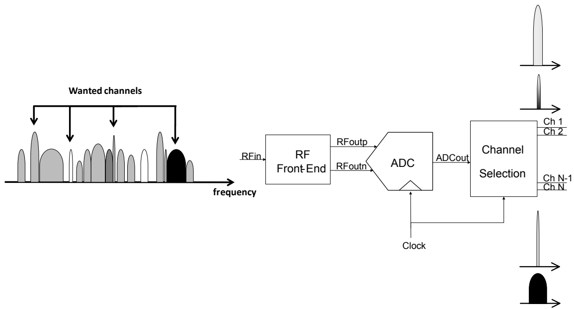
Fig 1. Direct RF digitization receiver
