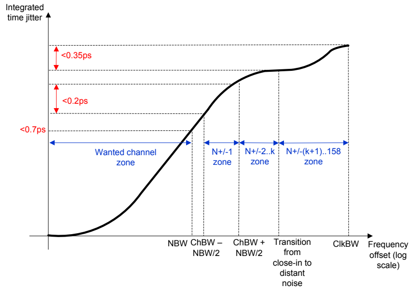
Fig 23. Clock phase noise specification for cable reception
