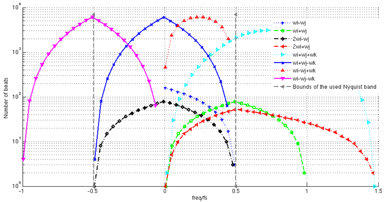
Fig 30. Number of beats across frequency, sampling in 1 st Nyquist band, 158 tones equally distant tones
