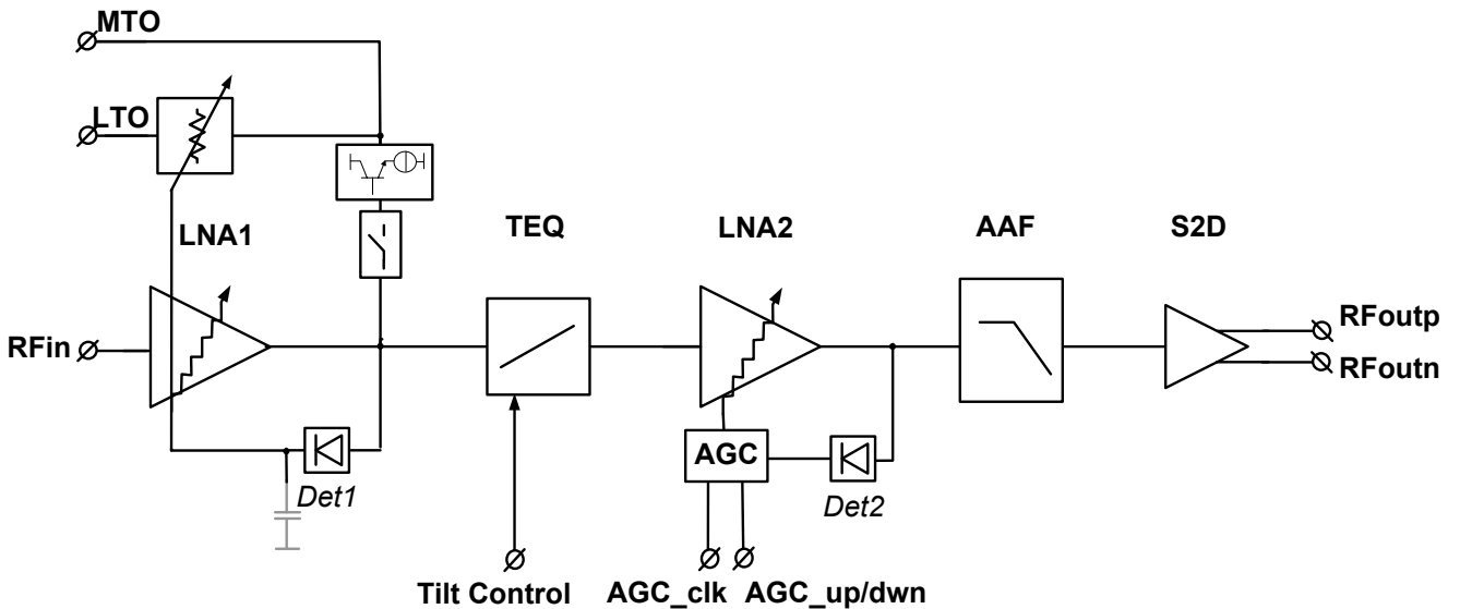
Fig 2. Wideband path of the RFFE IC block diagram
