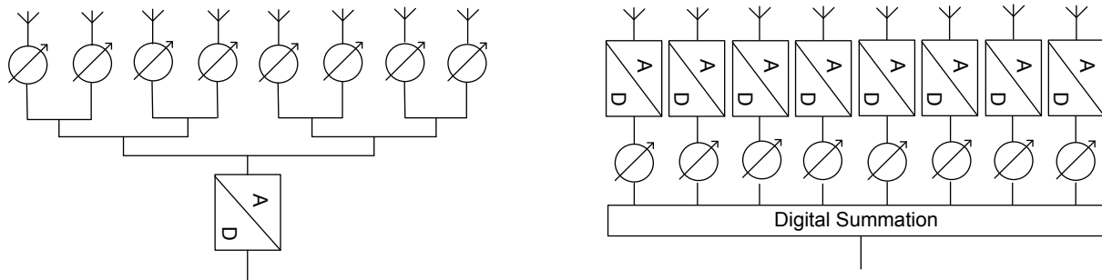
Fig 2. Left: Analog beamforming. Right: Digital beamforming
