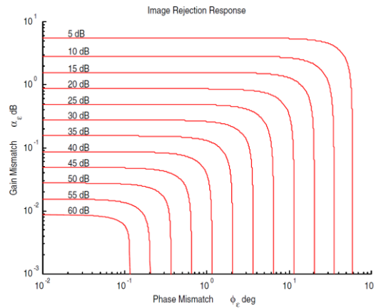
Fig 6. Image rejection ratio
