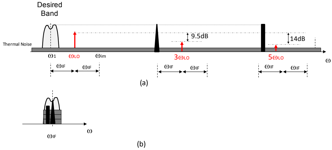
Fig 8. Mixing with LO harmonics
