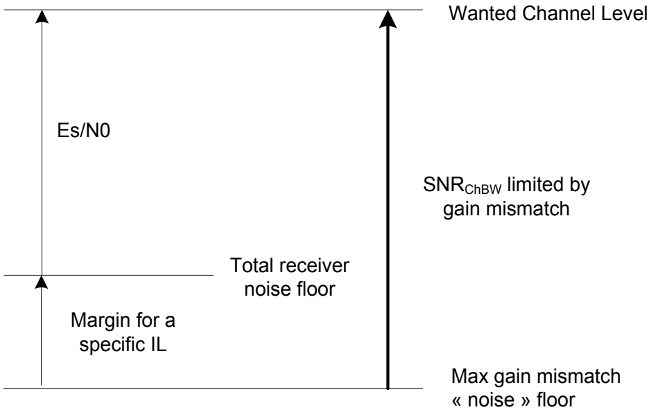
Fig 41. Specification for gain mismatch caused SNR
