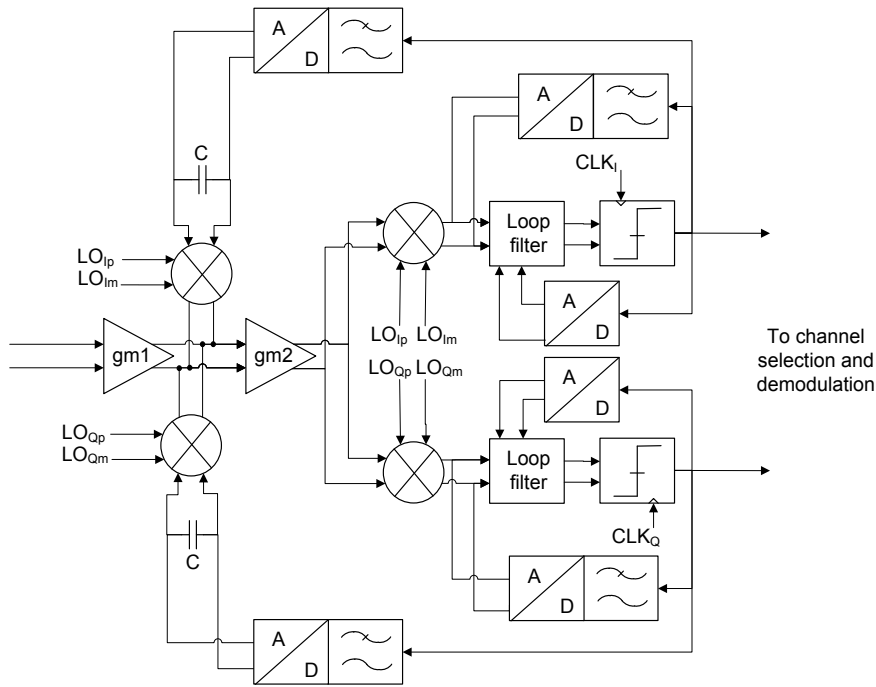
Fig 35. Direct conversion delta-sigma receiver
