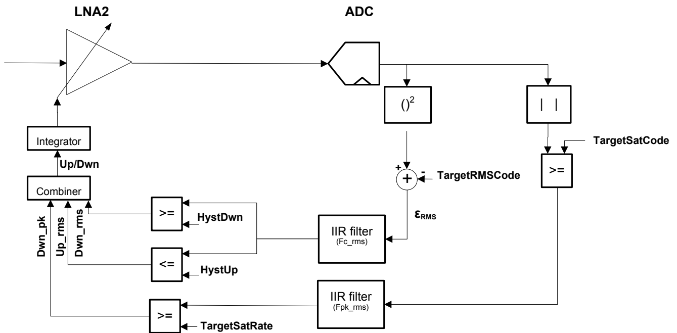
Fig 26. Mixed-signal AGC loop
