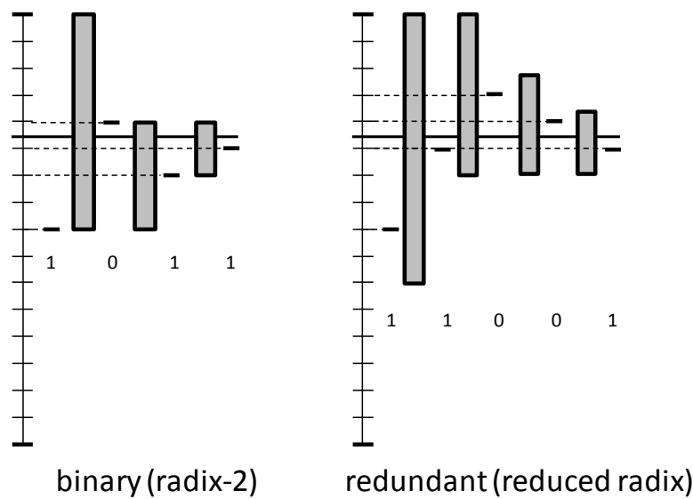
Fig 24. Operation of binary and redundant SAR ADCs
