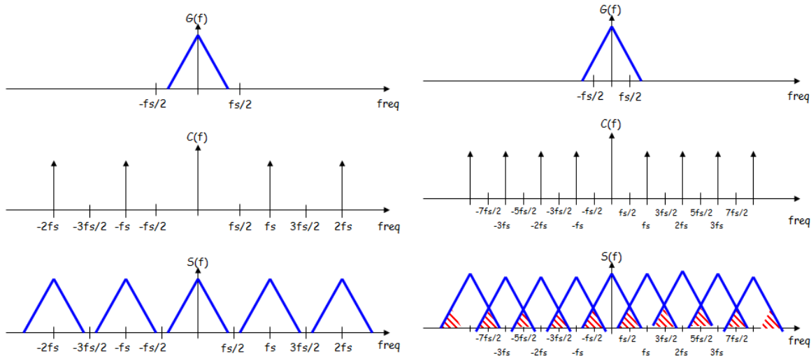
Fig 13. Sampling process in the frequency domain. Left: no aliasing, right: with aliasing
