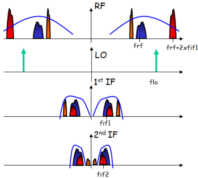
Fig 32. Signal processing operations in dual superheterodyne receiver
