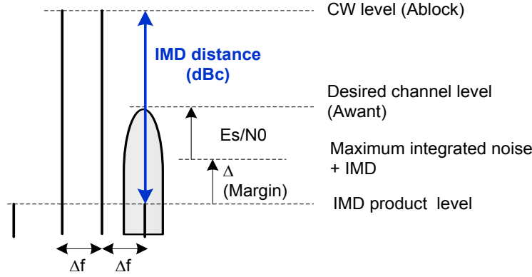
Fig 29. Third-order Intermodulation requirement
