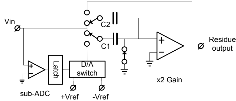
Fig 22. Pipeline stage switched-capacitor implementation
