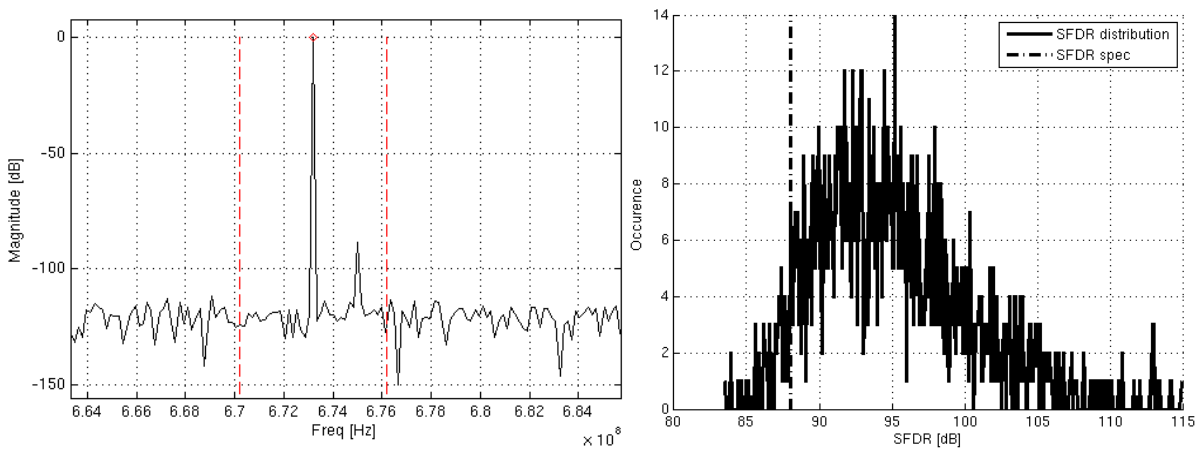
Fig 18. TD simulation of offset mismatch, \sigma_{off}=7\mu V . Left: zoom at F_s/4 on ADC output spectrum, right: SFDRFS/4 distribution
