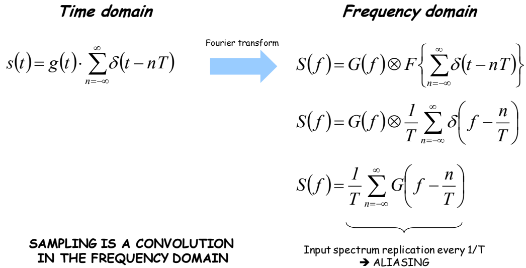
Fig 12. Sampling process: form time-domain to frequency domain
