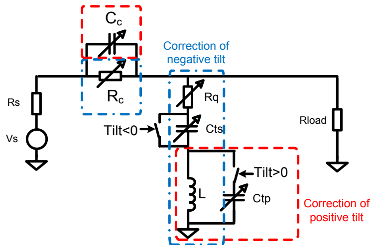
Fig 5. Tilt equalizer topology
