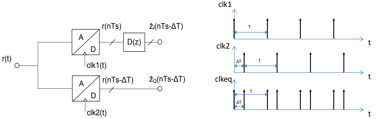
Fig 16. 2 nd -order sampling. Left: block diagram, right: sampling streams
