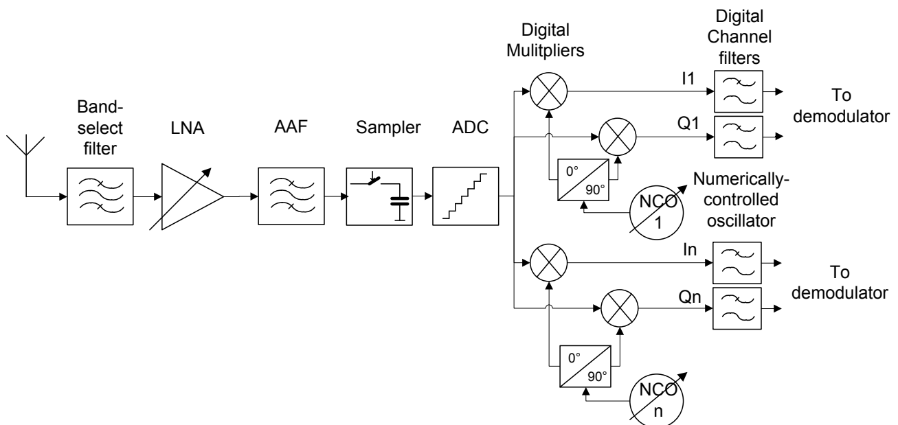
Fig 48. RF sub-sampling receiver
