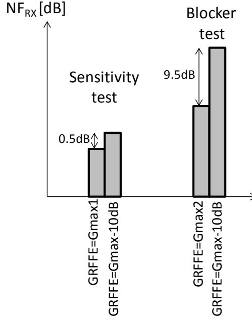
Fig 25. Cascaded Receiver NF, for sensitivity test and blocker test, for different RFFE gains
