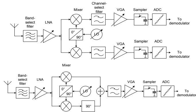
Fig 36. Low-IF receiver (left: complex baseband, right: real baseband)
