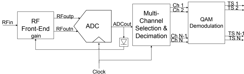
Fig 5. Direct-RF Sampling Home Gateway receiver
