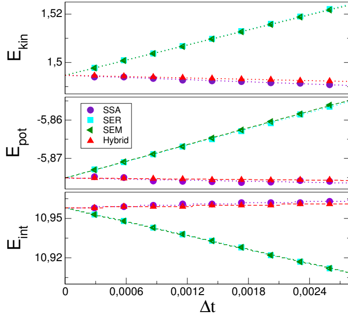
Figure 3.12 | Numerical estimations of the equilibrium properties as a function of the time step for \sigma = 2 obtained with parallel simulations. Top: Kinetic energy estimates (3.4). Middle: Average potential energy (3.5). Bottom: Internal energy estimates (3.6). SSA estimates have been computed on a system of N = 4000 particles on a single processor.
