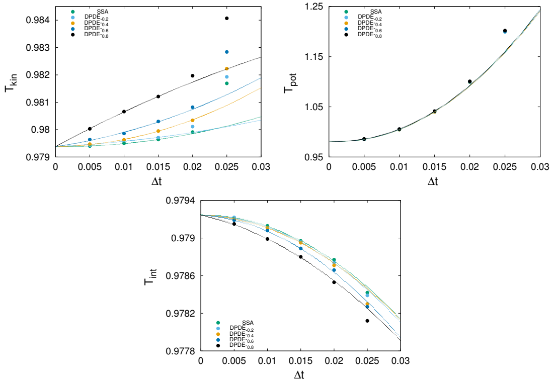
Figure 5.3 | Numerical estimations of the equilibrium temperature as a function of the time step for \sigma = 4 , for DPDE- with various rejection probability and SSA. Top: Kinetic temperature (2.24) (left) and potential temperature (2.25) (right). Bottom: Internal temperature (2.26).
