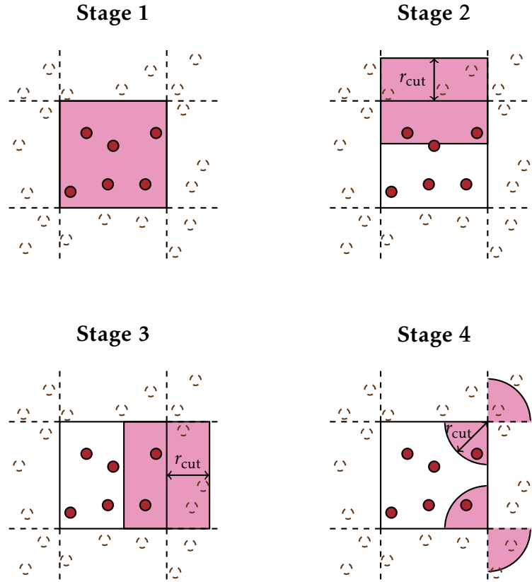
Figure 2.5 | Illustration of the SSA parallelization procedure of [LBM + 14] in a two-dimensional case. Each box represents a space domain allocated to a single processor. The zone highlighted in red defines the region of space where the central processor integrates the elementary fluctuation/dissipation interactions. The same procedure is used by the other processors in the neighboring domains (delimited by dashed lines). Between each stage, all the updated particle's data are sent to their respective processor.
