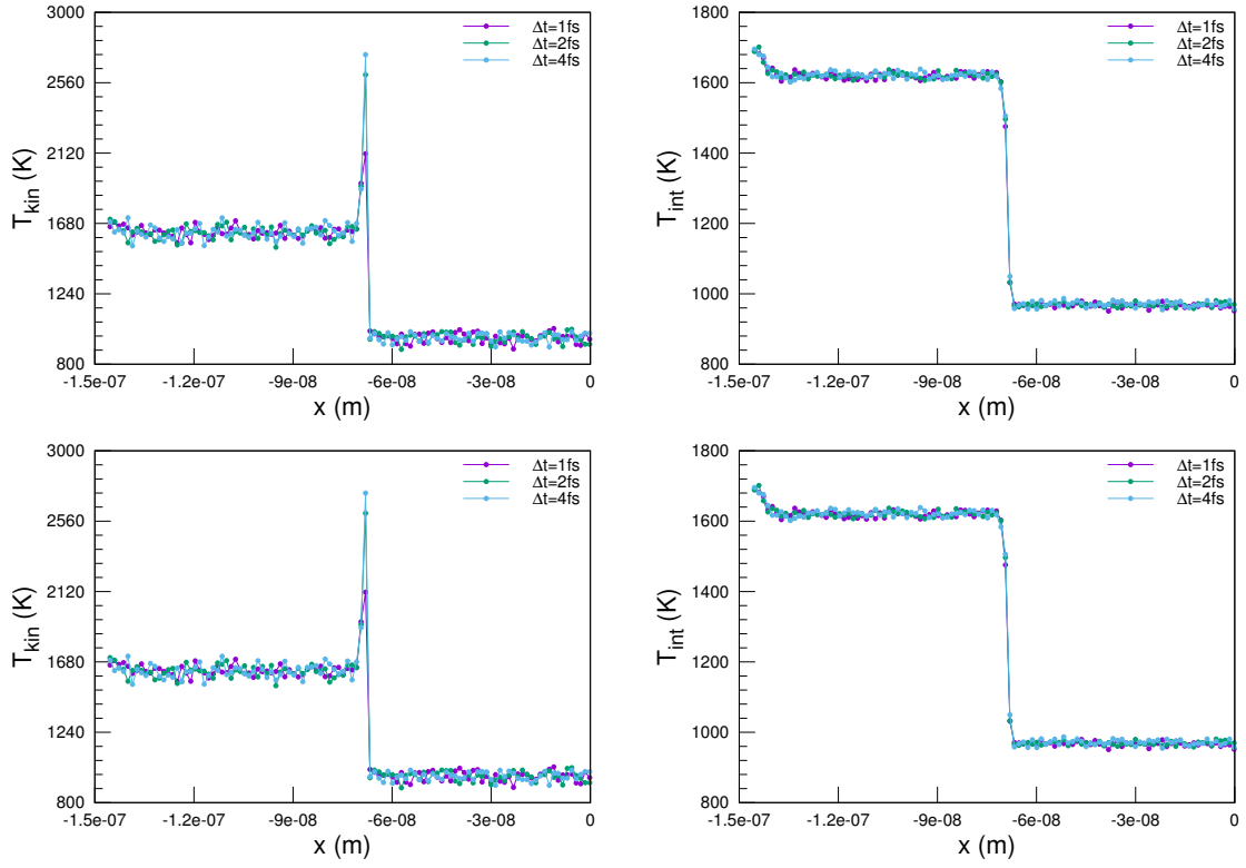
Figure 4.6 | Instantaneous kinetic (left) and internal (right) temperature profiles on the slabs of the cross-section (y,z) for Hybrid (top) and SER (bottom) integrated with time steps ranging from \Delta t = 10^{-15} s to \Delta t = 4 \times 10^{-15} s at time t = 4 \times 10^{-11} s.
