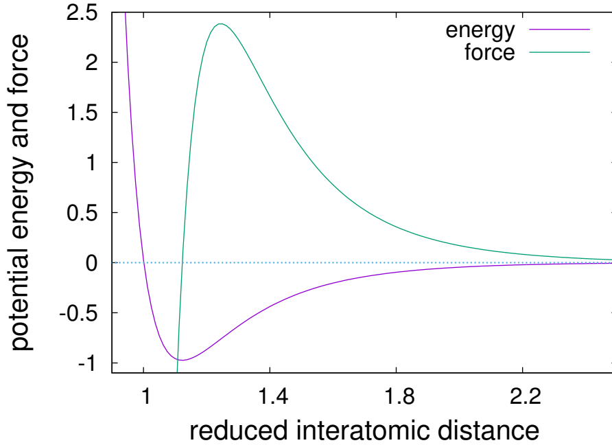
Figure 1.2 | Example of a Lennard-Jones potential where the energy and the distance is expressed in terms of the reference distance \sigma and the reference energy \varepsilon .
