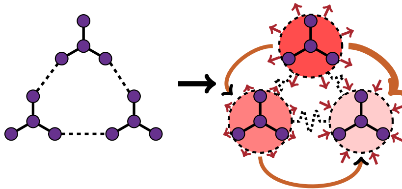
Figure 2.3 | Incorporating the heat conduction to the DPDE: in addition to the mechanical energy variations, thermal exchanges occur between particles with different internal temperatures. The intensity of the heat flows are proportional to the differences between internal temperatures and are represented by the orange arrows: the larger the arrow the more heat is transferred.
