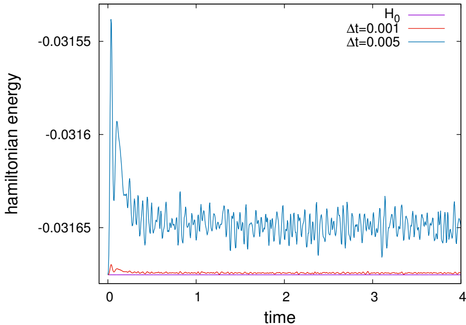
Figure 1.5 | Energy preservation by the Velocity-Verlet scheme (symplectic, see (1.12)) for time steps \Delta t^* = 0.001 and \Delta t^* = 0.005 on an atomistic system described by a Lennard-Jones potential. After a transition time, the energy stabilizes around an average value close to its initial value. The difference between the two increases with the time step, as well as the amplitude of the oscillations around the average stabilized value.
