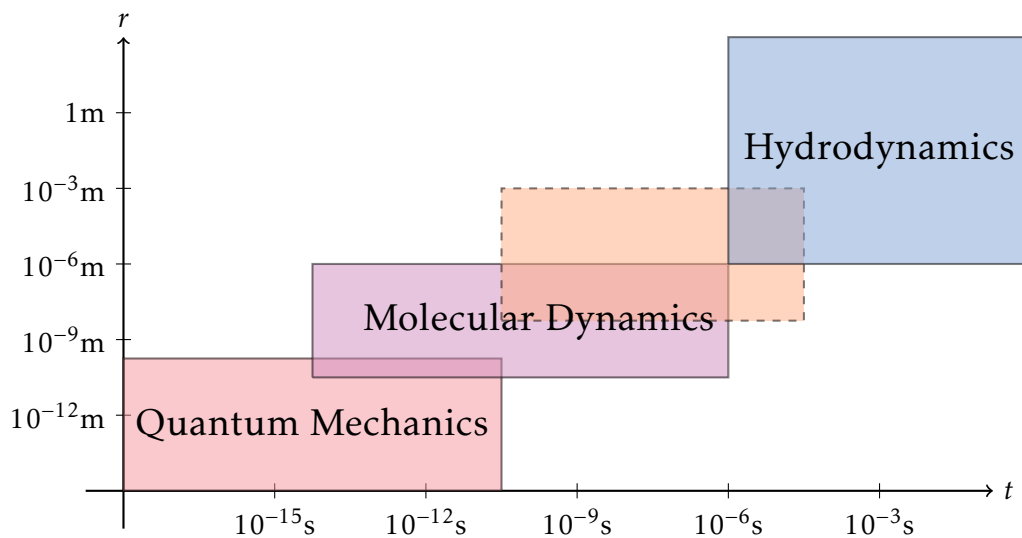
Figure 6 | Approximate scales of length and time of different descriptions of matter. The orange dashed box represents the domain where coarse-graining models are desirable.
