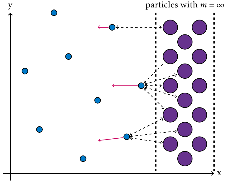
Figure 1.3 | Illustration of fixed wall boundary conditions.
