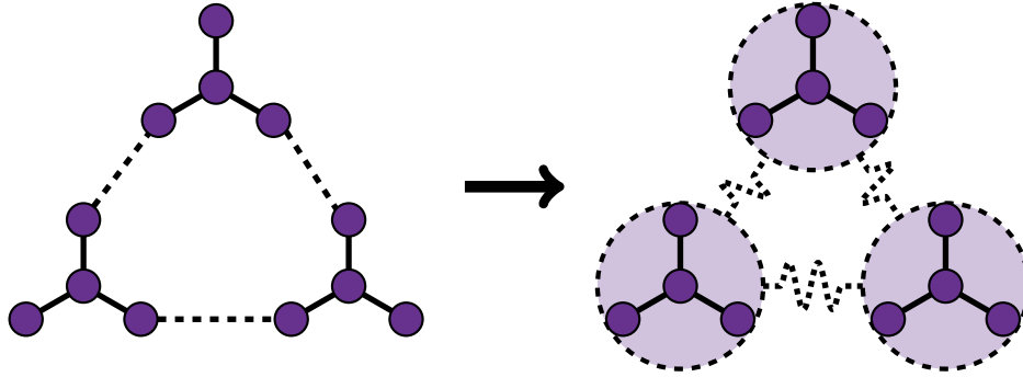
Figure 2.1 | Illustration of DPD coarse-graining process: each of the three molecules (purple atoms) interacting through conservative forces (straight lines: full for short-range interactions and dashed for long-range ones) are represented by a single meso-scale DPD particle (dashed circles) interacting through conservative, friction and random interactions (dashed oscillating lines). Note that DPD interactions are therefore stochastic and no longer deterministic.
