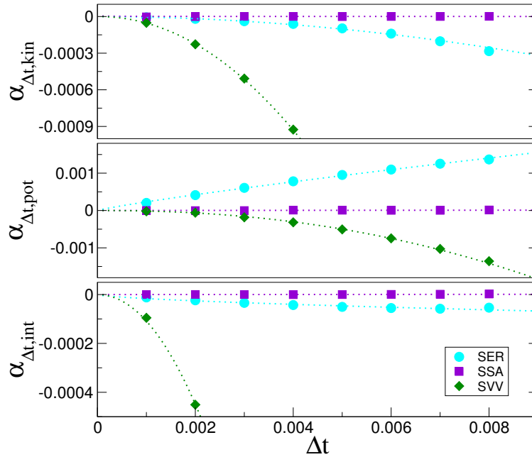
Figure 3.6 | Drift rates per unit time of the kinetic (top), potential (middle) and internal (bottom) energies.
