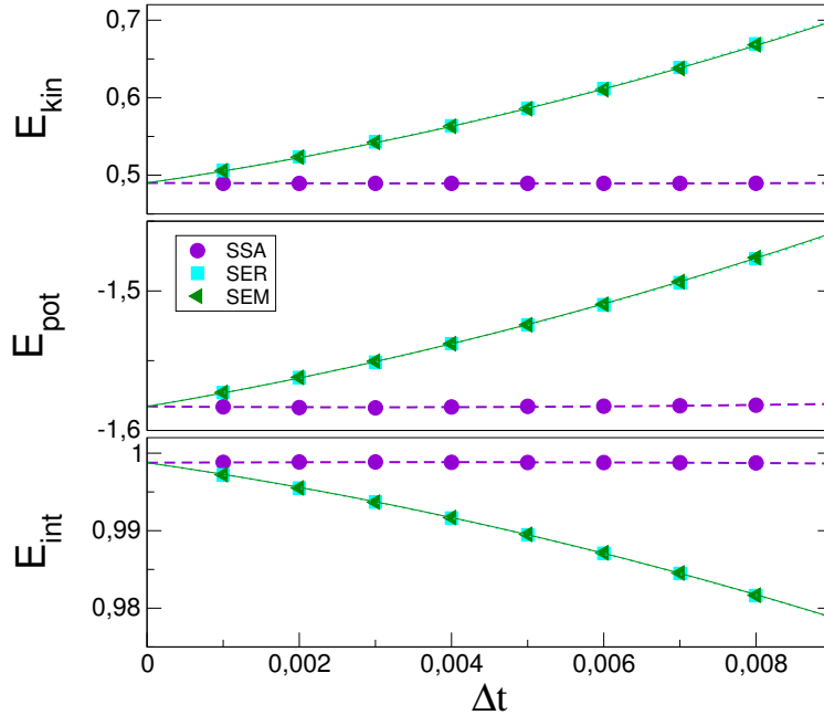
Figure 3.9 | Numerical estimations of the components of the energy as a function of the time step for \sigma = 4 . Top: Kinetic energy (3.4) and potential energy (3.5). Bottom: Internal energy (3.6).
