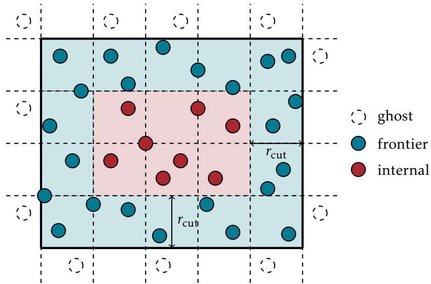
Figure 5.2 | The enclosed box in the full lines represents the space domain allocated to processor p , the exterior region being allocated to other processors. Internal-internal or internal-frontier elementary fluctuation/dissipation interactions are discretized with a SSA interaction. Frontier-ghost elementary fluctuation/dissipation interactions are neglected.
