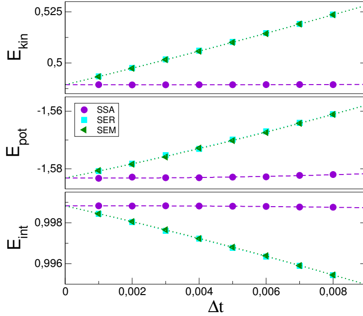
Figure 3.10 | Numerical estimations of the components of the energy as a function of the time step for \sigma = 2 . Top: Kinetic energy (3.4) and potential energy (3.5). Bottom: Internal energy (3.6).
