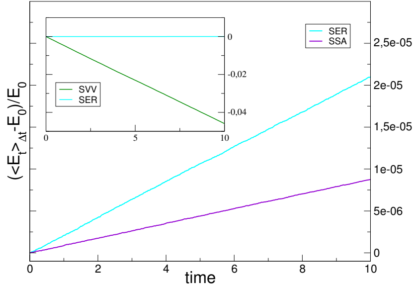
Figure 3.3 | Time-dependent energy drift averaged over trajectories, as a function of time when \Delta t = 0.006 , for three-dimensional simulations.
