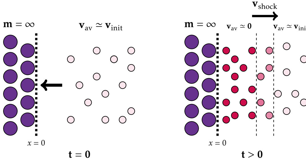
Figure 4.1 | Schematic of the shocked system simulation procedure. At t = 0 , we set the equilibrated system in motion toward the left wall at a velocity v_{\text{init}} = -2000 \text{ m.s}^{-1} (left drawing). The system is compressed when it reaches the wall, and a shock wave propagates at velocity v_{\text{shock}} > v_{\text{init}} from the left to the right of the simulation box (right drawing). The particles on the left of the shock front are hotter and more densely distributed than those on the right.
