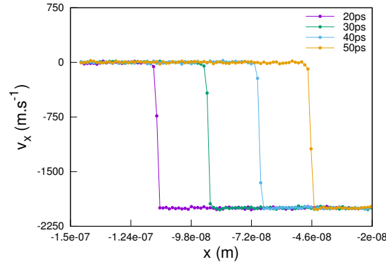
Figure 4.7 | Instantaneous velocity on the x -axis profiles averaged on the slabs normal to the x -axis of an Hybrid simulation or \Delta t = 10^{-15} s (SER yields similar results).
