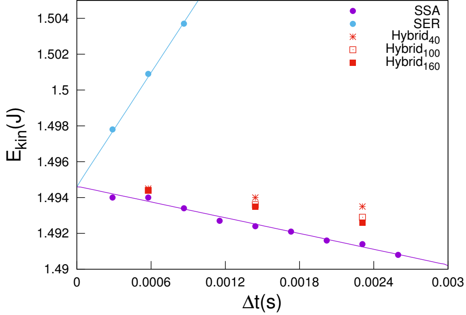
Figure 3.13 | Kinetic energy estimations for Hybrid simulations with a number N_x of particles along the x axis equal to 40, 100 and 160. The SSA and SER estimations displayed are those reported in Figure 3.12.
