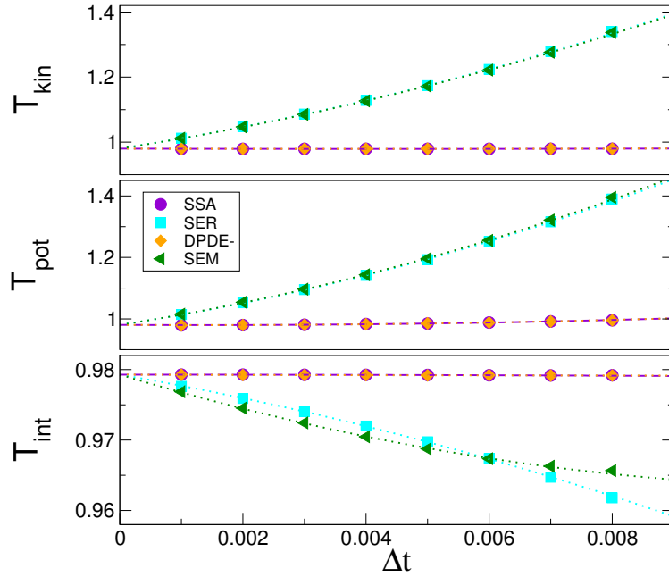
Figure 5.4 | Numerical estimations of the equilibrium temperature as a function of the time step for \sigma = 4 (with \eta = 0.5 ). Top: Kinetic temperature (2.24) and potential temperature (2.25). Bottom: Internal temperature (2.26). Results of DPDE- and SSA are on top of each other.
