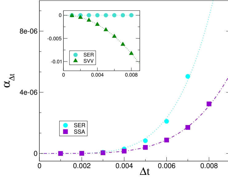
Figure 3.5 | Average energy drift rate \alpha_{\Delta t} as a function of the time step. A fit \alpha_{\Delta t} = K\Delta t^\omega is superimposed to the data.
