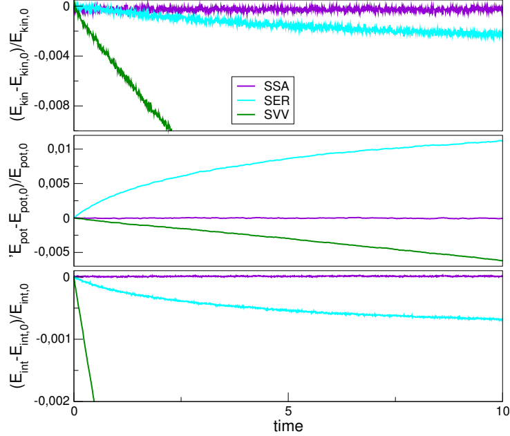
Figure 3.7 | Time-dependent drift for the kinetic (top), potential (middle) and internal (bottom) components of the energy, averaged over trajectories, as a function of time when \Delta t = 0.006 .
