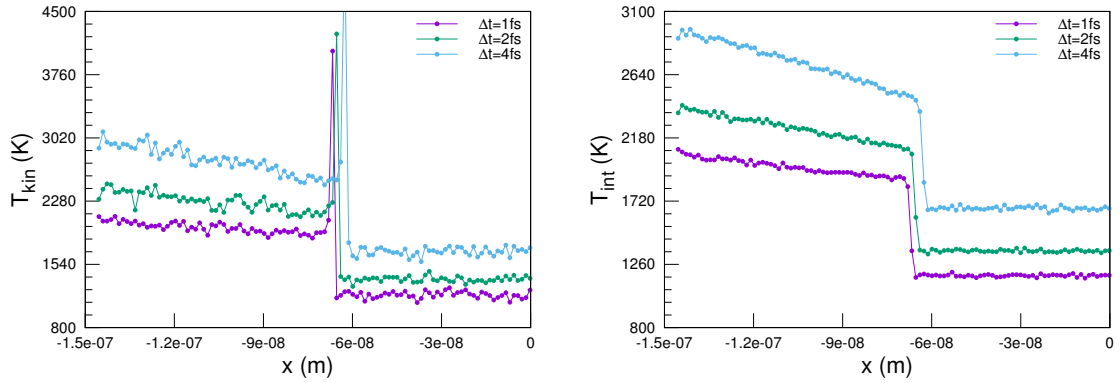
Figure 4.4 | Instantaneous kinetic (left) and internal (right) temperature profiles on the slabs of the cross-section (y,z) for the SEM scheme integrated with time steps ranging from \Delta t = 10^{-15} s to \Delta t = 4 \times 10^{-15} s at time t = 4 \times 10^{-11} s.
