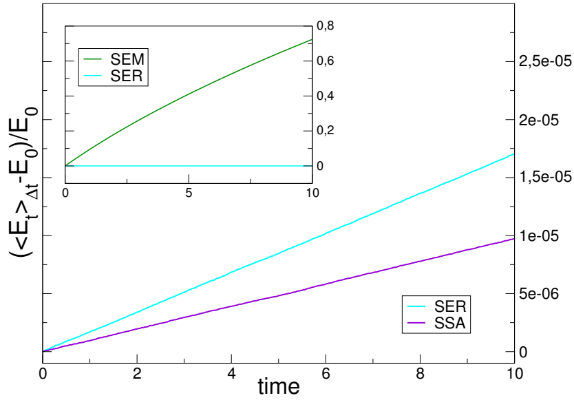
Figure 3.4 | Time-dependent energy drift averaged over trajectories, as a function of time when \Delta t = 0.006 , for two-dimensional simulations.
