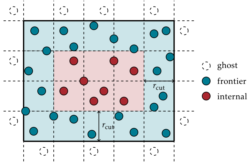
Figure 2.4 | Illustration of the SSA parallelization issue: the enclosed box in the full lines represents the space domain allocated to a given processor, the exterior region being allocated to other processors. The dashed boxes of length r_{\text{cut}} represent the cells of the linear scaling techniques: a particle on a given cell can only interact with particles in the neighboring cells. The dashed particles ("ghost" particles) are particles allocated to other processors. The particles at a distance r > r_{\text{cut}} of the frontier ("internal" particles, in red) never interact with ghost particles: the sequentiality of the integration does not affect the computation speed because no additional idle time nor information transfer between processors are needed. The particles at a distance r < r_{\text{cut}} of the frontier ("frontier" particles, in blue) interact with ghost particles: the processor eventually has to wait before accessing any ghost particle's data, or wait for another processors to access its frontier particle's data, thus generating delays.
