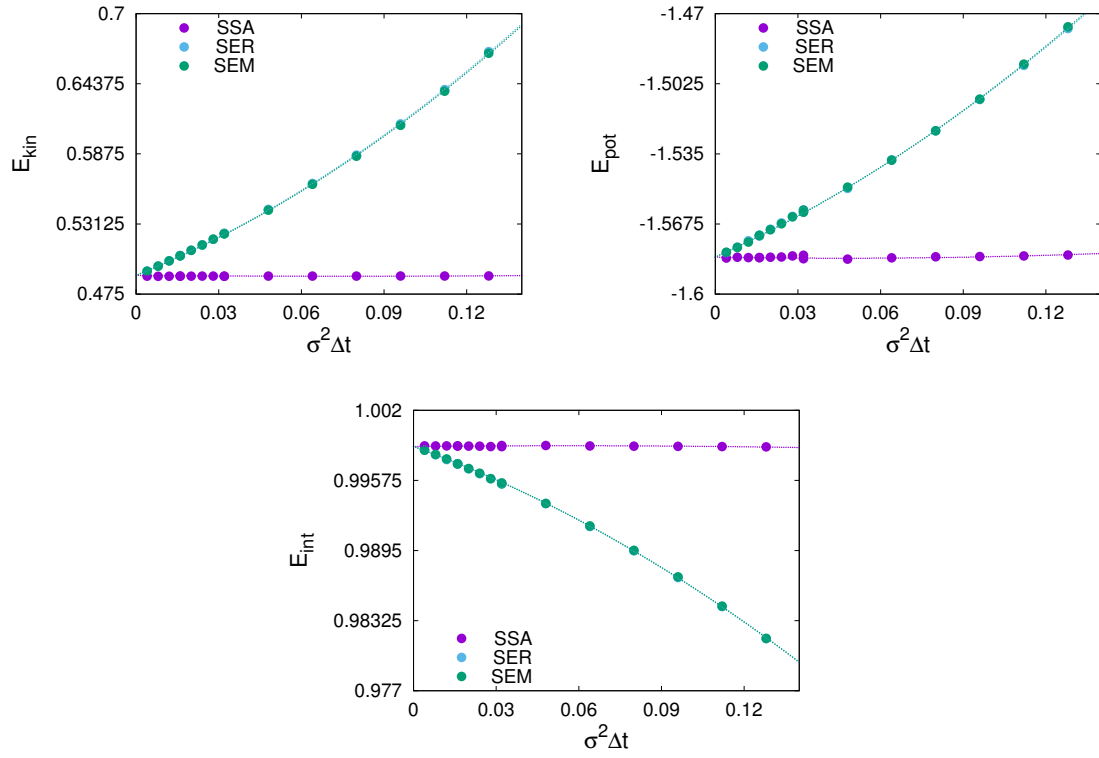
Figure 3.11 | Numerical estimations of the components of the energy as a function of \sigma^2 \Delta t . Top: Kinetic energy (3.4) and potential energy (3.5). Bottom: Internal energy (3.6).
