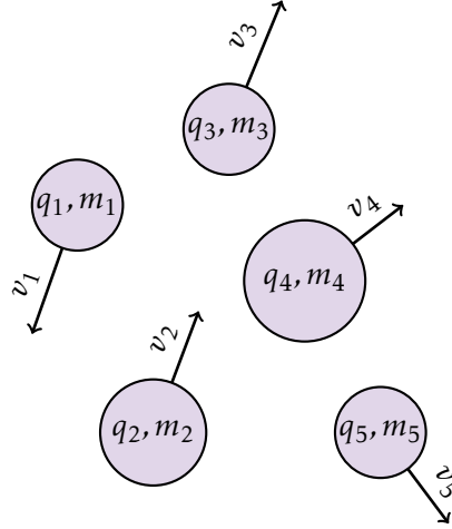
Figure 1.1 | Two-dimensional representations of particles in the classical description of matter: Each particle indexed by i is represented by its position q_i , its mass m_i and its momentum p_i = m_i v_i (where v_i is its velocity).
