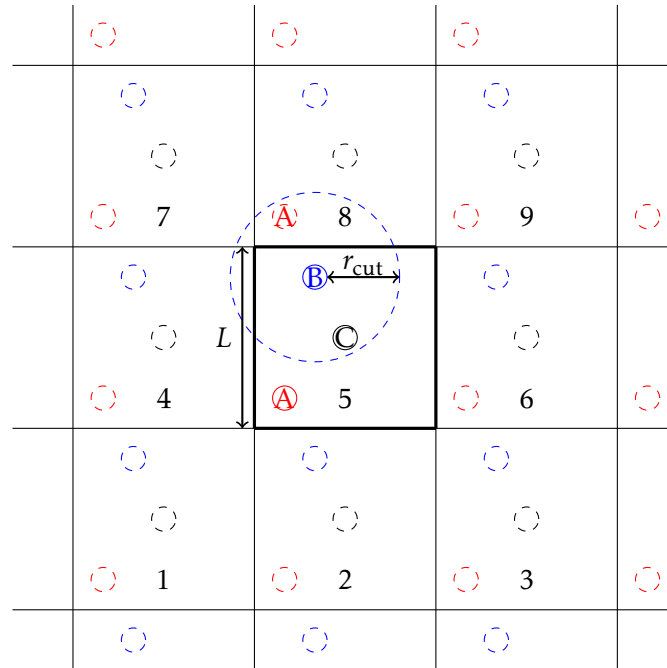
Figure 1.4 | Example of a two-dimensional simulation box with periodic boundary conditions applied. Particle B interacts with particle C in the box 5 (main box) but also with the periodic image of particle A in box 8.
