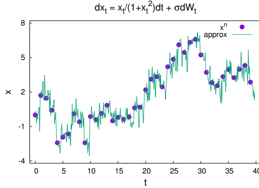
Figure 1.6 | Example of the approximation \tilde{x}_t defined by (1.31) of the Euler-Maruyama discretization of the dynamics dx_t = \frac{x_t}{1+x_t^2}dt + \sigma dW_t , with \sigma = 3 . The dots are realizations of the EM scheme and the line is a discrete approximation of the process \tilde{x}_t using a very small time step.
