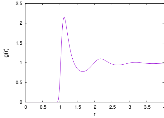
Figure 3.1 | Computed radial distribution function g(r) of the considered fluid at equilibrium. The radial distribution function represents the probability for each atom to find a neighboring atom according to a distance r . The above plot represents a liquid, where particles are semi-organized, yielding peaks of decreasing amplitude that do not touch zero.
