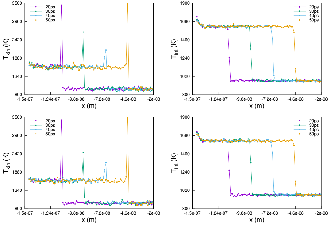
Figure 4.5 | Instantaneous kinetic (left) and internal (right) temperature profiles on the slabs of the cross-section (y, z) for the Hybrid (top) and SER (bottom) schemes integrated with a time step \Delta t = 10^{-15} s.
