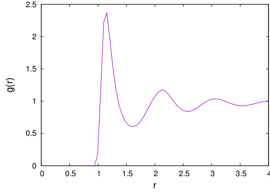
Figure 3.8 | Computed radial distribution function g(r) of the considered fluid at equilibrium. We see that the higher density yields oscillations of greater amplitude than in Figure 3.1.
