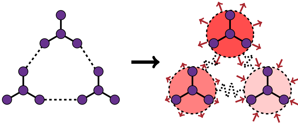
Figure 2.2 | Illustration of DPDE coarse-graining process: in addition to the DPD coarse-graining process (dashed lines and circles, see Figure 2.1), the meso-scale particles have internal temperatures and energies (the redder the color the hotter the particle). Internal/external equilibration is done through energy exchanges, turning internal energy into kinetic energy and reversely.
