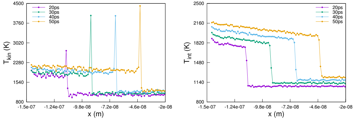
Figure 4.3 | Kinetic (left) and internal (right) temperature average on the slabs of the cross-section (y,z) for the SEM scheme integrated with a time step \Delta t = 10^{-15} s.
