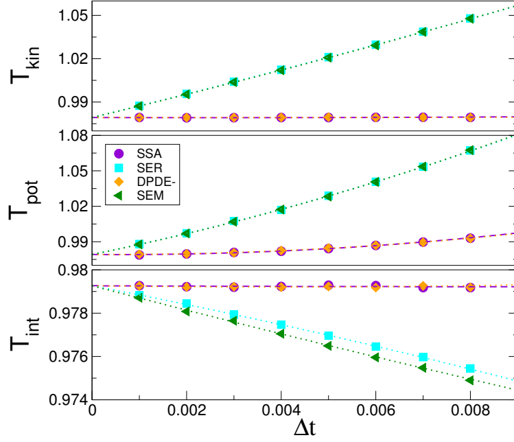
Figure 5.5 | Numerical estimations of the equilibrium temperature as a function of the time step for \sigma = 2 (with \eta = 0.5 ). Top: Kinetic temperature (2.24) and potential temperature (2.25). Bottom: Internal temperature (2.26). Results of DPDE- and SSA are on top of each other.
