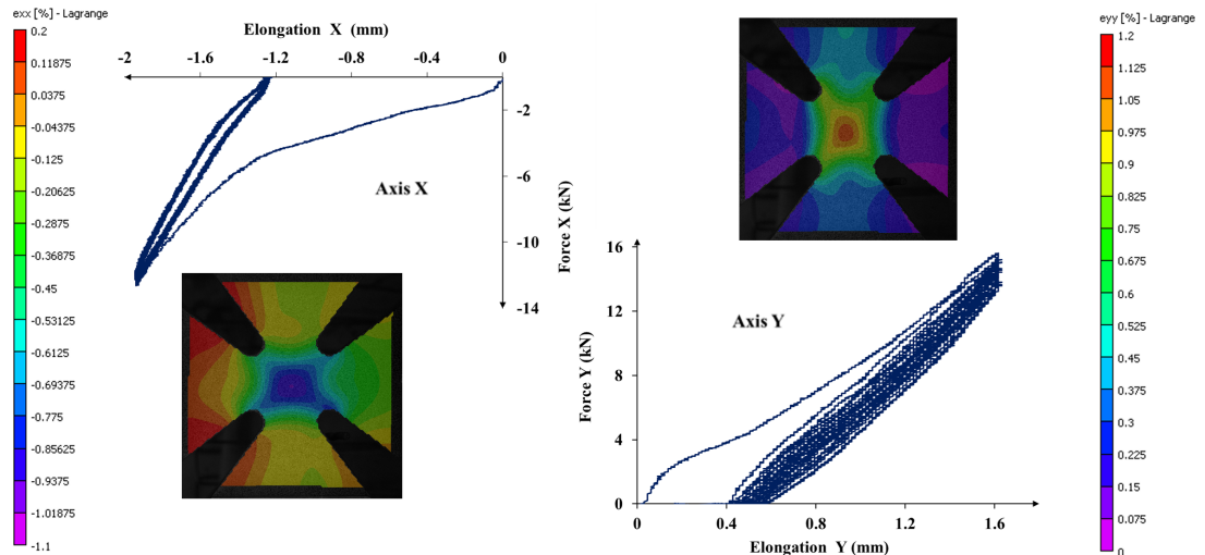
FIGURE 2.13 – Force-elongation diagram of Sample 1 on axes X and Y with the respective strain maps at the end of loading of the last cycle sequence A.
