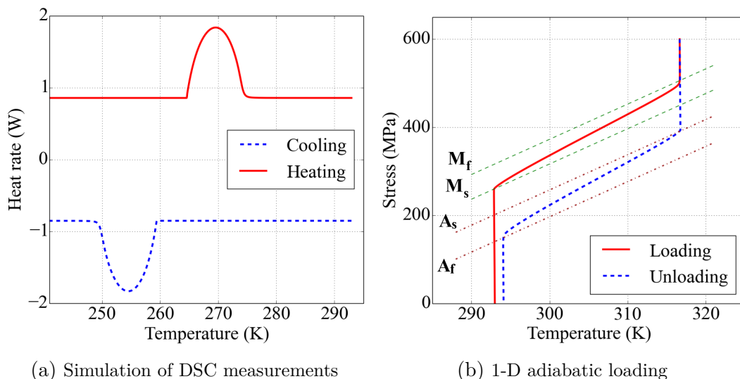
FIGURE 4.4 – Heat rate - temperature diagram of a simulated DSC test (a) and stress-temperature relation on a phase diagram for a simulated 1-D stress-controlled loading under adiabatic conditions (b) for a hypothetical NiTi composition. The starting temperature is 293 K in both cases.
