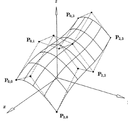
Figure 2.8: A quadratic x cubic Bézier surface
