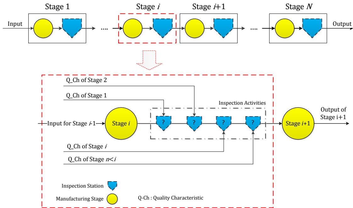
Figure 3.1. Inspection of quality characteristics in a serial MPS
