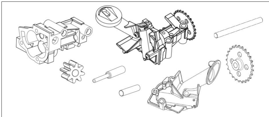
Figure 3 . La pompe
