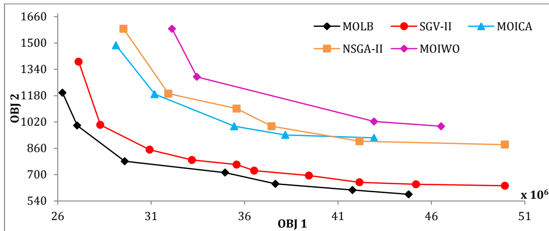
Figure 5.12. NFs of different meta-heuristics from problem number 30
