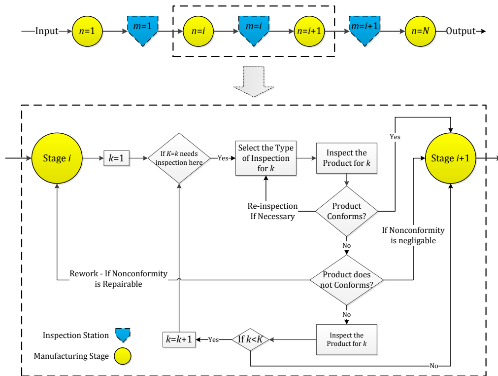
Figure 2. Inspection planning problem in a MPS
