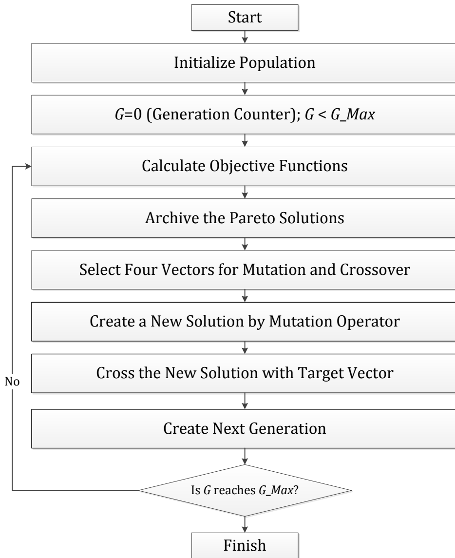
Figure A3.5. Genetic algorithm flowchart
