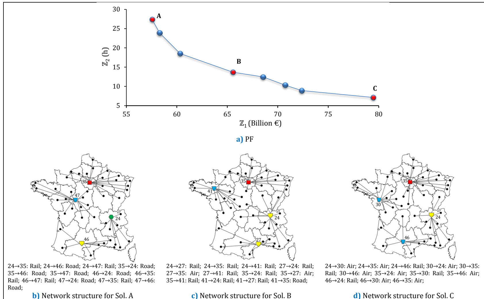
Figure 5.17. Results of \mathbb{P}_4
