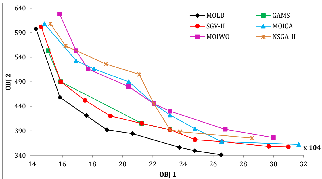
Figure 5.11. NFs of different meta-heuristics fro problem number 5
