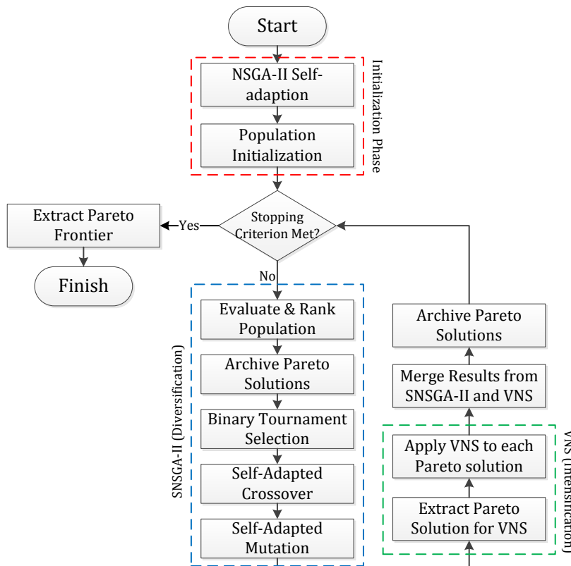
Figure 5.6. Flowchart of the proposed SGV-II
