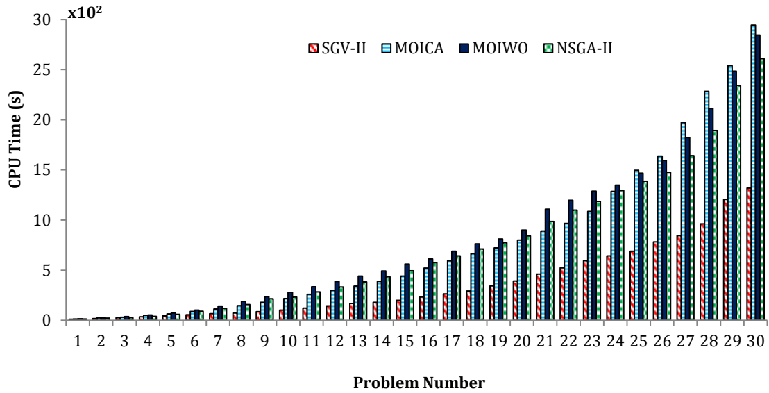
Figure 5.10. CPU time of different algorithms for different problems
