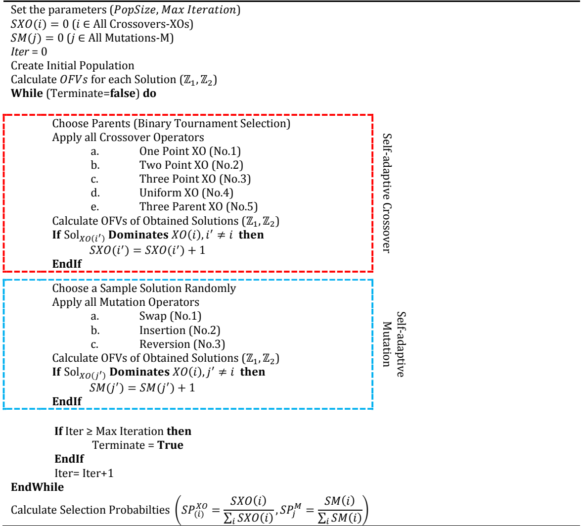
Figure 5.5. Pseudo code of SNSGA-II's initialization phase
