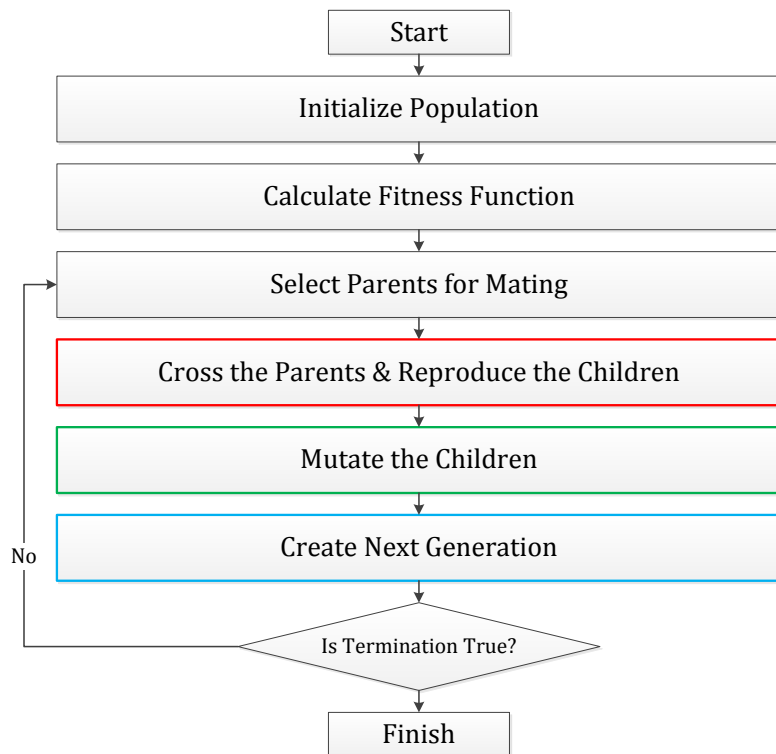
Figure A3.1. Genetic algorithm flowchart
