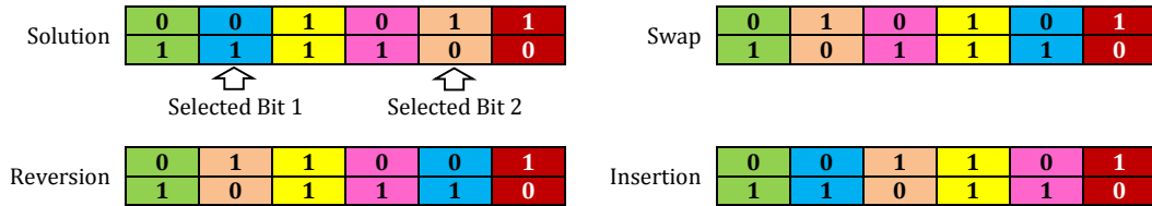
Figure A3.3. Mutation operators
