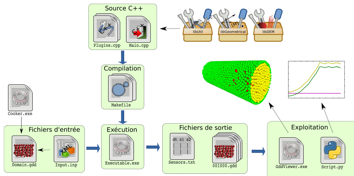
FIGURE E.1 – Architecture de GranOO [Charles 13].
