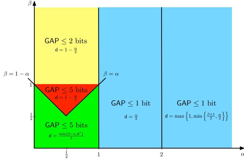
Figure 4.4: Different regimes depending on the values of \alpha and \beta , with d^* := \max\{\alpha, 1 - \alpha\} + \max\{\alpha, 1 + \beta - \max\{\alpha, \beta\}\} .
