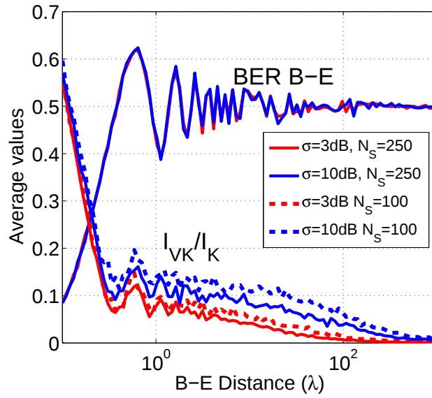
Figure 4-7: Averaged BER and vulnerable key bits as function of the separation distance d between Bob and Eve.
