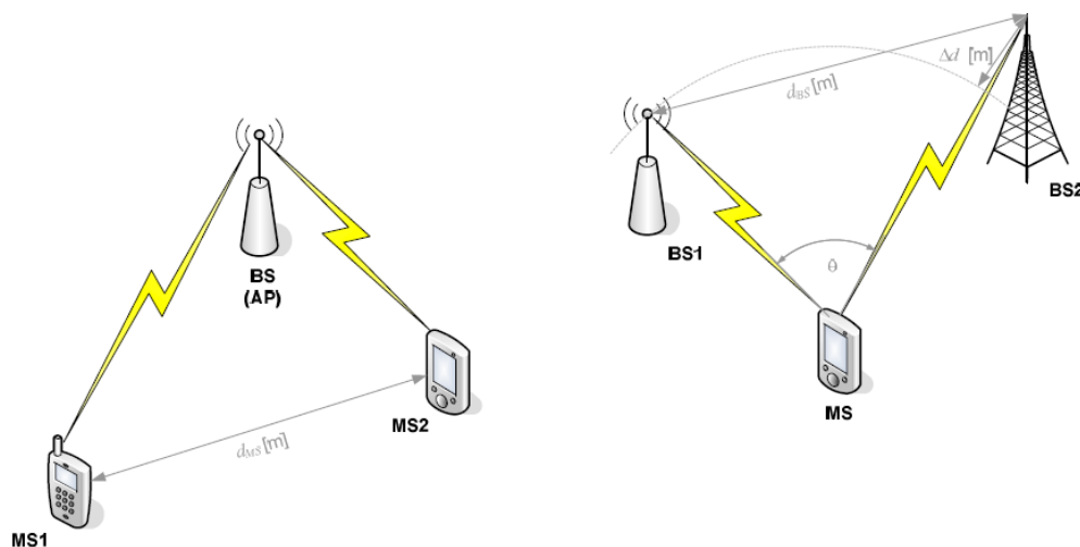
Figure 4-1: Shadow fading auto-correlation (right) and shadow fading cross-correlation (left) [1].
