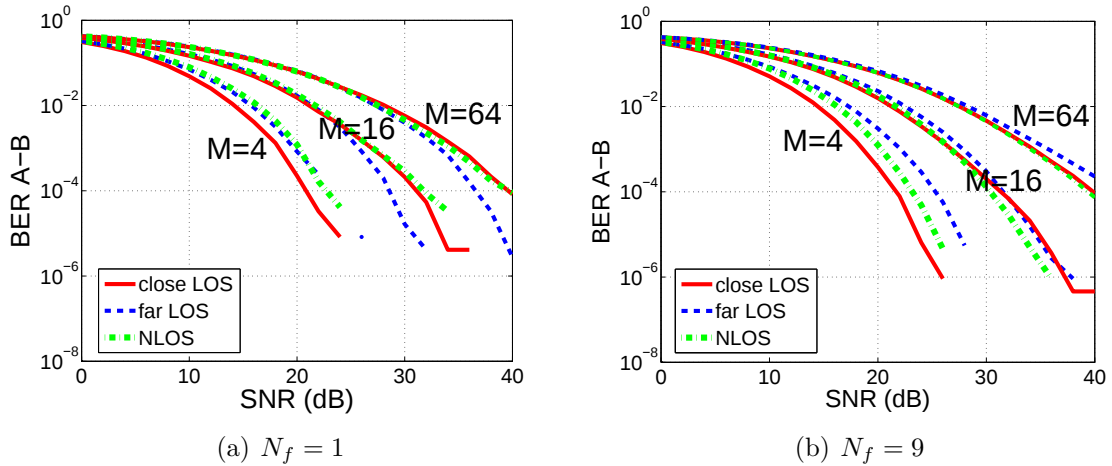
Figure 6-4: Alice-Bob BER vs. SNR and M .
