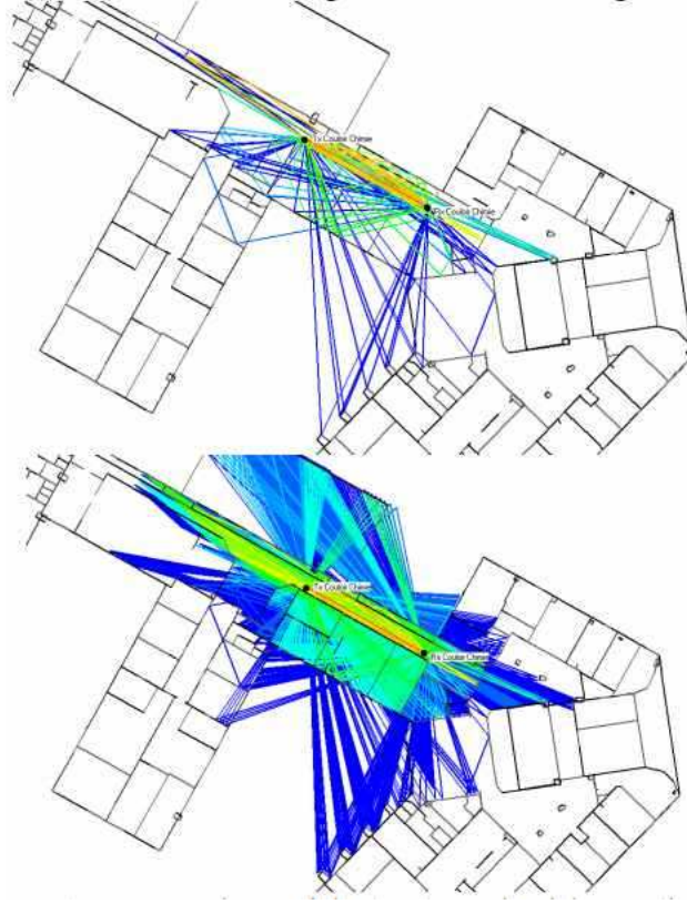
Figure 5-1: Example of an (indoor) deterministic simulation without (up) and with (down) diffuse scattering.
