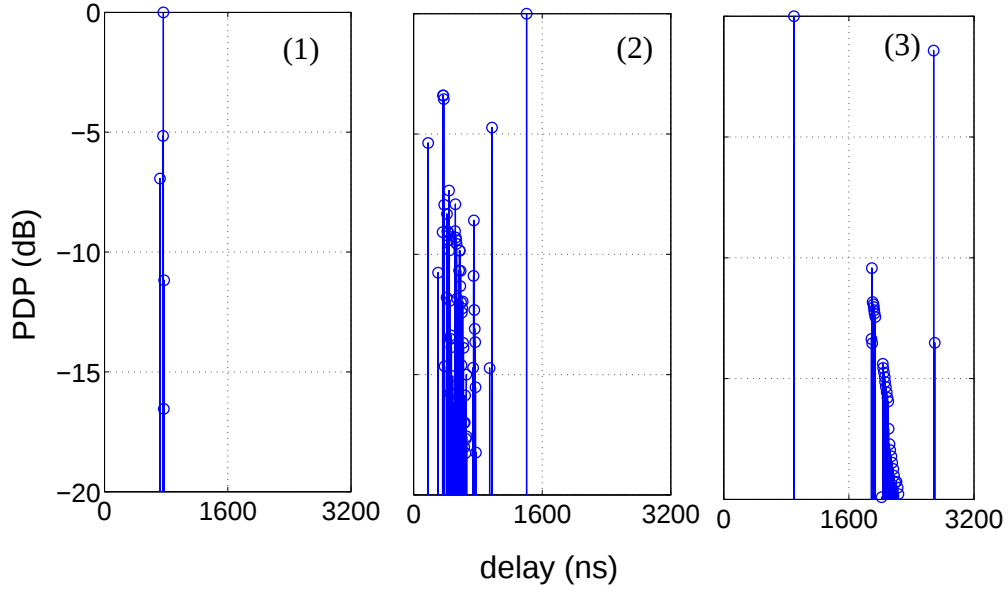
Figure 5-5: Some examples of PDPs corresponding to Louvre48 (right: \sigma_\tau = 15 ns, middle: \sigma_\tau = 360 ns, left: \sigma_\tau = 728 ns).
