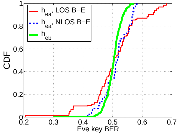
Figure 6-7: BER of Eve key bits for M = 4 and for NB channels.
