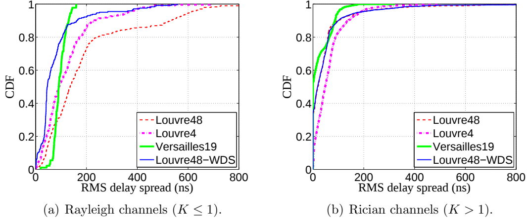
Figure 5-4: RMS delay spread statistics.
