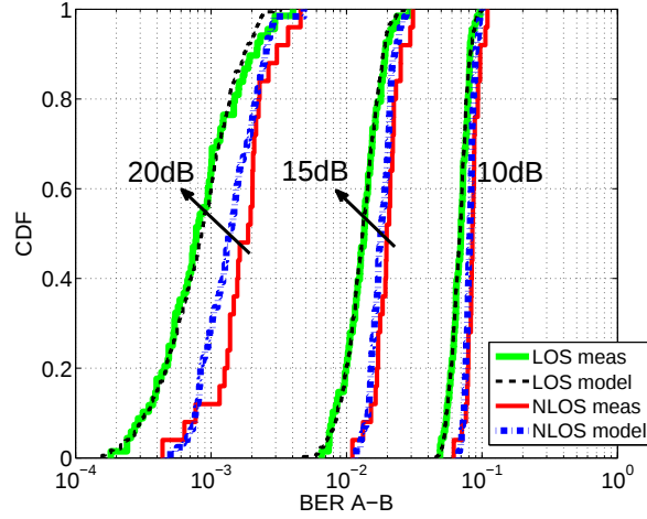
Figure 6-6: Comparison of the BER A-B computed over both the measurements and the model, for SNR=10, 15 and 20 dB.
