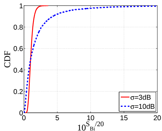
Figure 4-4: Log-normal shadowing per path for both \sigma = 3 dB and \sigma = 10 dB.
