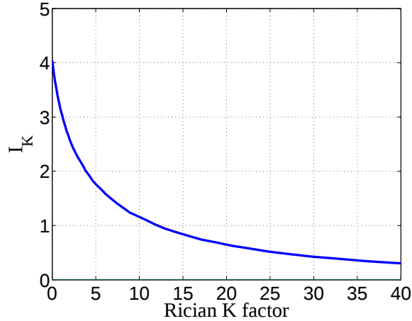
Figure 3-3: I_K as a function of the Rician K factor.
