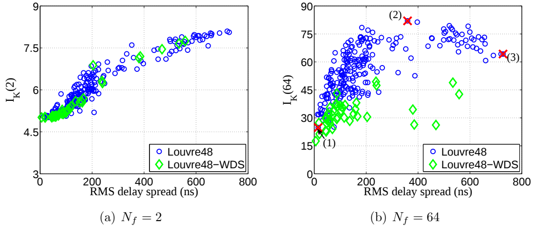
Figure 5-9: I_K as a function of the RMS delay spread ( \sigma_\tau ) for the scenario Louvre48.
