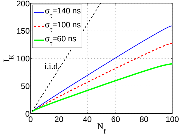
Figure 3-11: Evolution of I_K with respect to N_f and to RMS delay spread \sigma_\tau , for \Delta_\tau = 20 ns.
