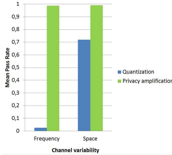
Figure 7-10: Mean pass rates before and after privacy amplification, for MKSM.
