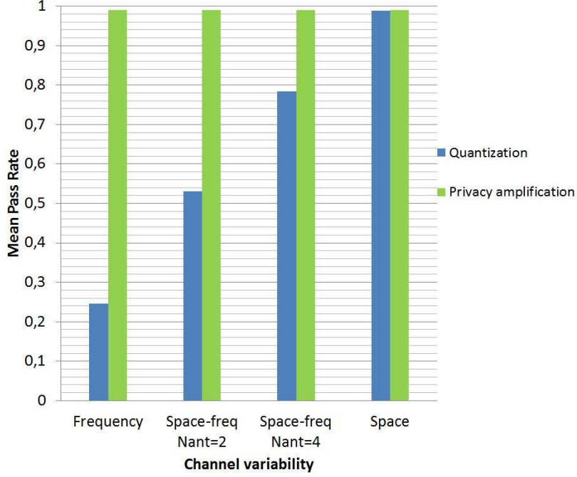
Figure 7-4: Mean pass rates before and after privacy amplification, for SKSM.
