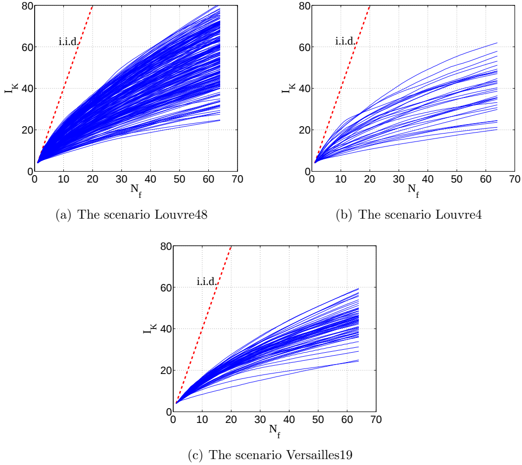
Figure 5-8: Evolution of I_K with respect to the number of frequencies N_f .
