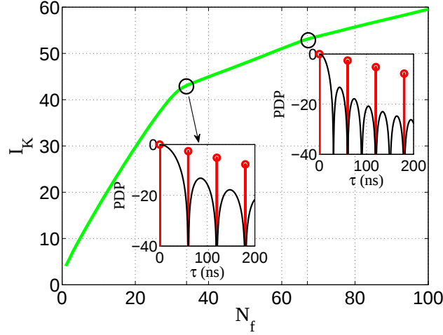
Figure 3-10: Equivalent time domain when perfectly resolved paths, for \Delta_\tau = 60 ns and \sigma_\tau = 100 ns.
