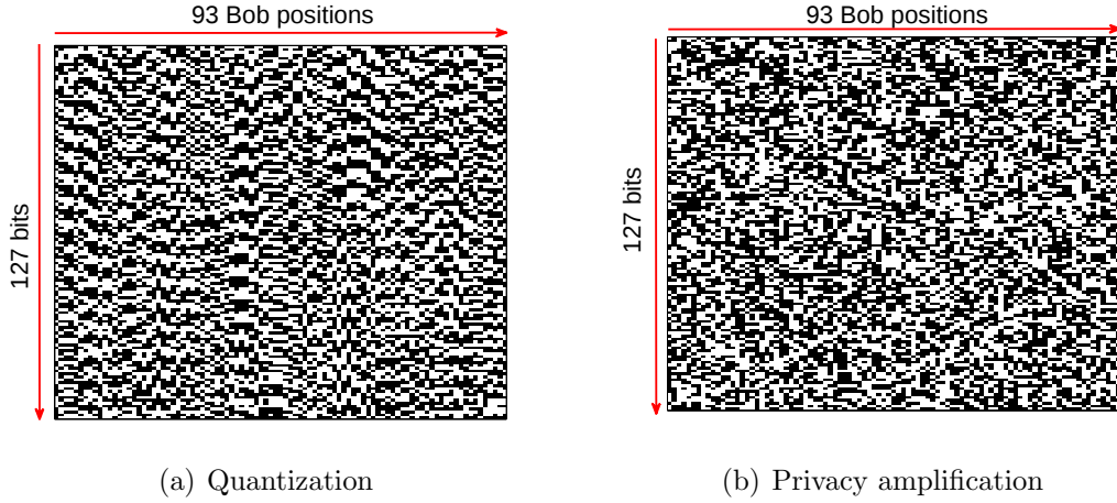
Figure 7-8: Keys from joint space-frequency DoFs ( N_{ant} = 4 ), for different Bob positions and for SKSM.
