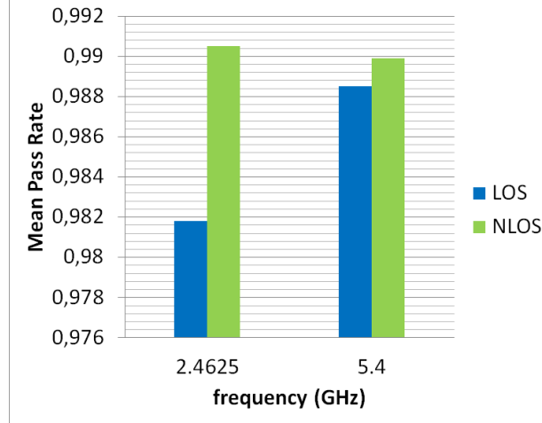
Figure 6-10: Mean pass rate exploiting spatial variability with respect to LOS/NLOS and for N = 128 .
