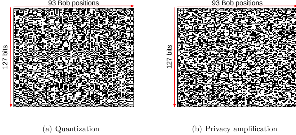
Figure 7-11: Keys from spatial DoFs, over Bob positions and for MKSM.
