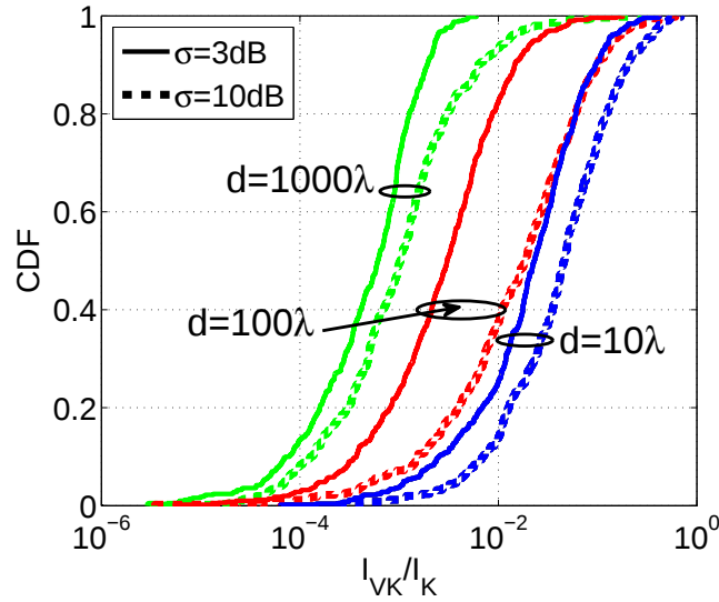
Figure 4-6: CDF of relative vulnerable key bits.
