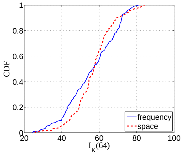
Figure 5-15: Space vs. frequency variability.
