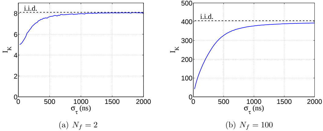
Figure 3-12: Variation of I_K with the RMS delay spread for \Delta_\tau = 20 ns.
