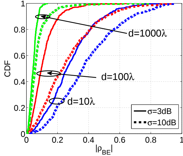
Figure 4-3: CDF of complex channel correlations.
