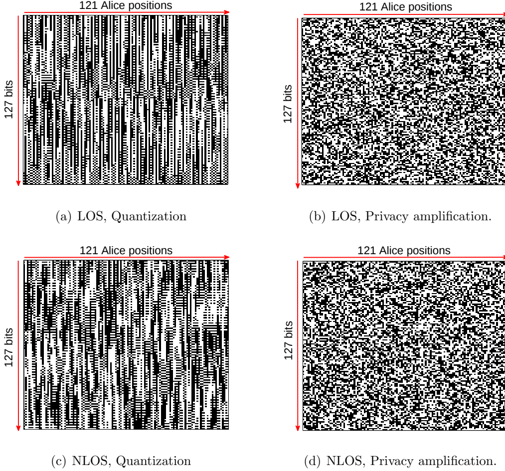
Figure 7-9: Keys from frequency DoFs, over Alice positions and for SKSM.
