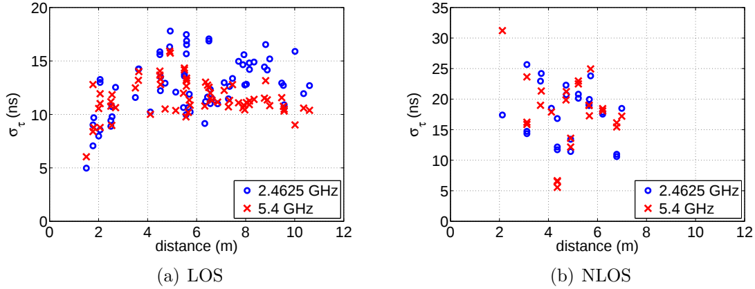
Figure 6-12: The variation of the RMS delay spread with the distance.
