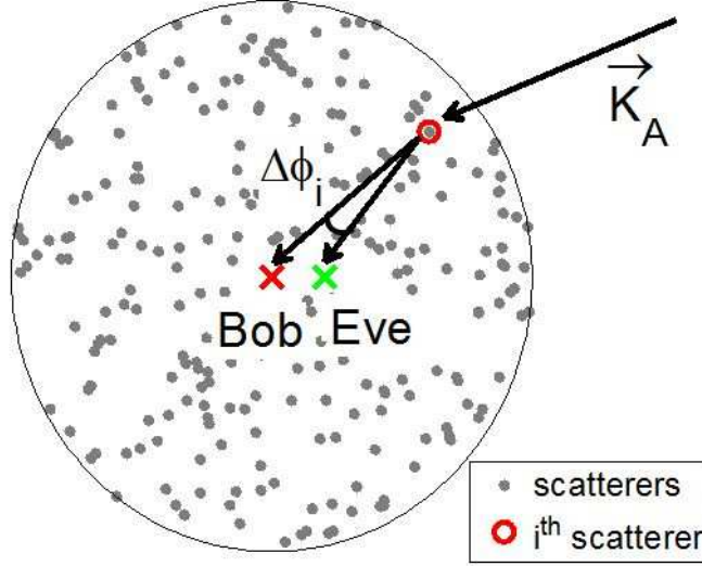
Figure 4-2: Geometrical representation of the communication scenario.
