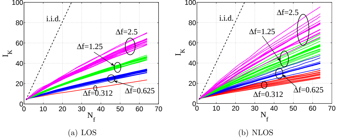
Figure 6-17: I_K as a function of N_f and the BW.
