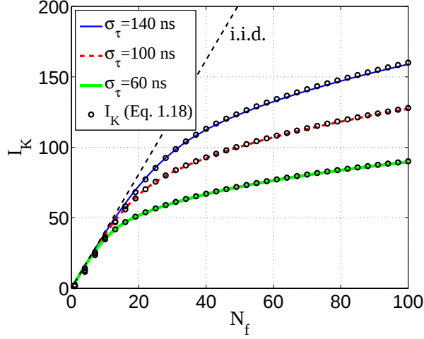
Figure 3-13: I_K as a function of N_f for BW = 50 MHz.
