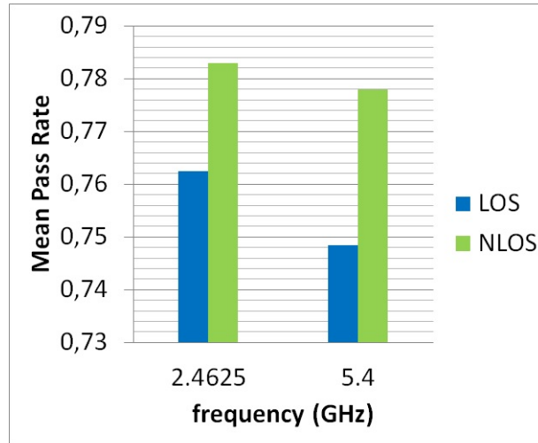
Figure 6-14: Mean pass rate exploiting frequency variability for BW = 40 MHz and M = 16 .
