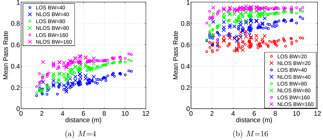
Figure 6-13: Mean pass rate as a function of the distance for 5.4 GHz and for frequency variability.
