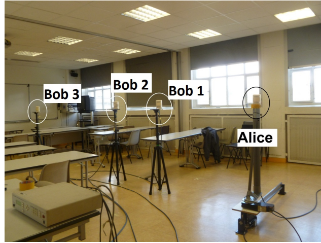
Figure 6-2: A sketch of measurement run in TPT classrooms scenario.
