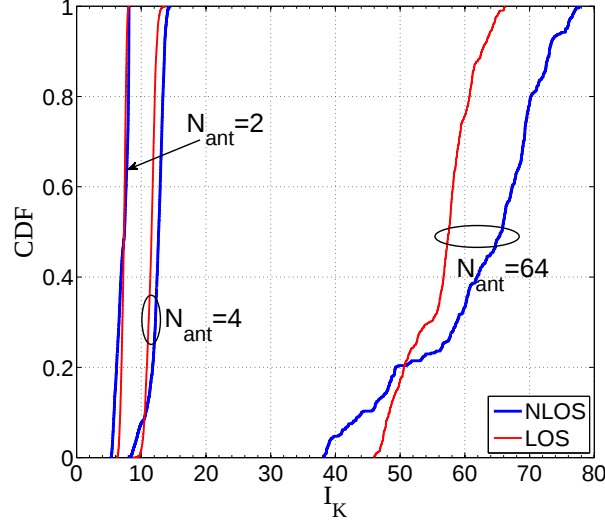
Figure 6-18: I_K vs. N_{ant} from space variability.
