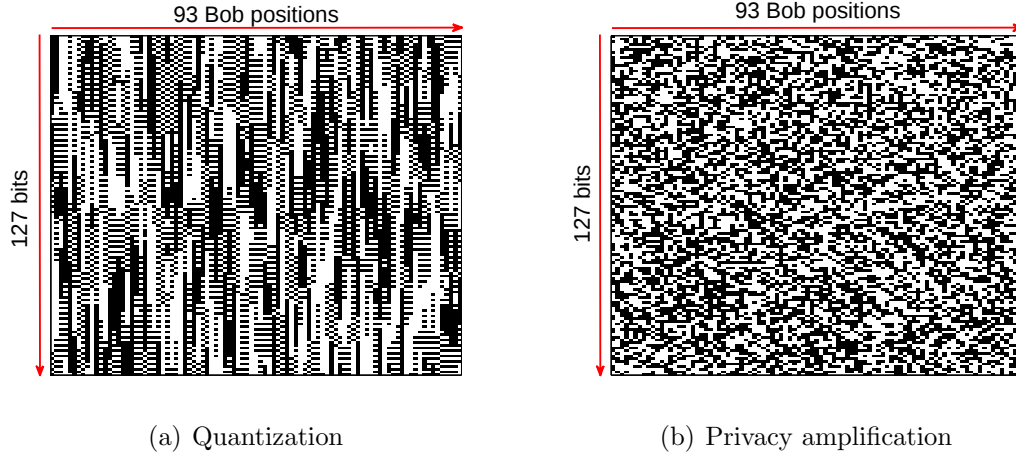
Figure 7-6: Keys from frequency DoFs, for different Bob positions and for SKSM.
