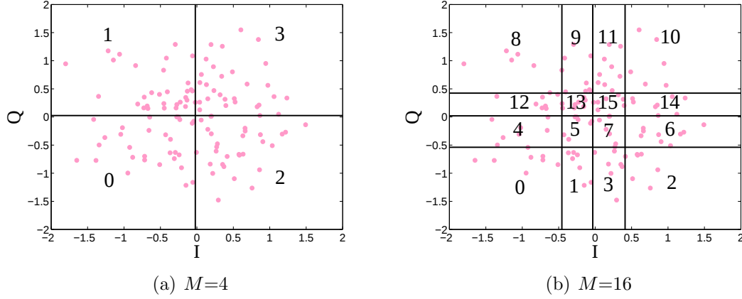
Figure 3-6: Correspondence between symbols and QR.
