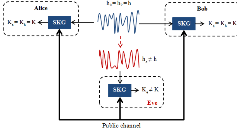
Figure 2-7: SKG in the presence of an eavesdropper.
