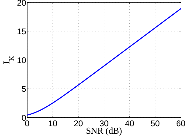
Figure 3-2: The impact of the SNR on I_K .
