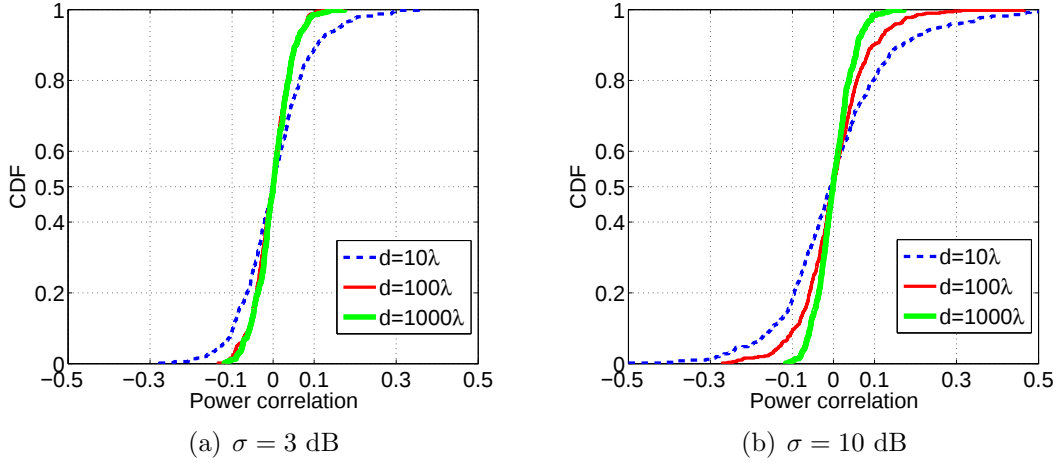
Figure 4-5: CDFs of the power envelope correlations.
