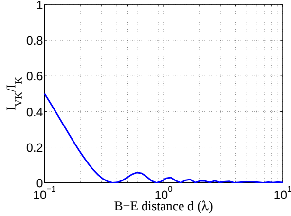
Figure 3-4: I_{VK}/I_K as a function of the separation distance d for Clarke's model.
