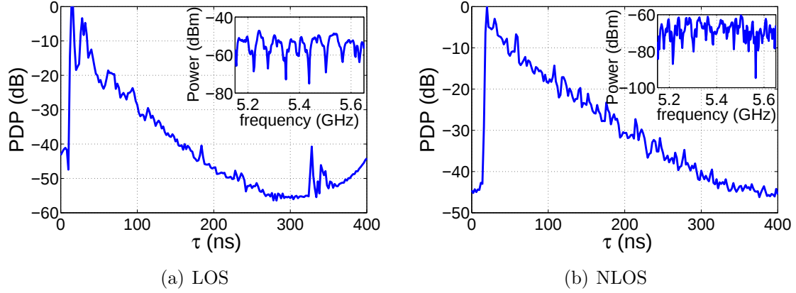
Figure 6-11: Examples of PDPs and channel transfer functions.
