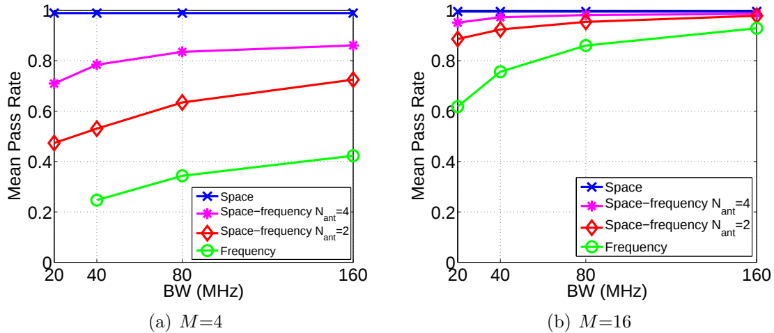
Figure 6-16: Comparison of key randomness in different channel variability at 5.4 GHz.
