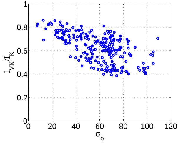
Figure 5-13: I_{VK}/I_K as a function of the angular spread, for N_f = 1 and d = 0.1\lambda .
