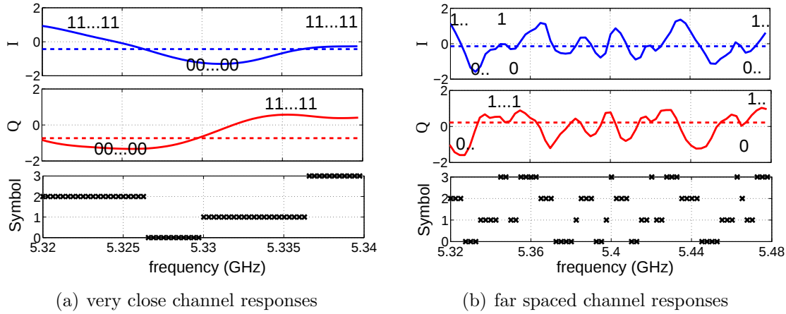
Figure 6-15: Example illustrating SKG from channel responses, for M=4 .
