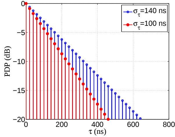
Figure 3-7: Some examples of PDP with different RMS delay spreads.
