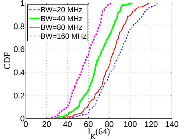
Figure 5-11: The impact of BW on I_K for N_f = 64 and for the scenario Louvre48.
