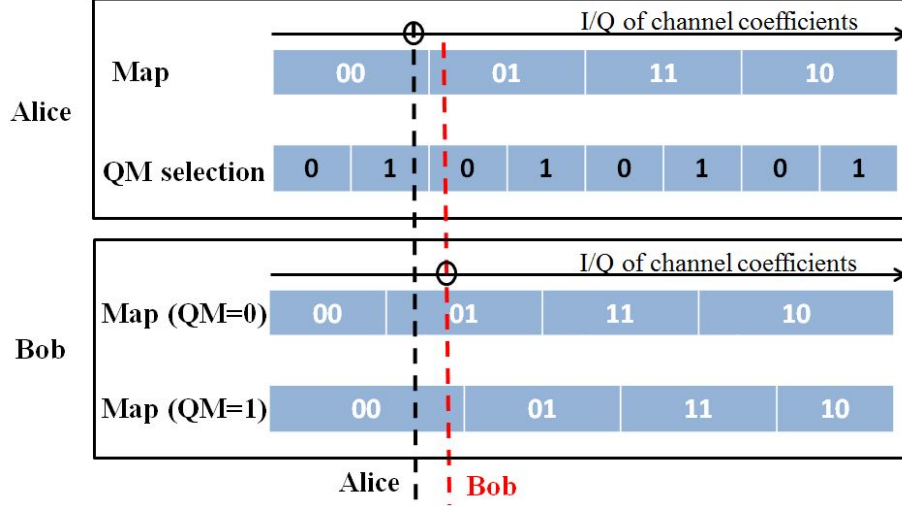
Figure 3-5: Illustration of the quantization intervals of the CQA scheme on one dimension I or Q with M = 16 .
