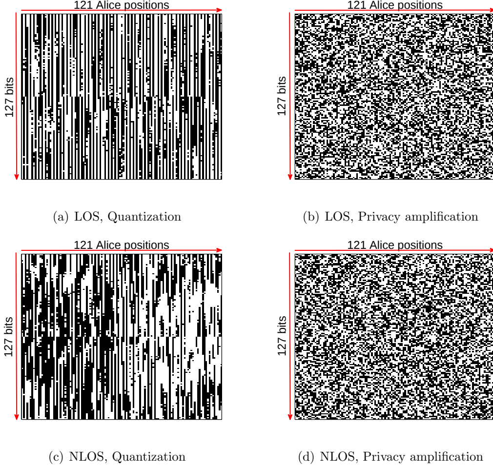
Figure 7-13: Keys from the frequency DoFs, over Alice positions and for MKSM.
