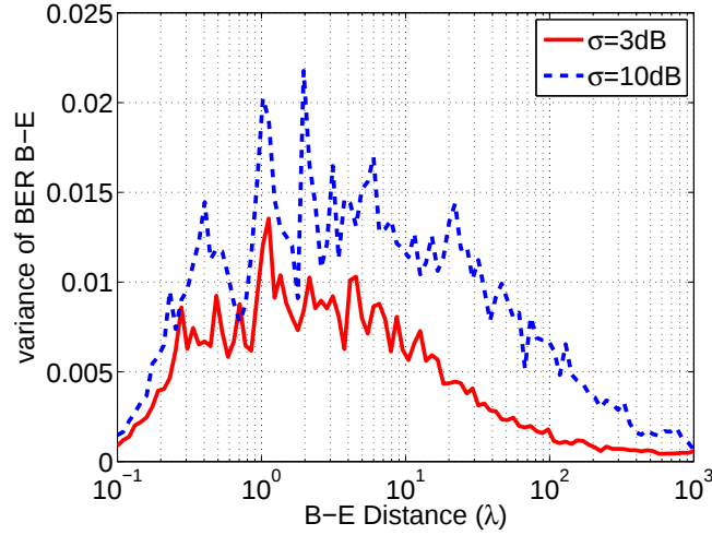
Figure 4-10: The statistical variance of BER as a function of d .
