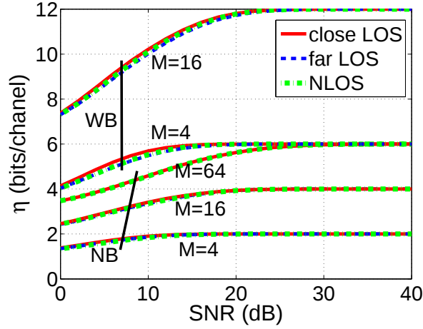
Figure 6-5: Secret key rate \eta for both NB and WB ( N_f = 3 ) channels.
