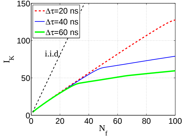
Figure 3-9: Evolution of I_K with respect to N_f and to the time resolution \Delta\tau , for \sigma_\tau = 100 ns.
