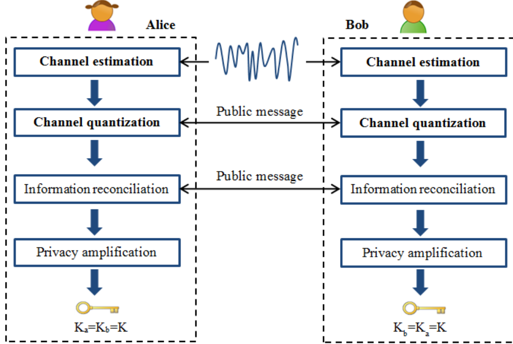
Figure 2-6: The four steps of SKG to agree on the same key.
