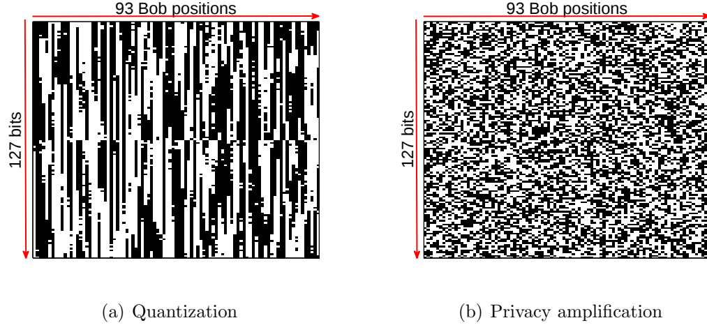
Figure 7-12: Keys from frequency DoFs, over Bob positions and for MKSM.
