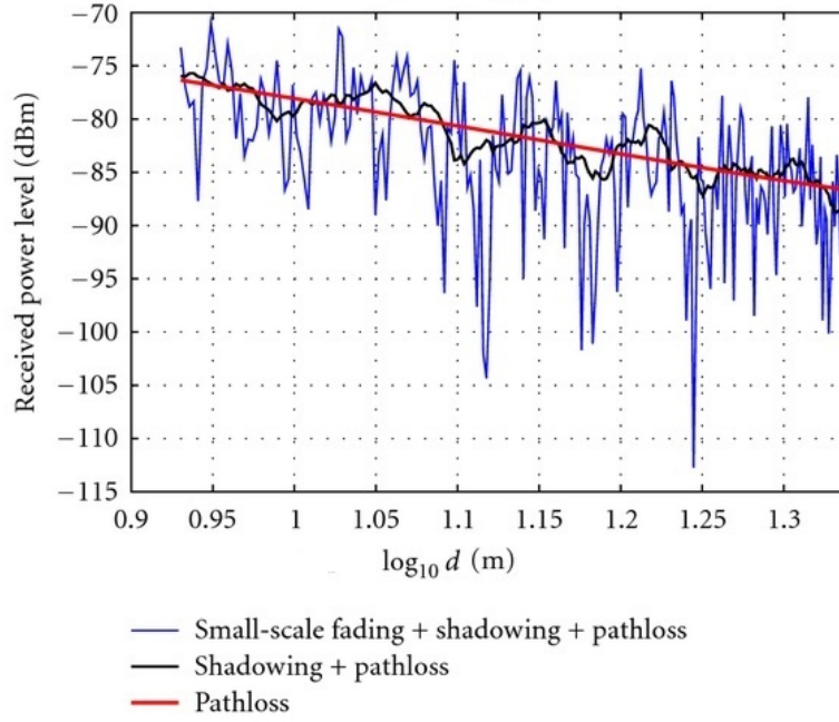
Figure 2-4: Path loss, shadowing and small scale fading.
