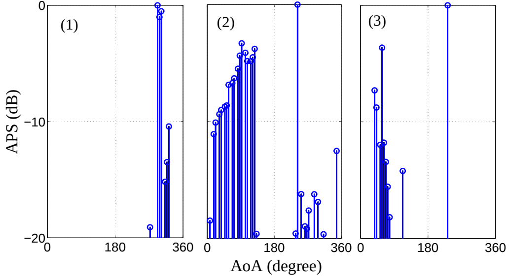
Figure 5-7: Some examples of APS corresponding to Louvre48 (right: \sigma_\phi = 5.3 degree, middle: \sigma_\phi = 71.3 degree, left: \sigma_\phi = 115 degree).
