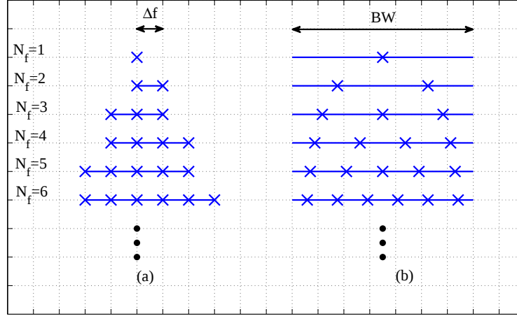
Figure 3-8: Frequency variability schemes with an increasing number of sub-carriers N_f : (a) an increasing BW and a fixed \Delta f , (b) a fixed BW and a decreasing \Delta f .
