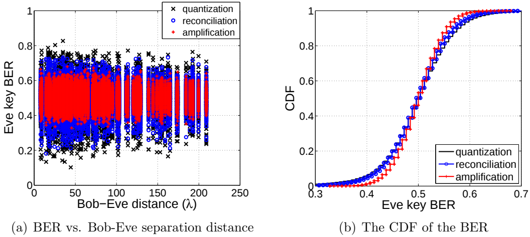
Figure 7-2: Disagreement between Bob and Eve keys for SKSM.
