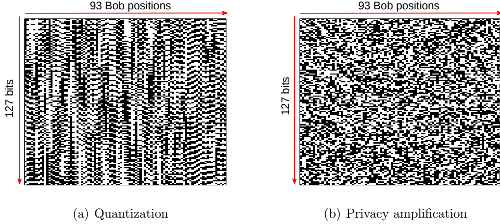
Figure 7-7: Keys from joint space-frequency DoFs ( N_{ant} = 2 ), for different Bob positions and for SKSM.
