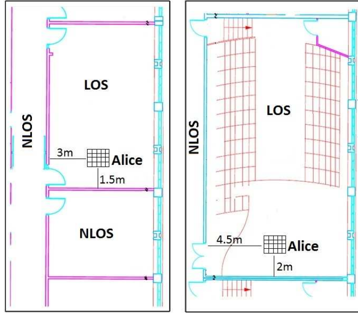
Figure 6-1: TPT measurement floor plans: (left) classrooms and (right) auditorium.
