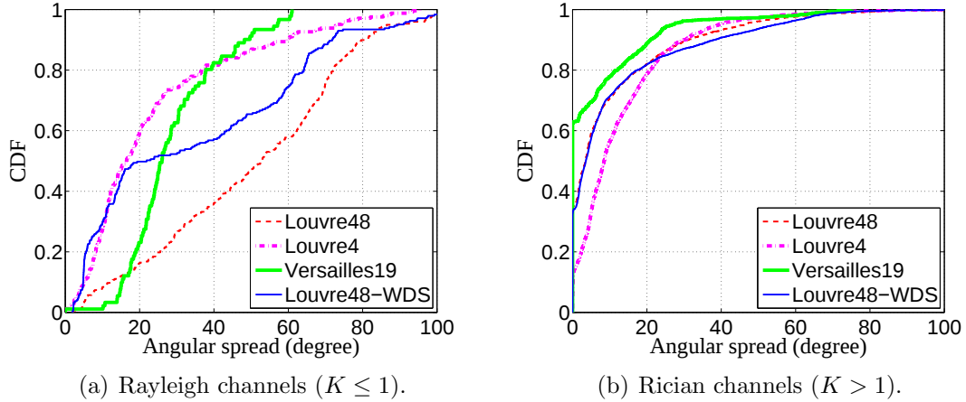
Figure 5-6: Angular spread statistics.
