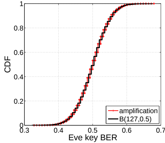
Figure 7-3: Eve key BER after privacy amplification vs. the BER for keys following B(127,0.5) .
