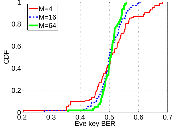
Figure 6-8: BER of Eve key bits from h_{ea} , for LOS B-E and for NB channels.
