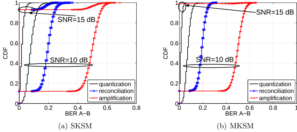
Figure 7-1: Disagreement between Alice and Bob keys.
