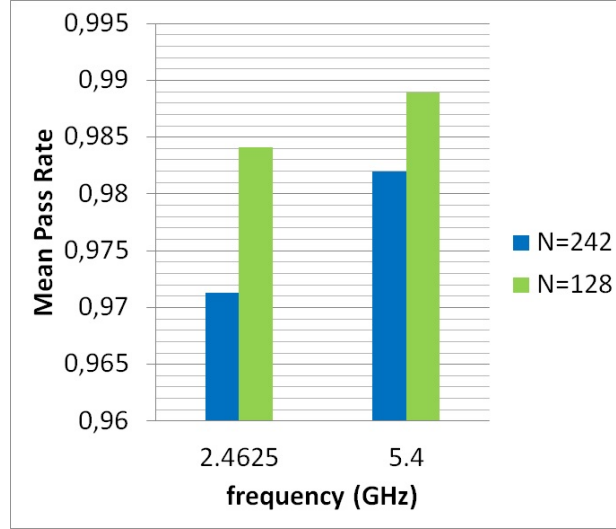
Figure 6-9: Mean pass rate exploiting spatial variability for both N = 128 and N = 242 .
