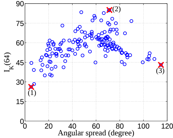
Figure 5-14: Space variability: I_K as a function of the angular spread.
