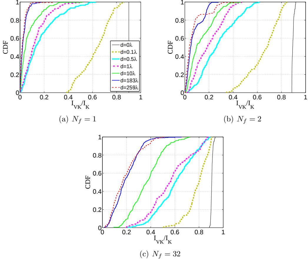
Figure 5-12: CDF of I_{VK}/I_K depending on N_f and on Bob/Eve distance (Louvre48).
