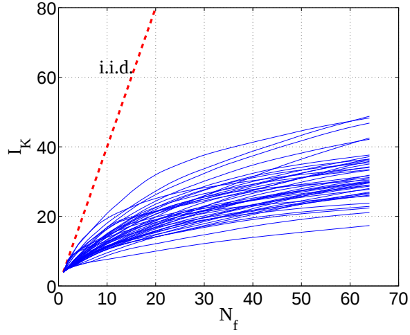
Figure 5-10: I_K as a function of N_f for the scenario Louvre48-WDS.
