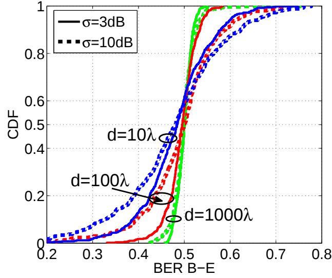
Figure 4-9: CDF of BER between Bob and Eve.
