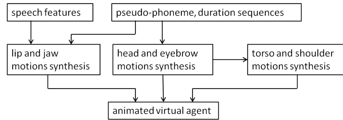
Figure 4.1: Overall architecture of multimodal behavior synthesis.
