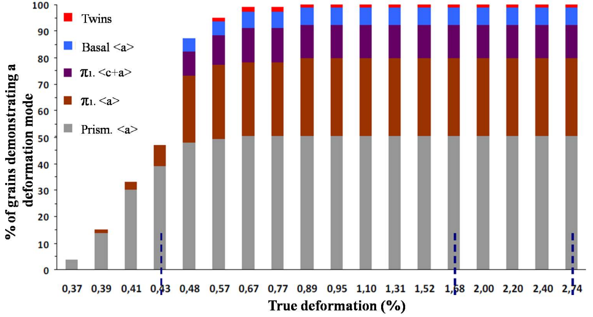
Figure 1.4: Frequency of slip modes under a transverse tensile for a T60 sample. Barkia's PhD thesis 2014 [11].
