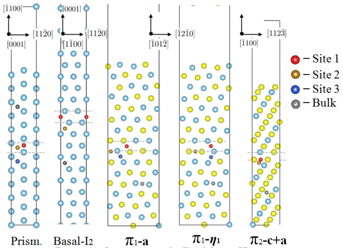
Figure 2.12: Segregation sites for H and O near SFs
