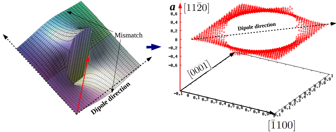
Figure 2.8: \langle a \rangle screw dislocation core dipole model. Continuous model and atomic model.
