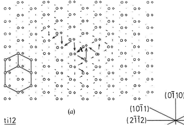
Figure 4.11: \langle \mathbf{c} + \mathbf{a} \rangle screw dislocation core dissociation in \pi_1 , \pi_2 and prismatic planes obtained using a ti12 potential with a dislocation line position at A [52].
