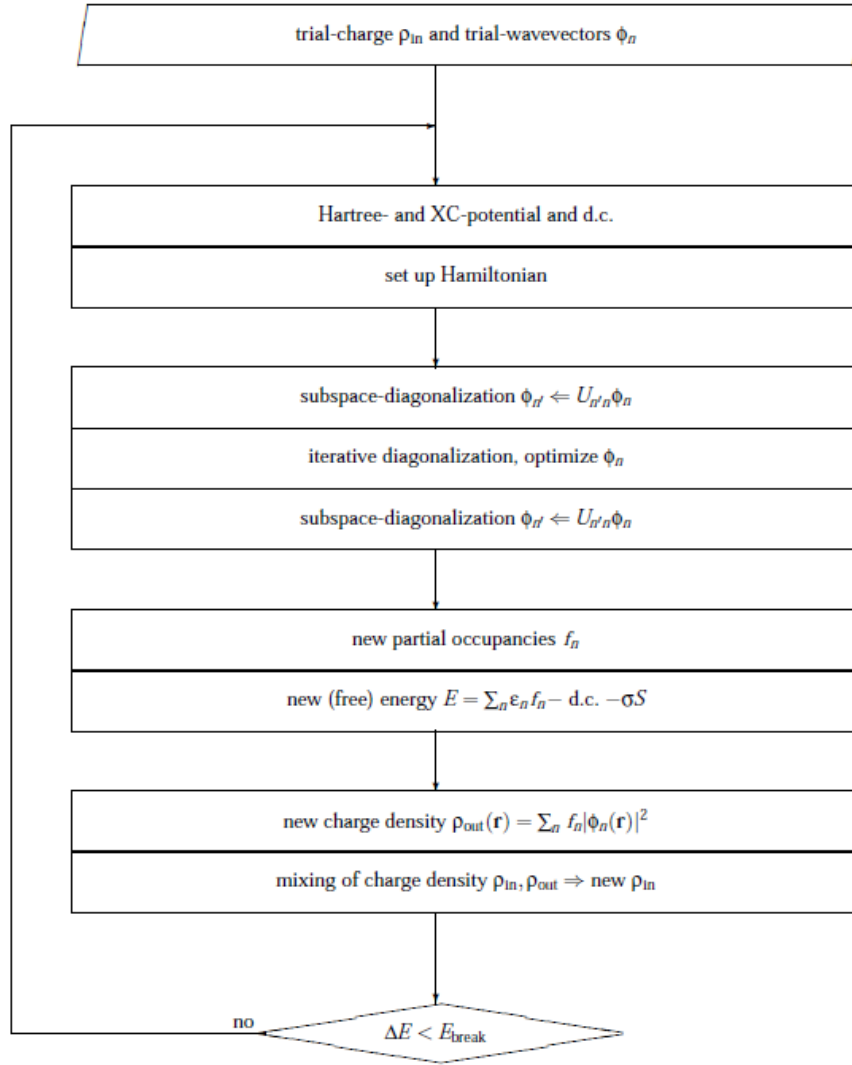
Figure 2.3: Procedures of a self-consistent calculation to obtain the KS ground state in VASP [145]
