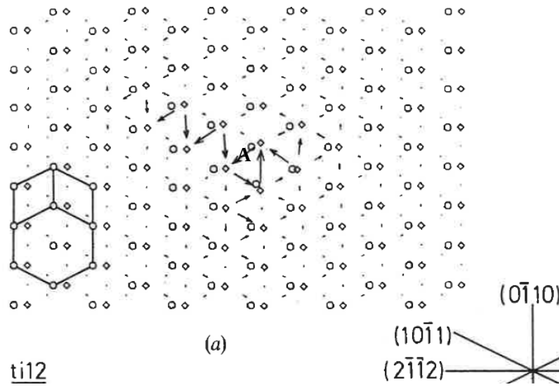
Figure 1.12: \langle \mathbf{c} + \mathbf{a} \rangle screw dislocation core dissociation in \pi_1 , \pi_2 and prismatic planes obtained using a ti12 potential with a dislocation line position at A [52].
