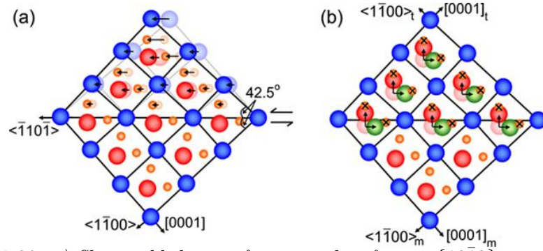
Figure 1.30: a) Shear added to perfect crystal to form a \{10\bar{1}2\} twin in \langle\bar{1}10\bar{1}\rangle direction; b) Arrows give the shuffles required to move the atoms in B-type sites (red) to either the B-(red) or C-type sites (green) in the twinned lattice. Reorientation of the lattice will eliminate the octahedral sites (marked with an X) where an oxygen atom could reside. [12].
