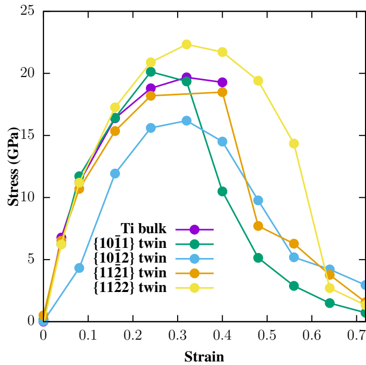
Figure 5.10: Twin boundary under deformations along perpendicular direction with Koyama method in pure Ti
