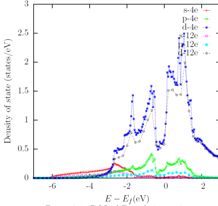
Figure 2.1: DOS of Ti with 4e or 12e
