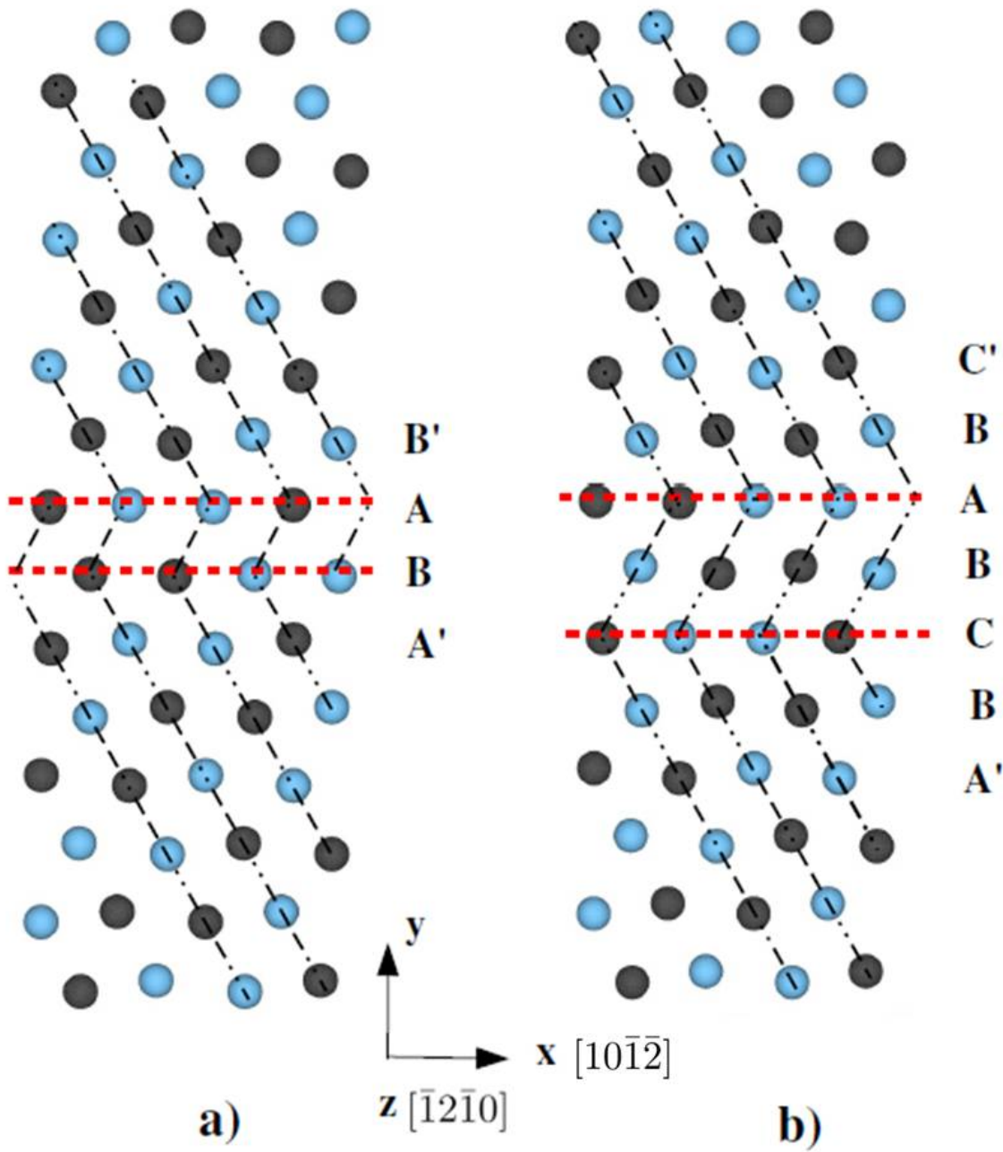
Figure 4.6: Two \{10\bar{1}1\} Twin-assisted SFs on \pi_1 . Left figure is related to the 0.215\langle 10\bar{1}2\rangle partial dislocation; right figure corresponds to the \frac{1}{2}\langle \mathbf{a} \rangle - \frac{1}{2}\langle \mathbf{b}_{TD} \rangle partial dislocation found in [44].
