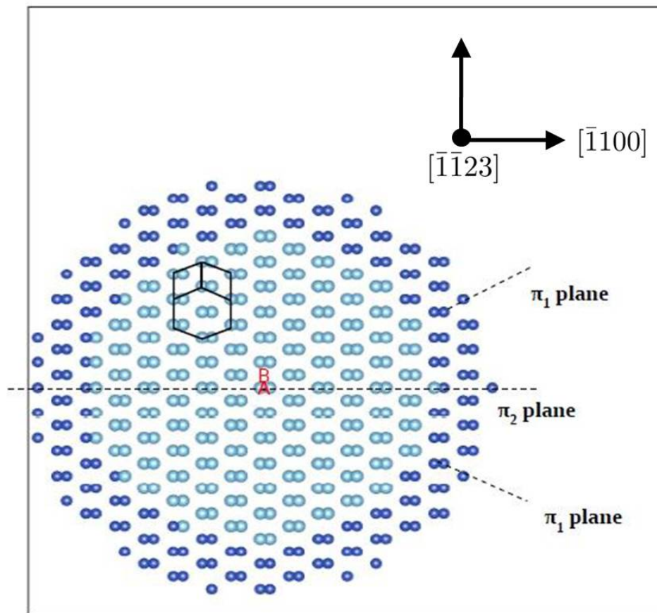
Figure 4.8: The \langle \mathbf{c} + \mathbf{a} \rangle screw dislocation visualized with two central core positions A and B for the application of u_z [eq. 2.22]. Direction perpendicular to \pi_2 plane is [11\bar{2}\frac{2}{\Lambda^2}] with \Lambda^2 = (2/3)(c/a)^2 . Cf. section 2.2.5.
