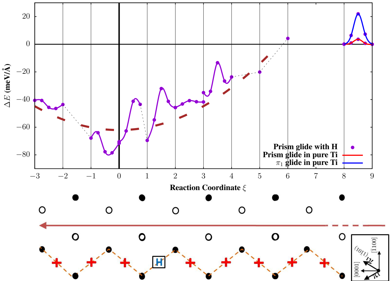
Figure 4.20: Up: MEP for a prismatic dislocation glide with H in dissociated plane; Down: Visualization of a prismatic dislocation glide with respect of a interstitial solute in an octahedral site. See text for critical comments.
