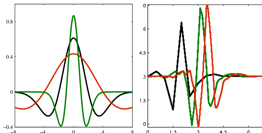
Figure 2.5: Ricker (left) and Symlet (right) wavelet with different a
