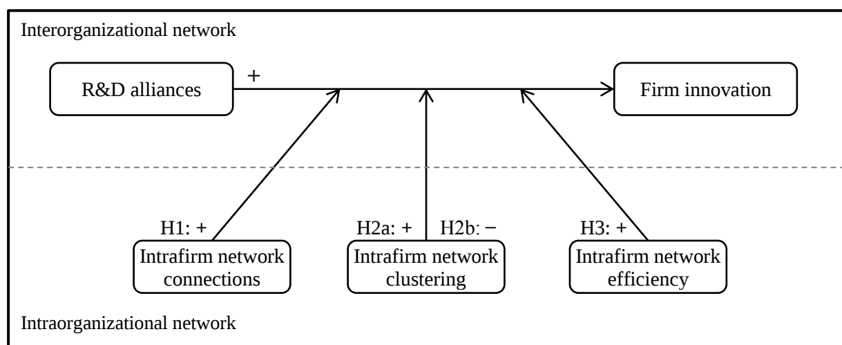
Figure 7 Theoretical framework
