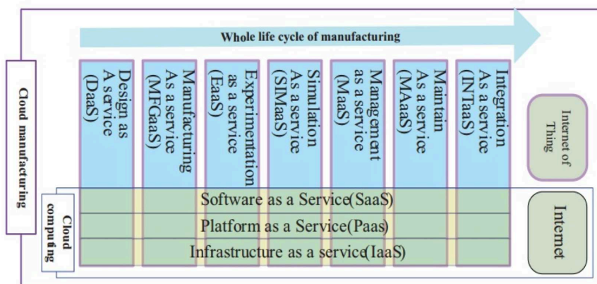
FIGURE 3.2 – Relation entre CC et CM [Tao 11]
