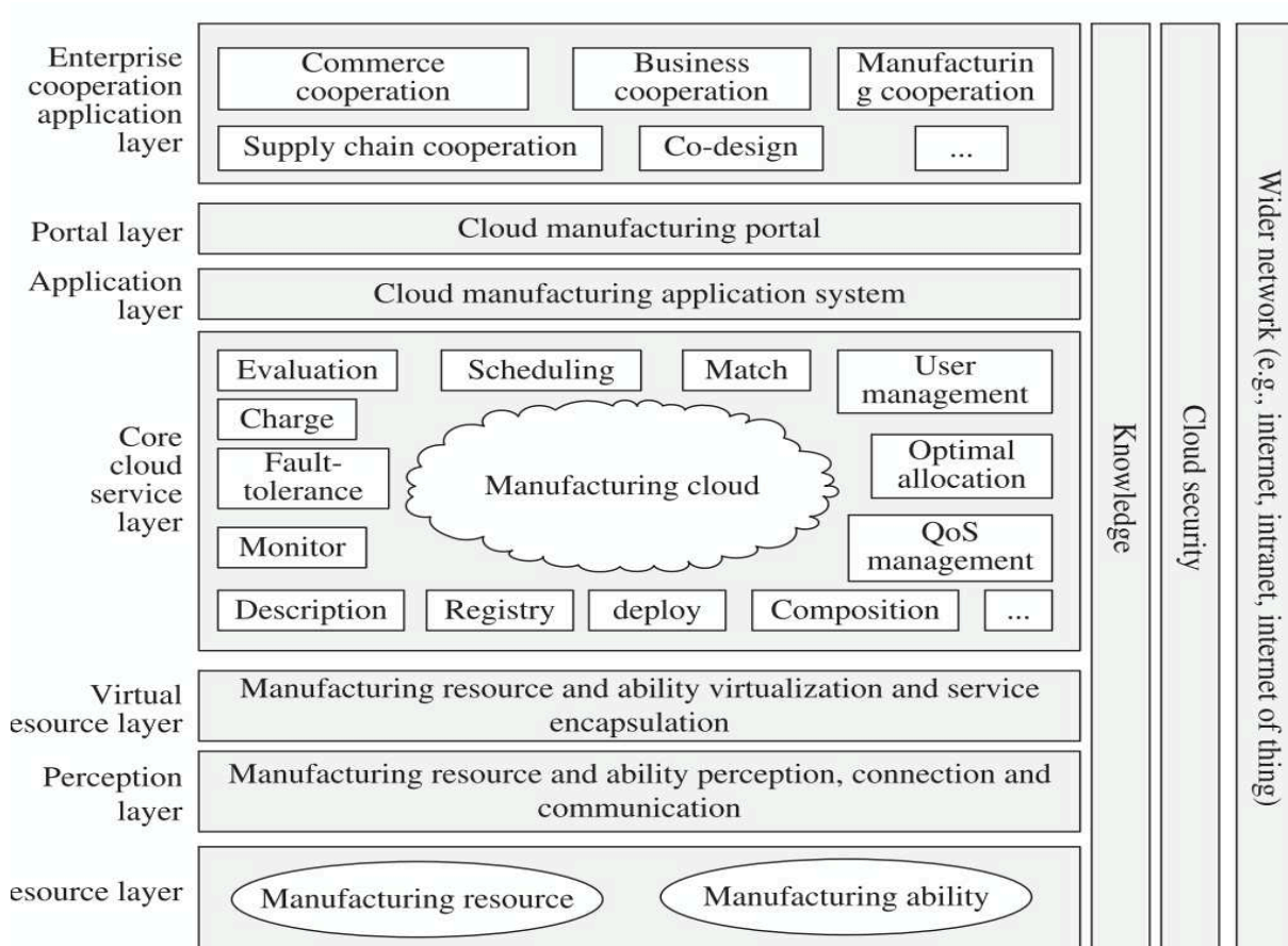
FIGURE 3.7 – L'architecture ManuCloud selon [Tao 11]
