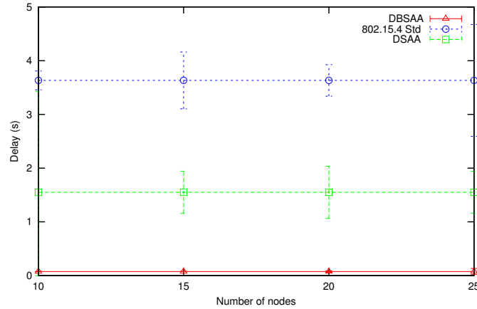
Figure 5.10: Delay DC=50% (BO=6,SO=2)
