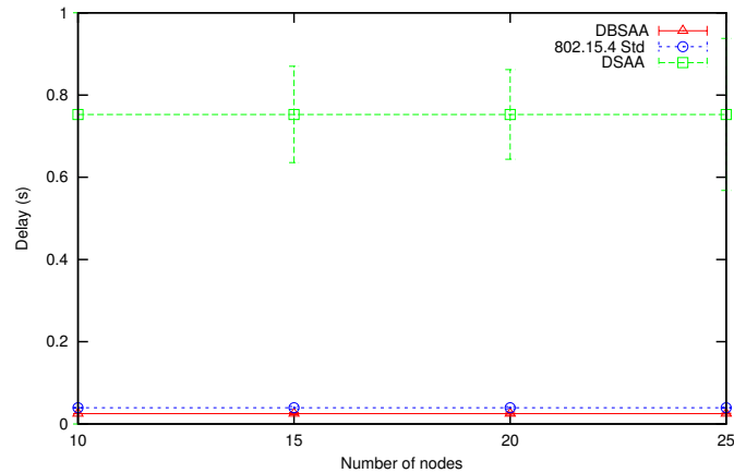
Figure 5.9: Delay DC=6% (BO=2,SO=1)]
