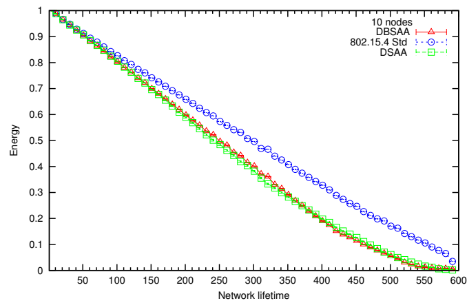
FIGURE 7 – Energy average consumption DC 50% (BO = 2, SO = 1) - 10 nodes
