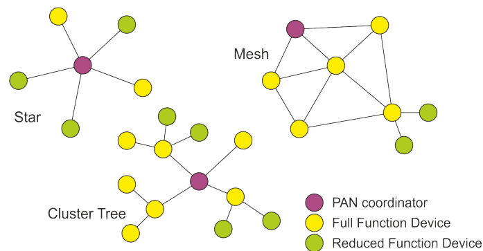
Figure 2.3: topology
