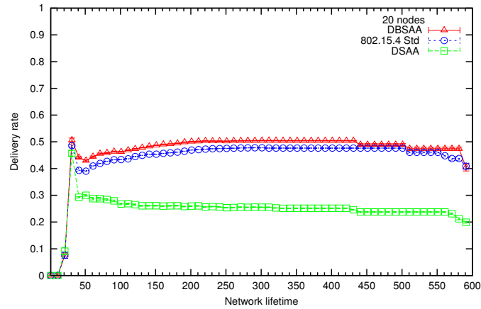
FIGURE 12 – Packet delivery ratio DC 50% (BO = 2, SO = 1) - 20 nodes
