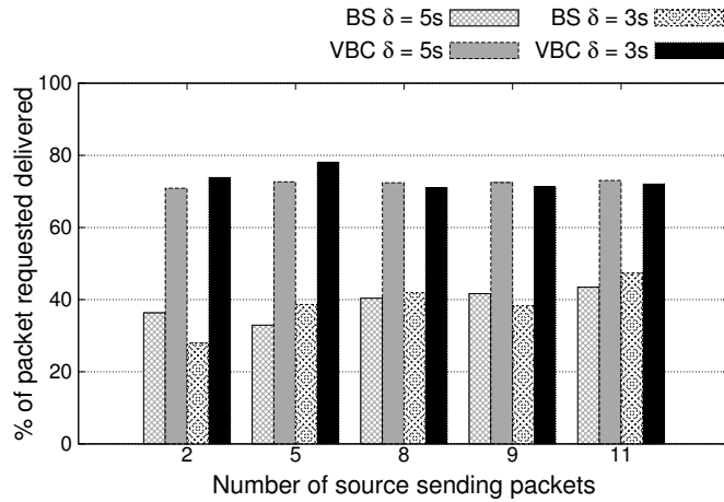
(b) Packet delivery ratio (FPVB)
