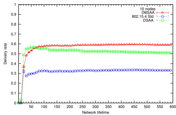
Figure 5.3: Packet delivery ratio DC 6% (BO = 6, SO = 2) 10 nodes
