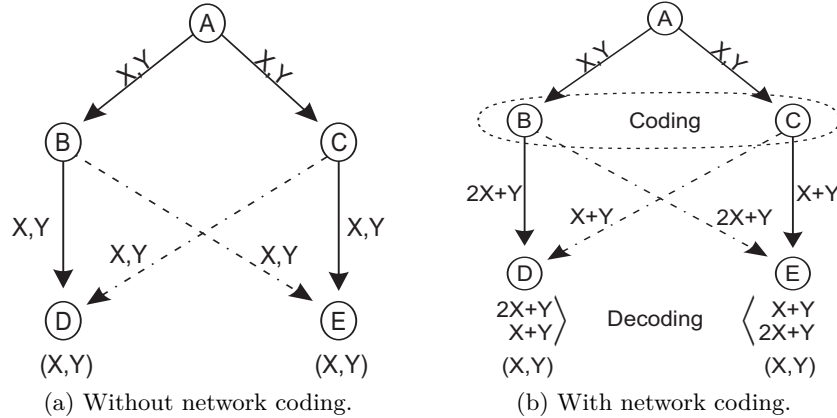
Figure 2.7: Example of Network Coding Operation.
