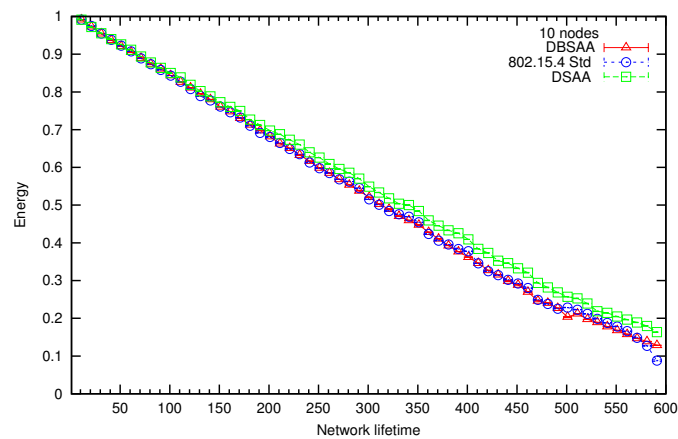
FIGURE 9 – Energy average consumption DC 6% (BO = 6, SO = 2) - 10 nodes
