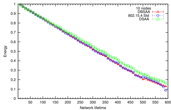
Figure 5.7: Energy average consumption DC 6% (BO = 6, SO = 2) 10 nodes
