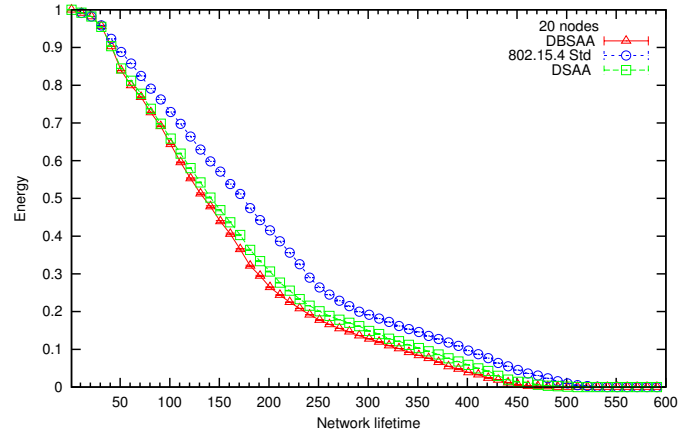
Figure 5.8: Energy average consumption DC 6% (BO = 6, SO = 2) 20 nodes
