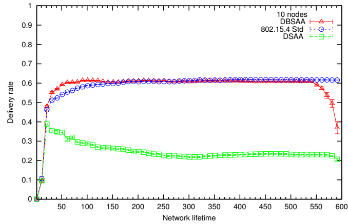
FIGURE 11 – Packet delivery ratio DC 50% (BO = 2, SO = 1) - 10 nodes
