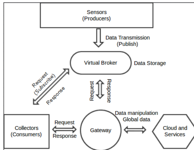
Figure 4.2: System model: iteration among entities
