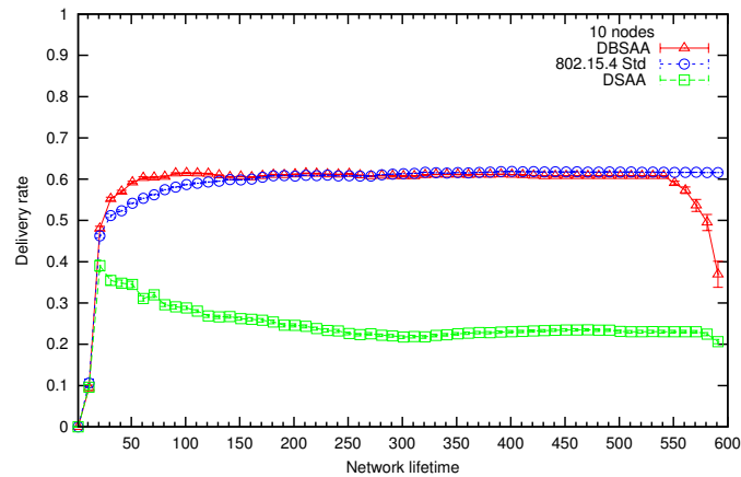
Figure 5.1: Packet delivery ratio DC 50% ( BO = 2 , SO = 1 ) 10 nodes
