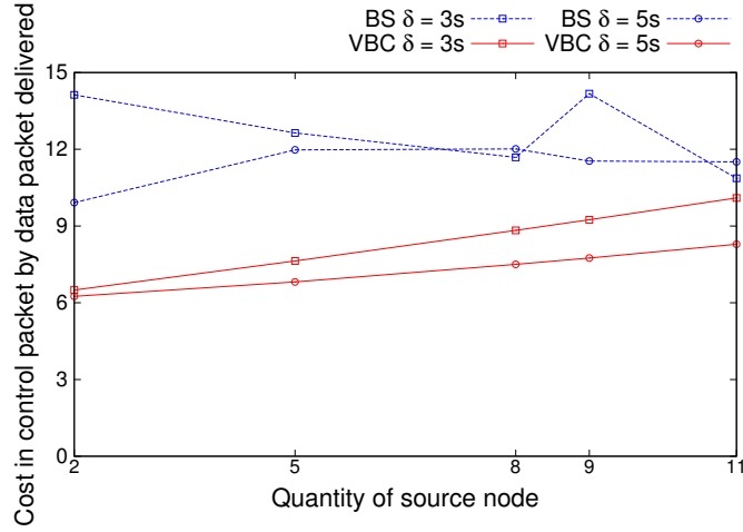
(a) Cost-benefit (EPCC)
