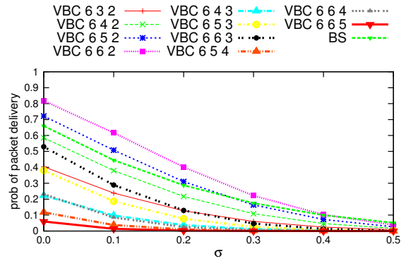
Figure 5.16: Packet delivery with \gamma = 0.33
