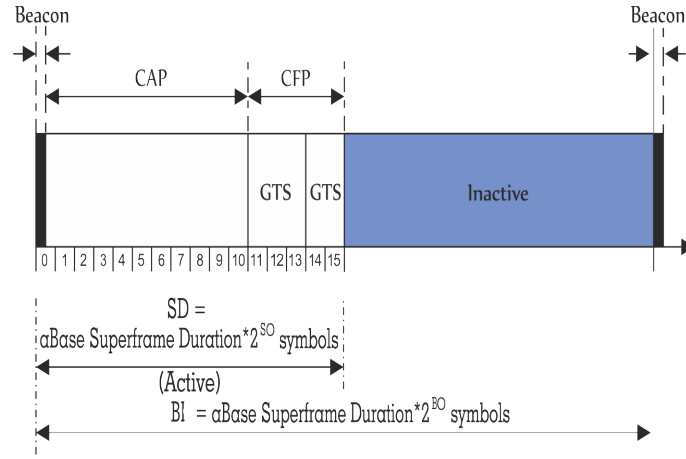
Figure 2.4: Super frame structure.
