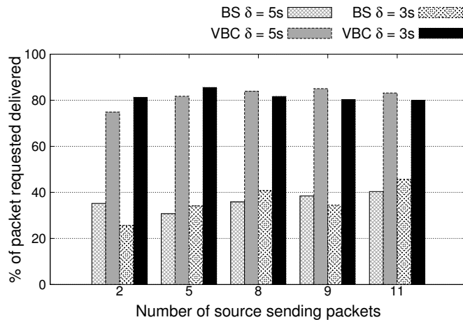
(a) Packet delivery ratio (EPCC)
