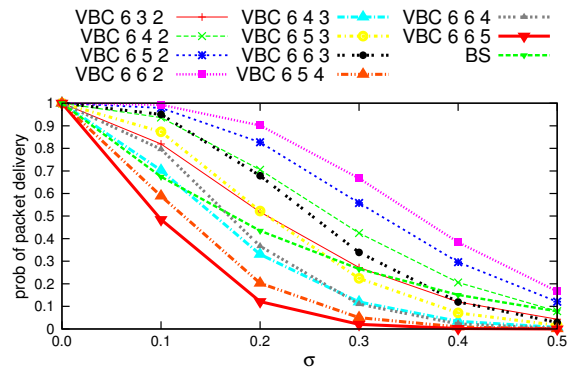
Figure 5.12: Packet delivery without DC
