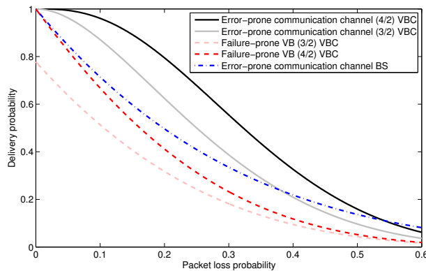
Figure 3.3: Packet delivery probability.
