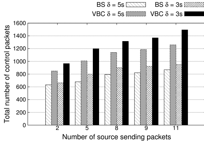
(b) Communication Cost (FPVB)
