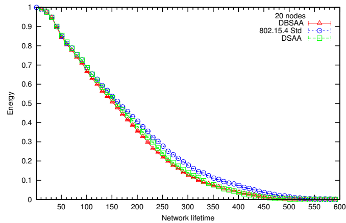
Figure 5.6: Energy average consumption DC 50% (BO = 2, SO = 1). 20 nodes
