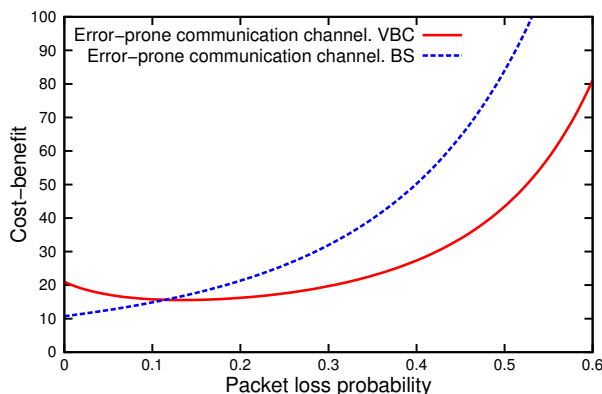
Figure 3.4: Cost per packet delivered.
