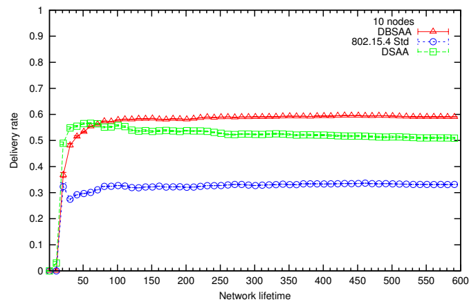
FIGURE 13 – Packet delivery ratio DC 6% (BO = 6, SO = 2) - 10 nodes
