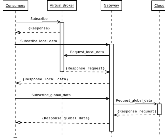
Figure 4.4: Sequence diagram of the subscribe operation
