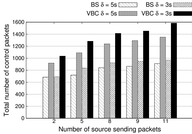
(a) Communication Cost (EPCC)
