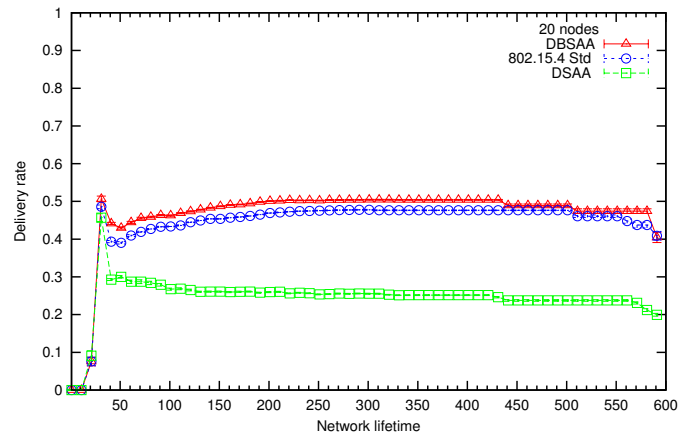
Figure 5.2: Packet delivery ratio DC 50% (BO = 2, SO = 1) 20 nodes
