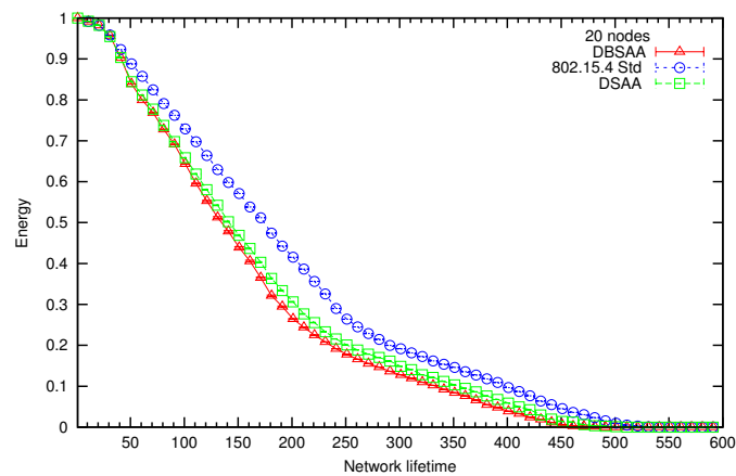
FIGURE 10 – Energy average consumption DC 6% (BO = 6, SO = 2) - 20 nodes
