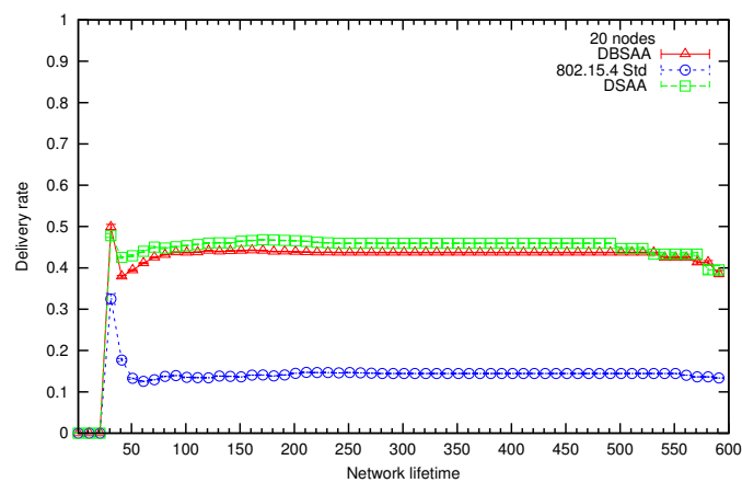
Figure 5.4: Packet delivery ratio DC 6% (BO = 6, SO = 2) 20 nodes
