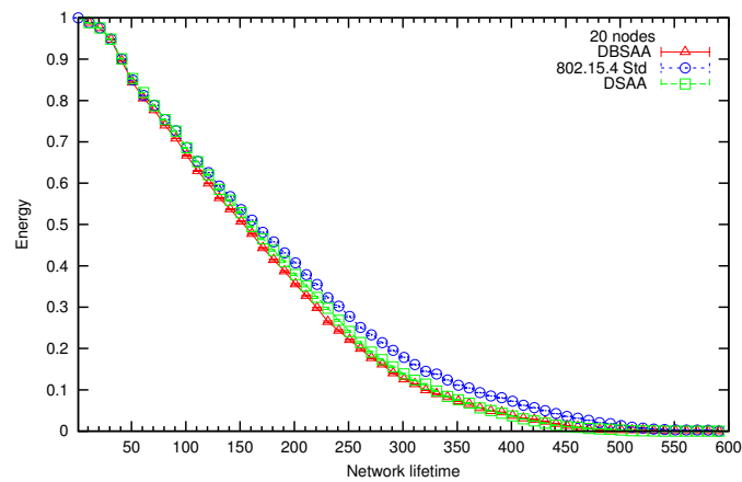
FIGURE 8 – Energy average consumption DC 50% (BO = 2, SO = 1)- 20 nodes
