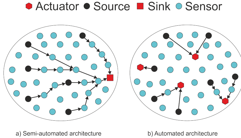
Figure 2.5: WSNs architectures.
