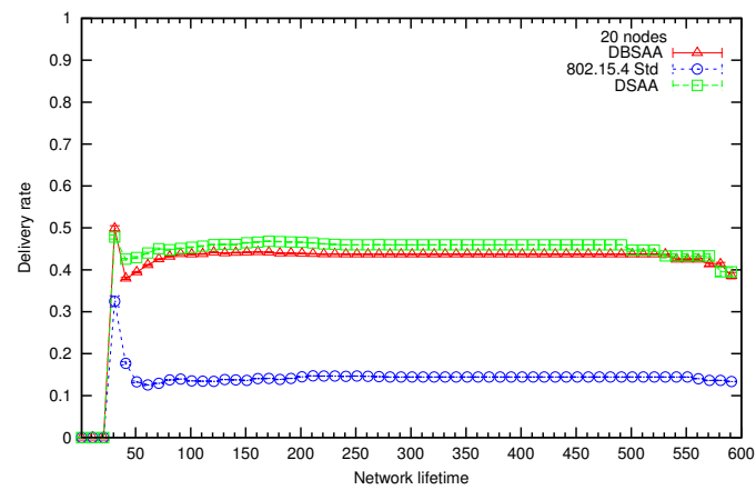
FIGURE 14 – Packet delivery ratio DC 6% (BO = 6, SO = 2) 20 - nodes
