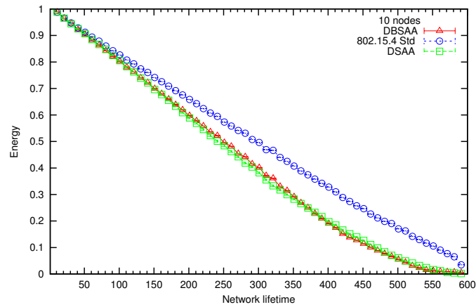
Figure 5.5: Energy average consumption DC 50% (BO = 2, SO = 1). 10 nodes
