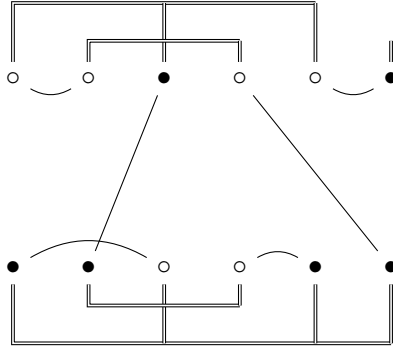
Figure 5.2: Two-colored bidiagram
