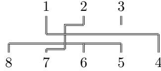
Figure 1.5: Two-level partition in P(3, 5) with block structure \{\{5, 6, 8\}, \{2, 7\}, \{1, 4\}, \{3\}\}
