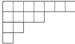
Figure 2.1: Young diagram of (7, 4, 2, 1) .
