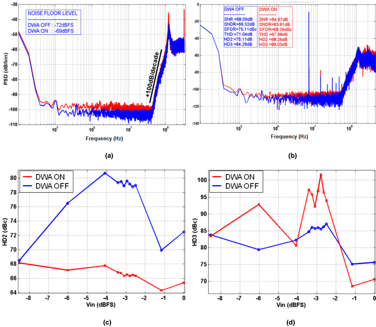
Figure 5-3. (a) PSD of the modulator output without input signal, (b) PSD of the modulator output with a 6MHz input sine tone of -4\text{dBFS} , (c) Measured second-order harmonic distortion as a function of the input signal amplitude with and without DWA (d) measured third-order harmonic distortion as a function of the input signal amplitude with and without DWA.
