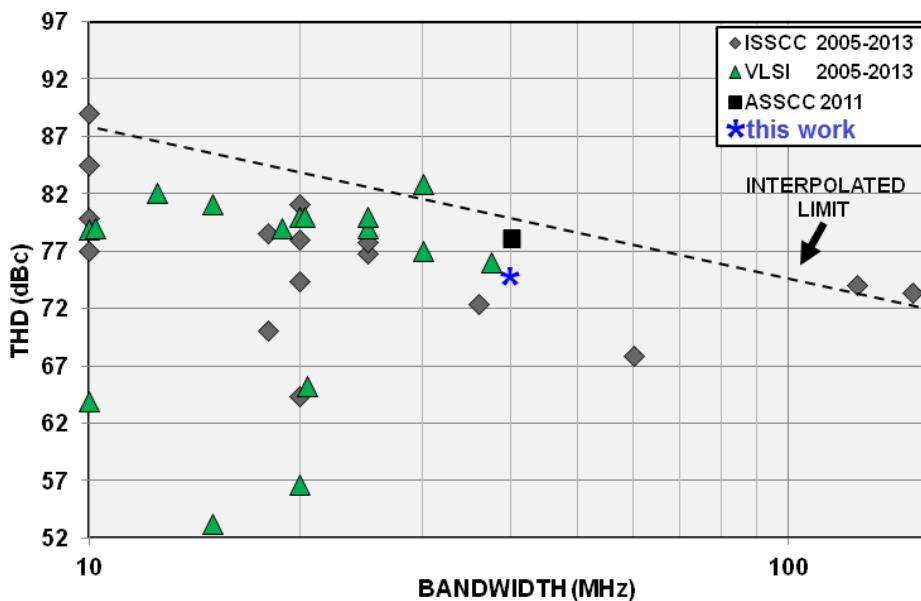
Figure 6-5. State-of-the-art THD as a function of the signal bandwidth of wideband low-pass CMOS \Delta\Sigma modulators.
