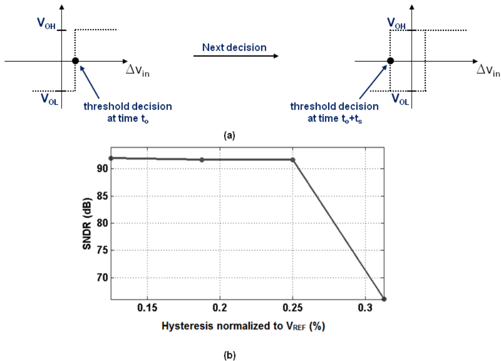
Figure 3-31. (a) Illustration of the hysteresis effect, (b) simulation of the impact of comparator hysteresis ( V_{in} = -1.1\text{dBFS} @ f_{in} = 10\text{MHz} ).
