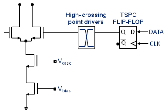
Figure 4-11. Unit current cell used in minors DACs (DAC2 & DAC3).
