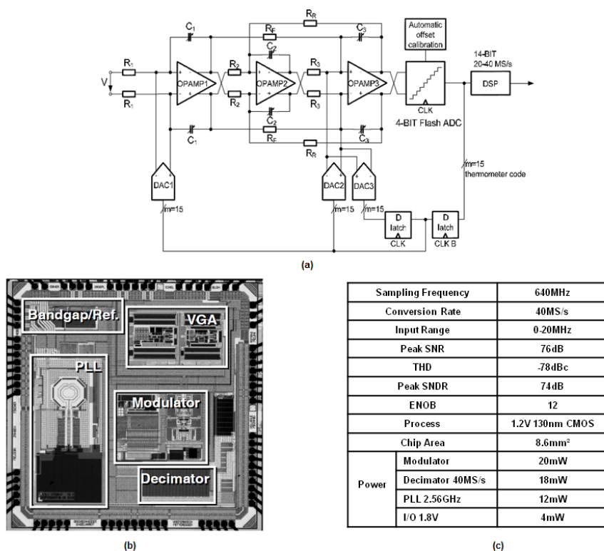
Figure 2-1. Characteristics of the \Delta\Sigma ADC IC introduced by Xignal Technologies in 2006 [3]. (a) CT \Delta\Sigma Modulator architecture, (b) Chip micrograph, (c) Performance summary.
