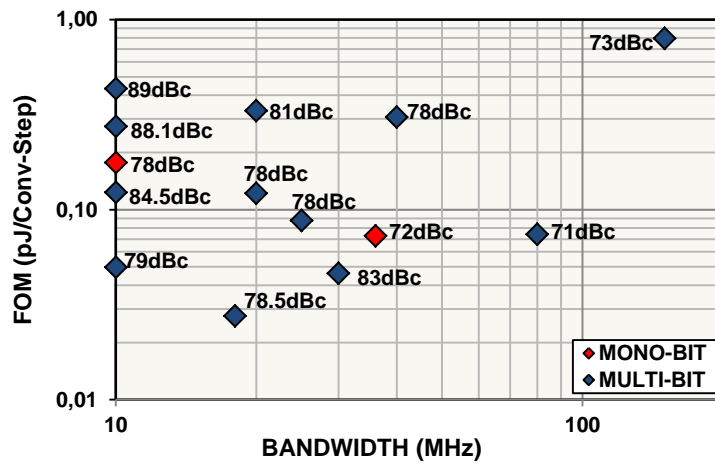
Figure 2-14. FoM repartition as a function of signal bandwidth for wideband mono-bit and multi-bit \Delta\Sigma modulator with ENOB \geq 11 -bit.
