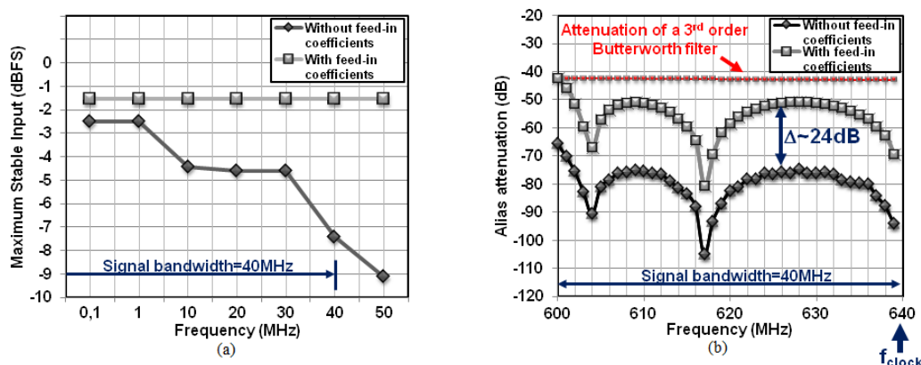
Figure 2-17. Feed-in coefficients effect on (a) the maximum stable input amplitude, (b) the inherent anti-alias filter transfer function.
