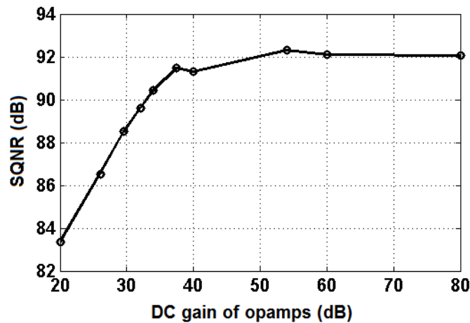
Figure 3-9. Influence of the finite gain of all opamps
